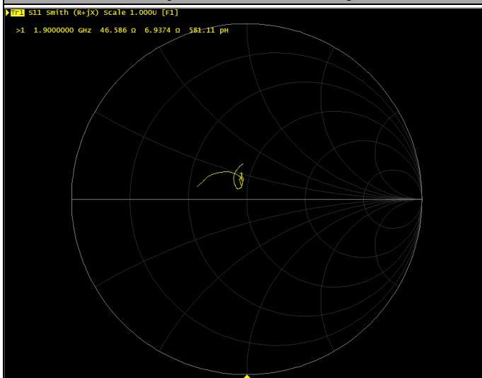
Impedance Test-Body
