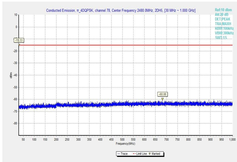
Fig. 34 Conducted Spurious Emission ( \pi/4 DQPSK, Ch78, 30 MHz-1 GHz)
