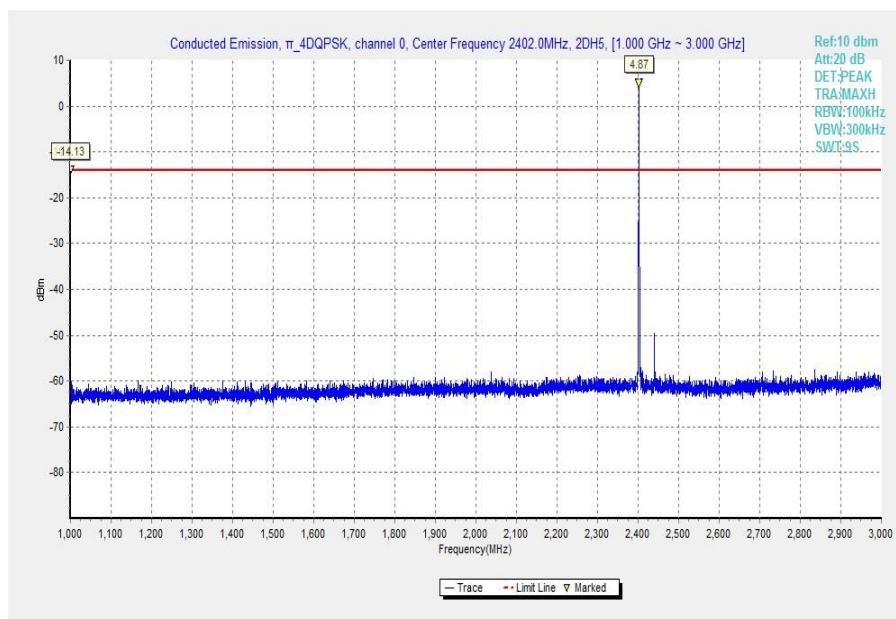
Fig. 27 Conducted Spurious Emission ( \pi /4 DQPSK, Ch0, 1GHz-3 GHz)
