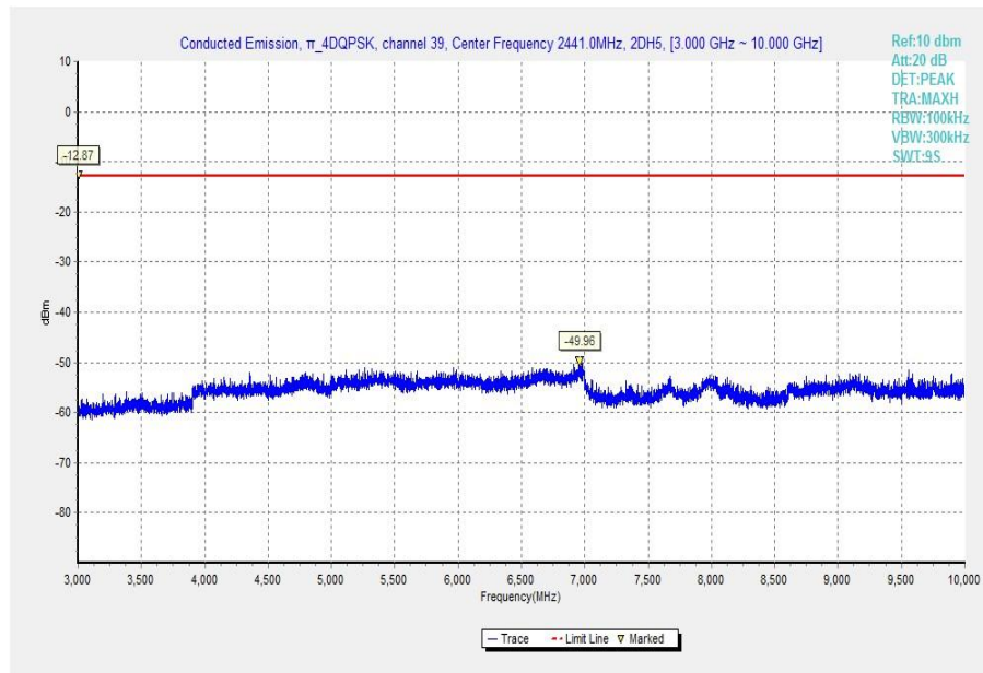
Fig. 32 Conducted Spurious Emission ( \pi/4 DQPSK, Ch39, 3GHz-10 GHz)
