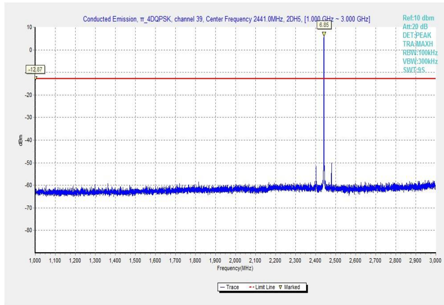
Fig. 31 Conducted Spurious Emission ( \pi/4 DQPSK, Ch39, 1 GHz-3 GHz)
