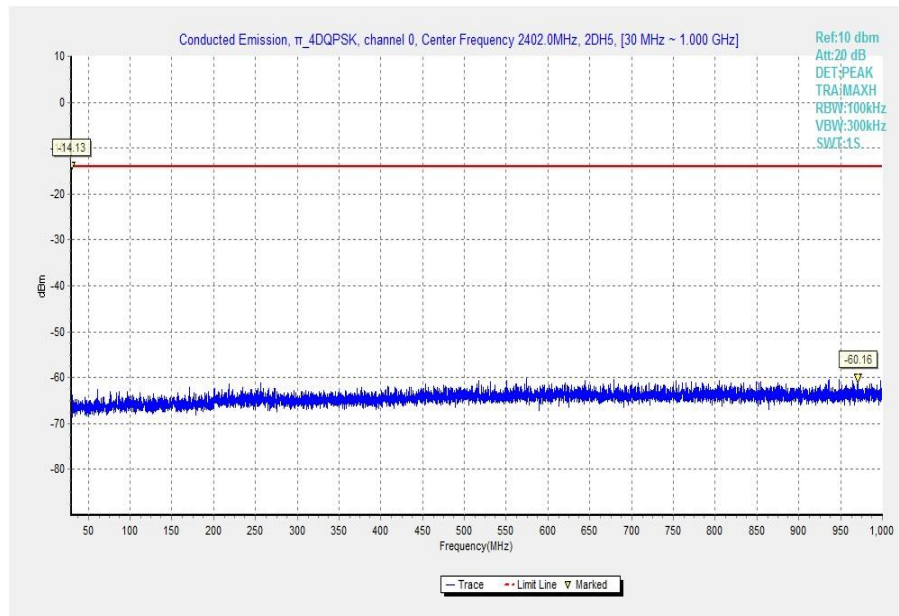
Fig. 26 Conducted Spurious Emission ( \pi/4 DQPSK, Ch0, 30 MHz-1 GHz)
