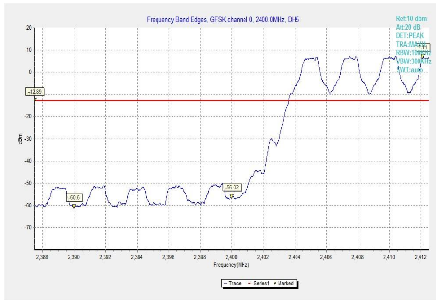
Fig. 1 Band Edges (GFSK, Ch 0, Hopping ON)
