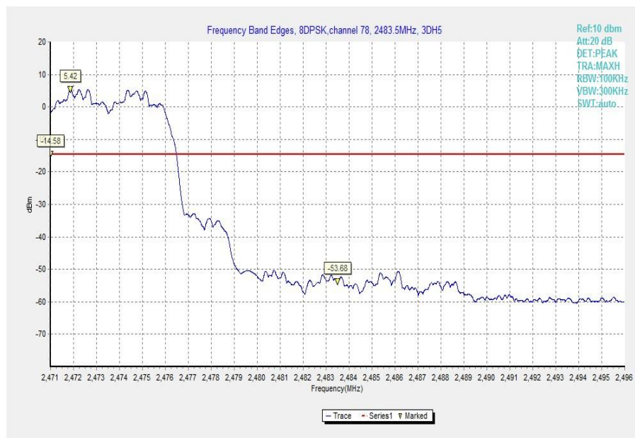
Fig. 6 Band Edges (8DPSK, Ch 78, Hopping ON)
