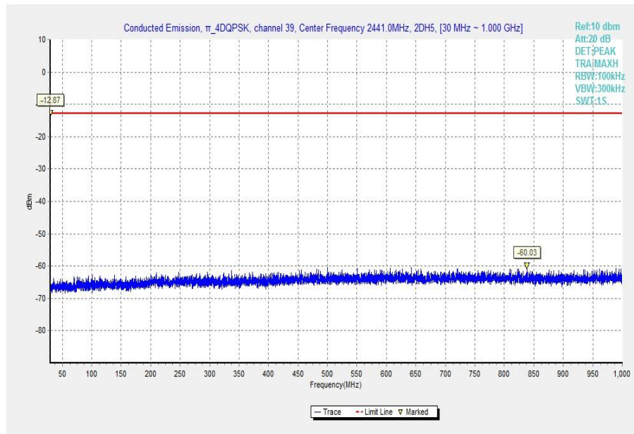
Fig. 30 Conducted Spurious Emission ( \pi/4 DQPSK, Ch39, 30 MHz-1 GHz)
