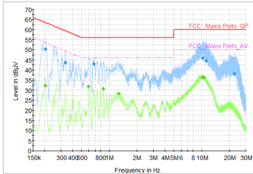
Fig. 107 AC Power line Conducted Emission (Idle, AE2, 240V)
