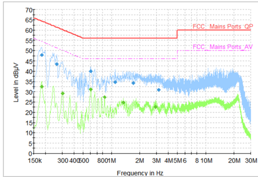
Fig. 104 AC Power line Conducted Emission (Traffic, AE1, 240V)
