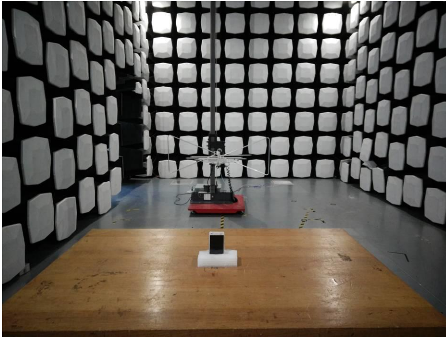
5. Radiated Emissions (Part 15C) 30M-1GHz)
