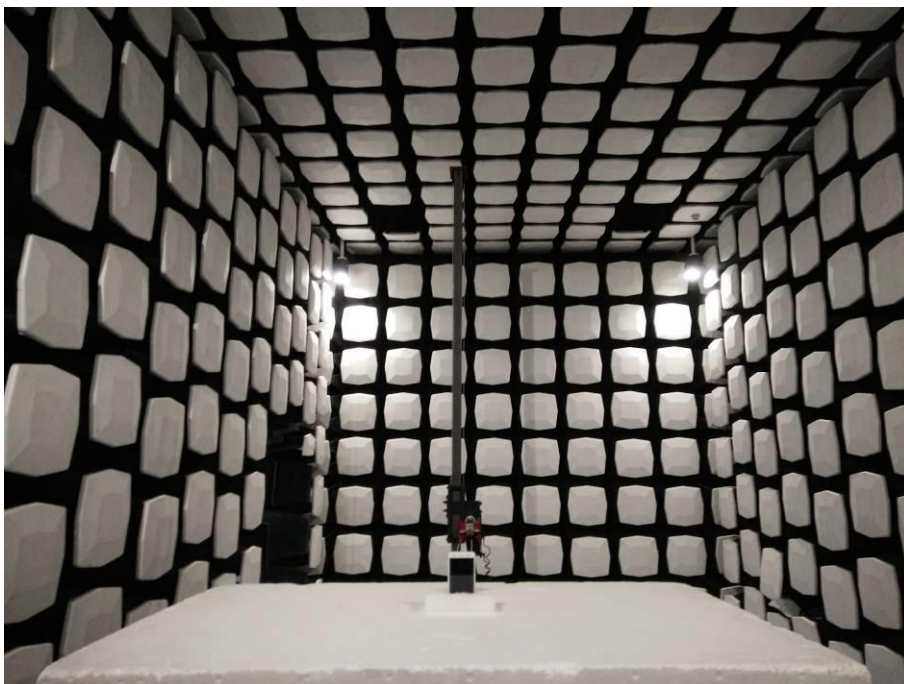
6. Radiated Emissions (Part 15C) (1-18GHz)
