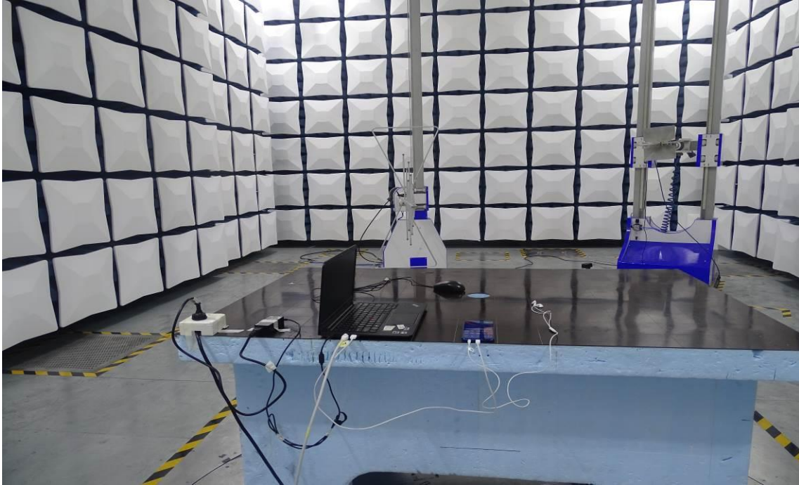
Radiated Disturbance Emissions (30MHz-1GHz)
