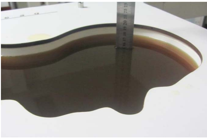
Photo 24:HBBL3500-5800MHz depth (15.2cm)
