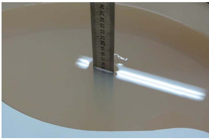
Photo 25:MBBL3500-5800MHz depth (15.1cm)
