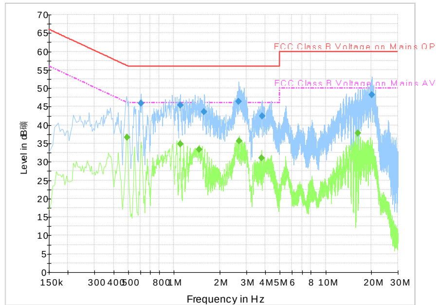
Fig. 78 AC Powerline Conducted Emission-802.11a
