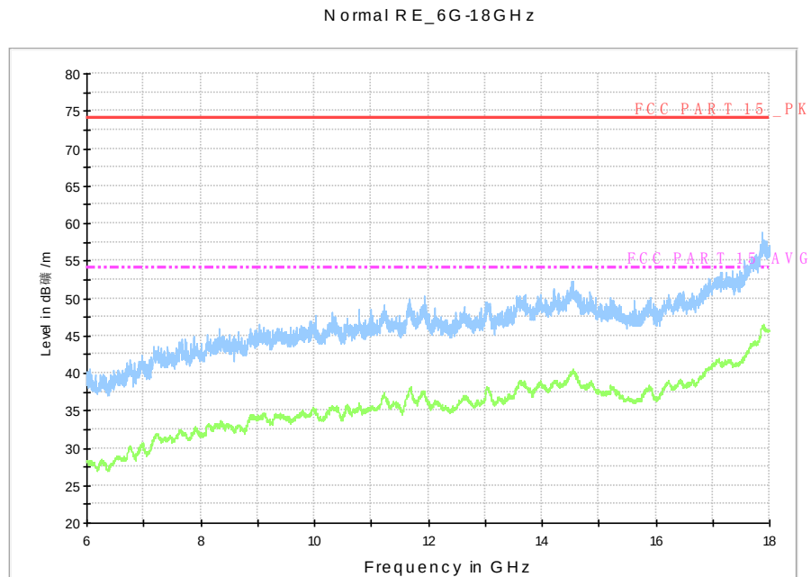
Fig. 45 Radiated Spurious Emission (802.11a, Ch157, 6 GHz-18 GHz)
