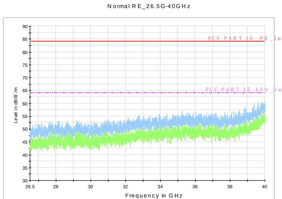
Fig. 63 Radiated emission: 802.11n, (802.11n-HT40, Ch151, 26.5 GHz - 40 GHz)
