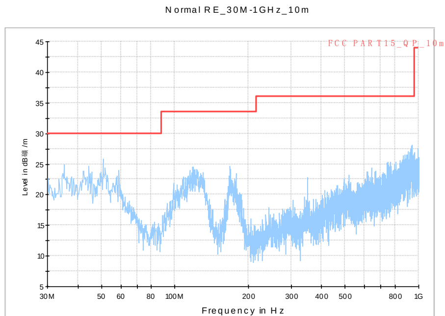
Fig. 59 Radiated Spurious Emission (802.11n-HT40, Ch151, 30 MHz-1 GHz)
