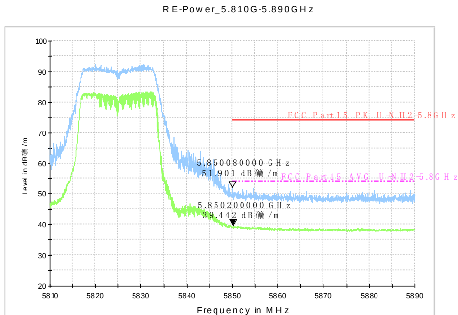
Fig. 73 Band Edges (802.11a, 5825MHz)
