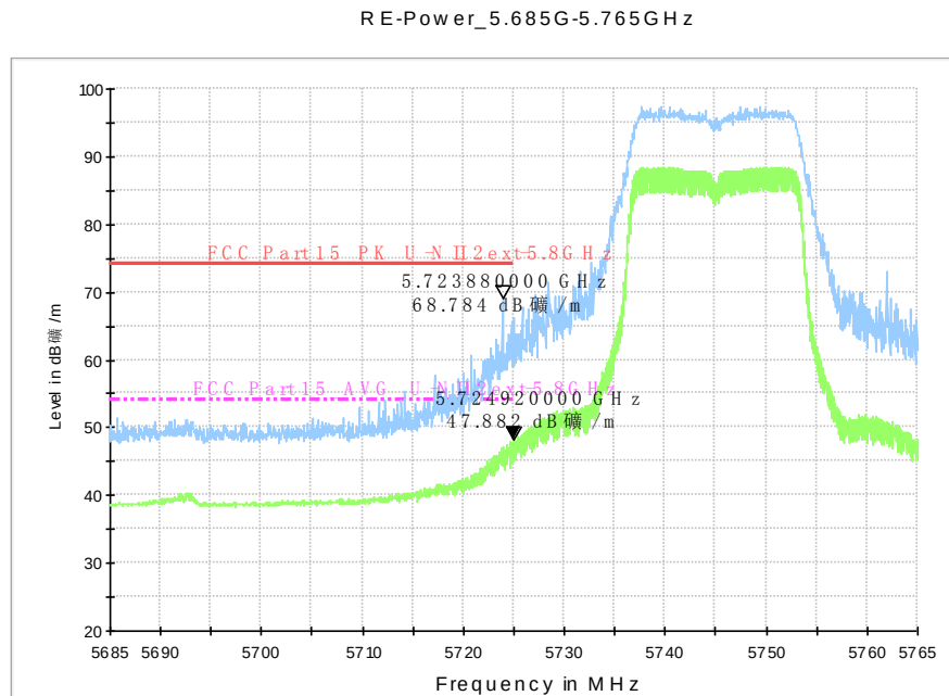
Fig. 72 Band Edges (802.11a, 5745MHz)
