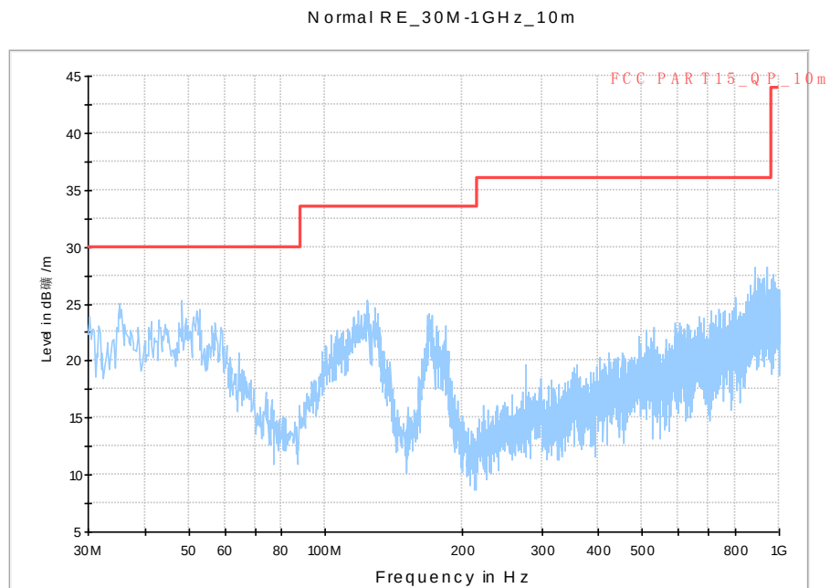
Fig. 52 Radiated Spurious Emission (802.11n-HT20, Ch157, 30 MHz-1 GHz)
