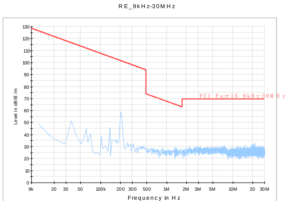
Fig. 80 Radiated Spurious Emission (802.11a, ch157, 9 kHz ~30 MHz)
