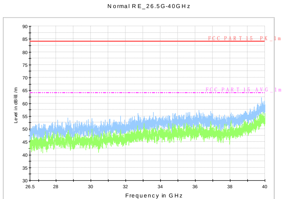
Fig. 47 Radiated emission: 802.11n, (802.11a, Ch157, 26.5 GHz - 40 GHz)
