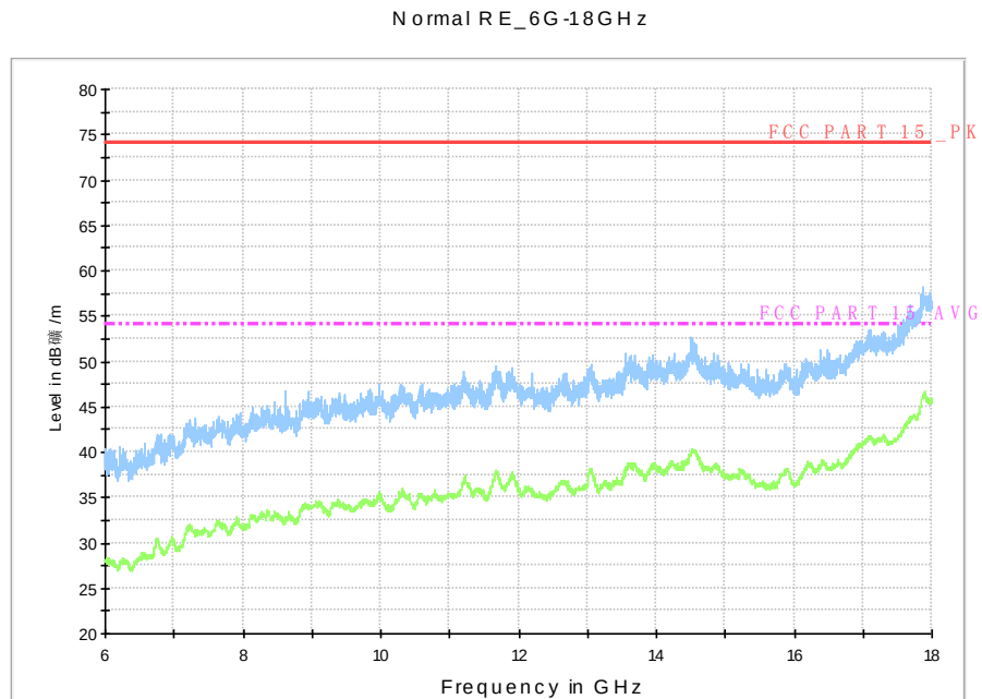
Fig. 61 Radiated Spurious Emission (802.11n-HT40, Ch151, 6 GHz-18 GHz)
