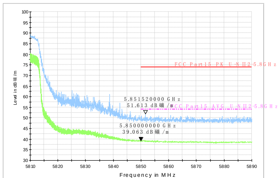
Fig. 77 Band Edges (802.11n-HT40, 5795MHz)
