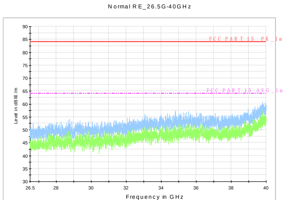
Fig. 56 Radiated emission: 802.11n, (802.11n-HT20, Ch157, 26.5 GHz - 40 GHz)
