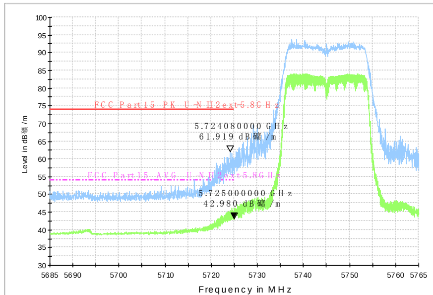
Fig. 74 Band Edges (802.11n-HT20, 5745MHz)
