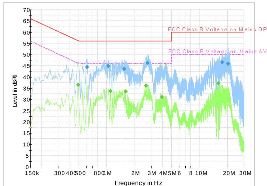
Fig. 79 AC Powerline Conducted Emission-Idle
