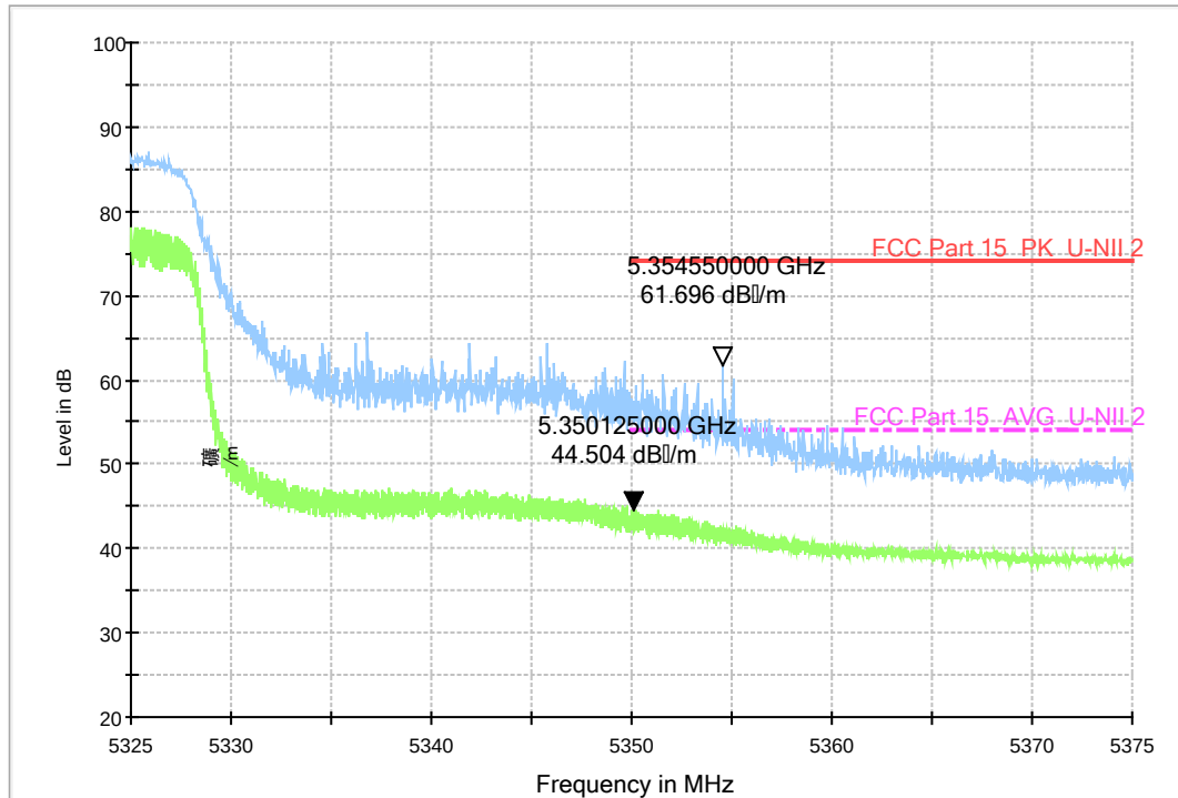
Fig. 47 Band Edges (802.11n-HT40, 5310MHz)
