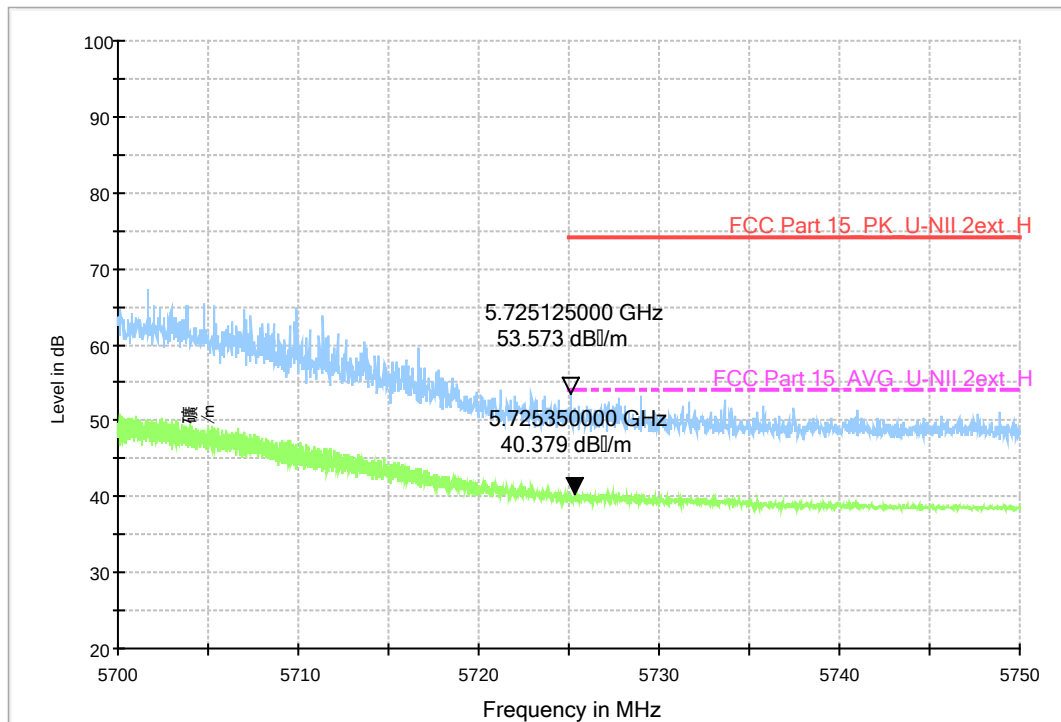
Fig. 49 Band Edges (802.11n-HT40, 5670MHz)
