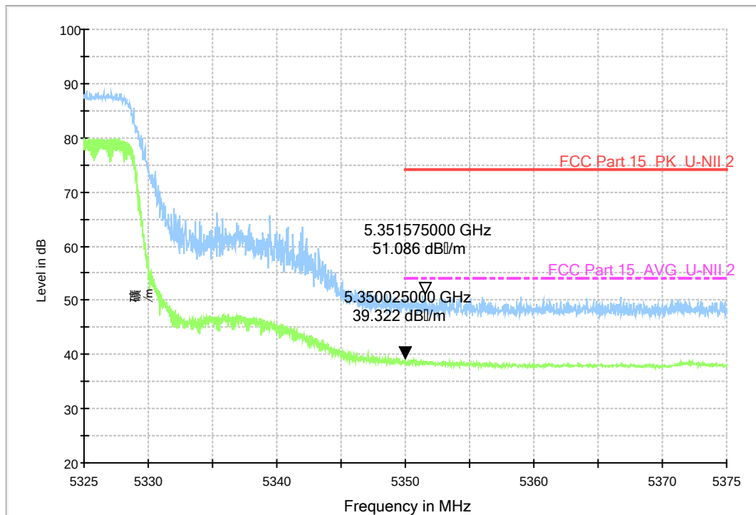
Fig. 43 Band Edges (802.11n-HT20, 5320MHz)
