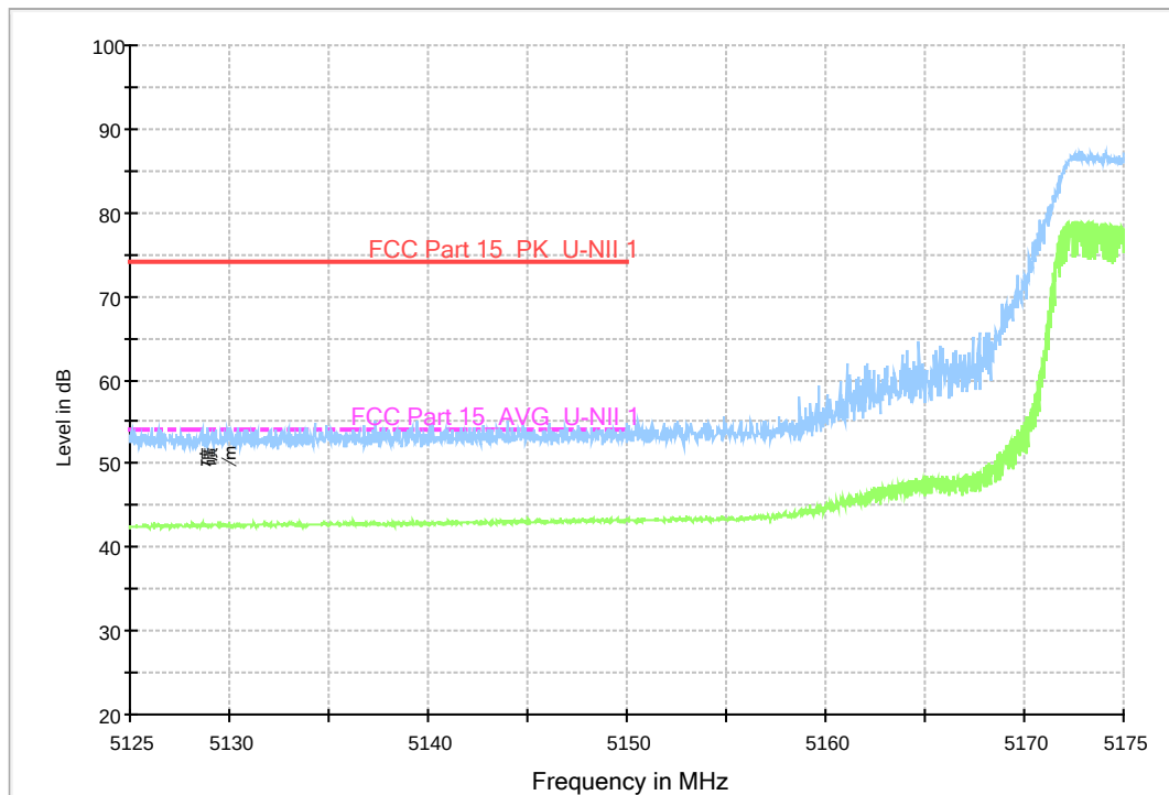
Fig. 38 Band Edges (802.11a, 5180MHz)
