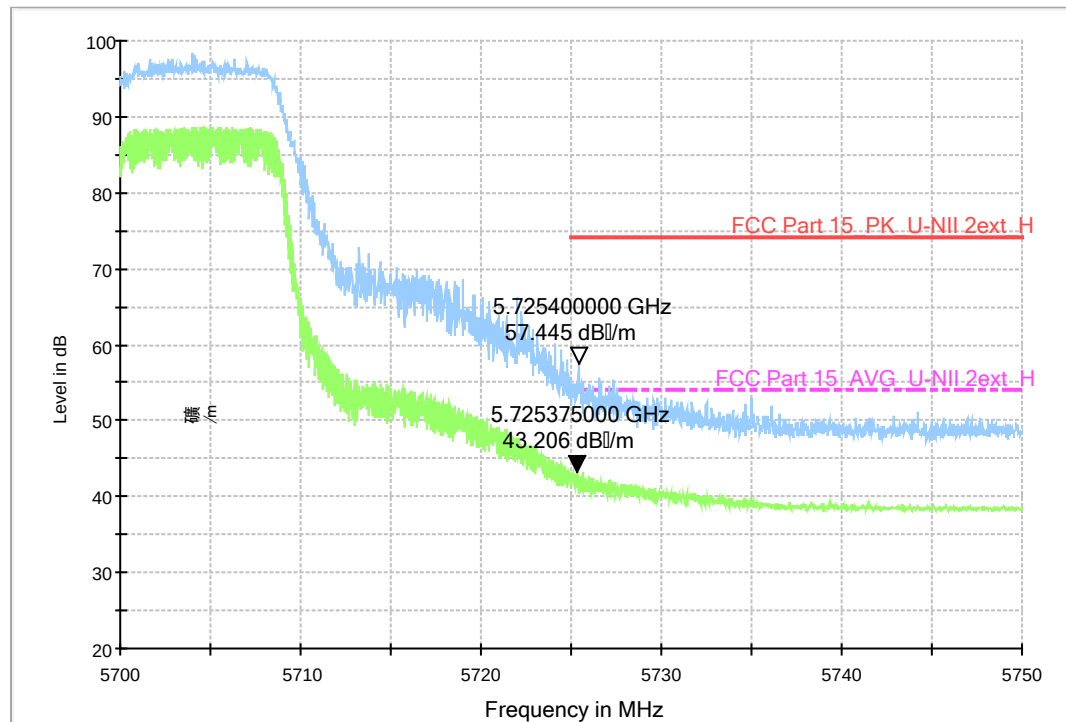
Fig. 45 Band Edges (802.11n-HT20, 5700MHz)
