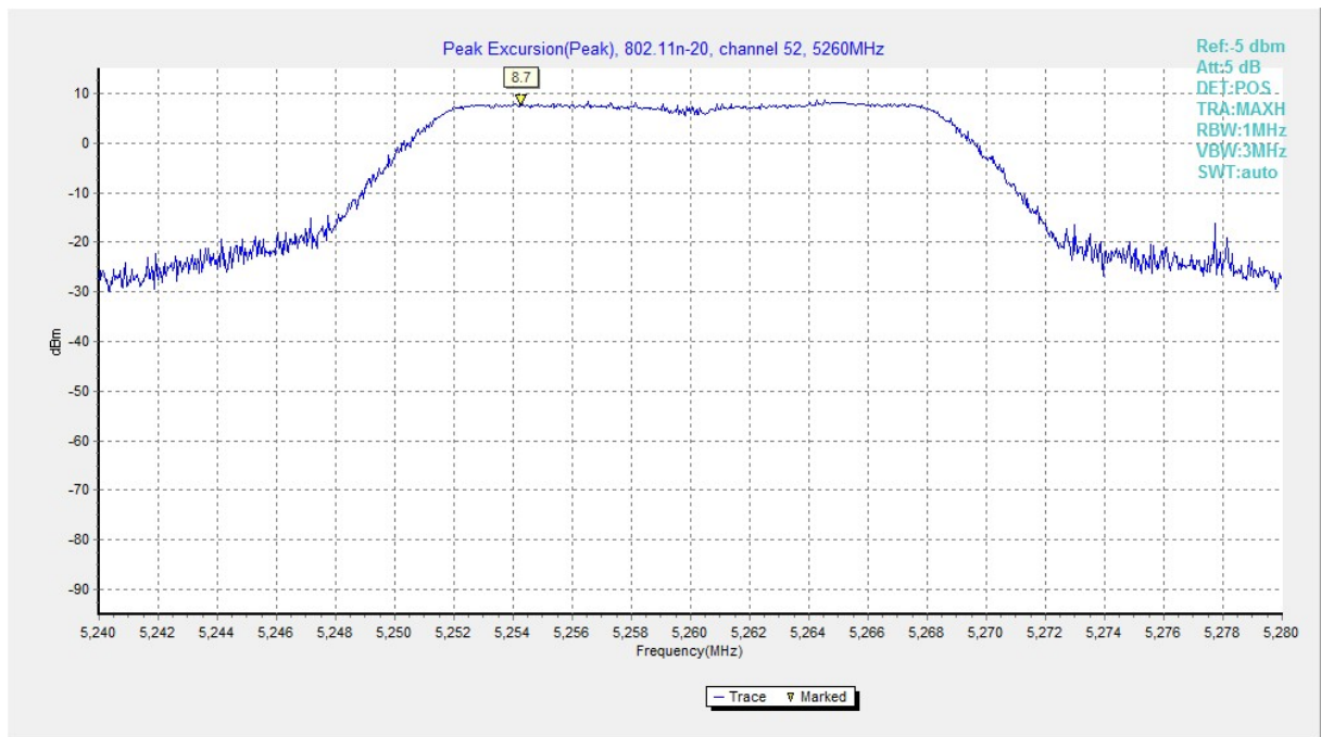
Fig. 153 Peak Excursions (802.11n-HT20, ch52, peak)
