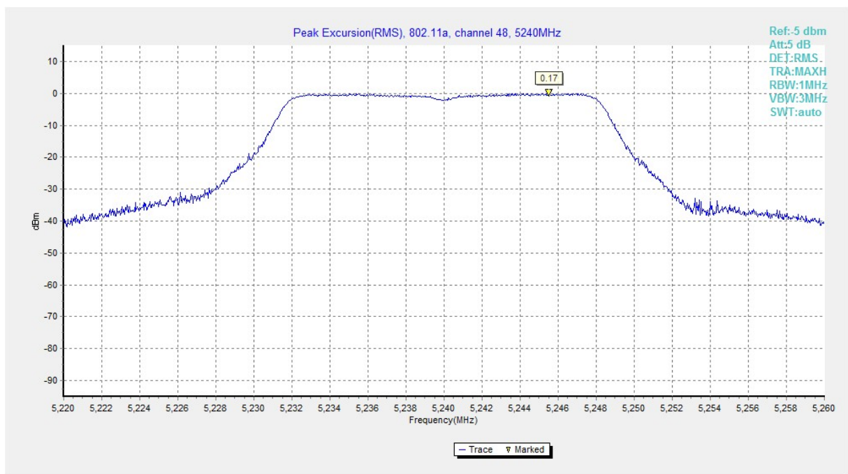
Fig. 134 Peak Excursions (802.11a, ch48, average)
