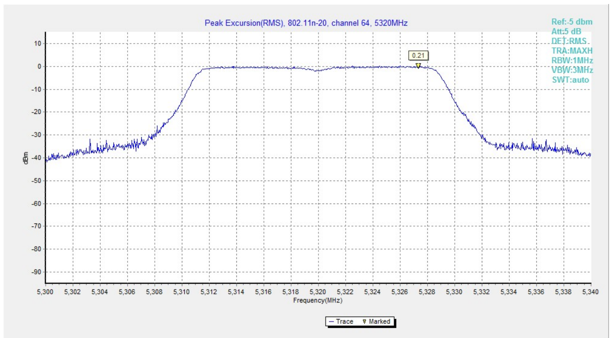
Fig. 158 Peak Excursions (802.11n-HT20, ch64, average)
