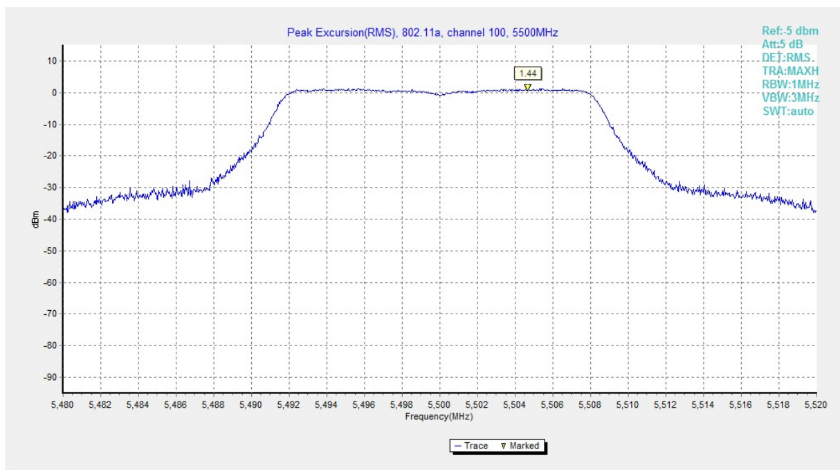
Fig. 144 Peak Excursions (802.11a, ch100, average)
