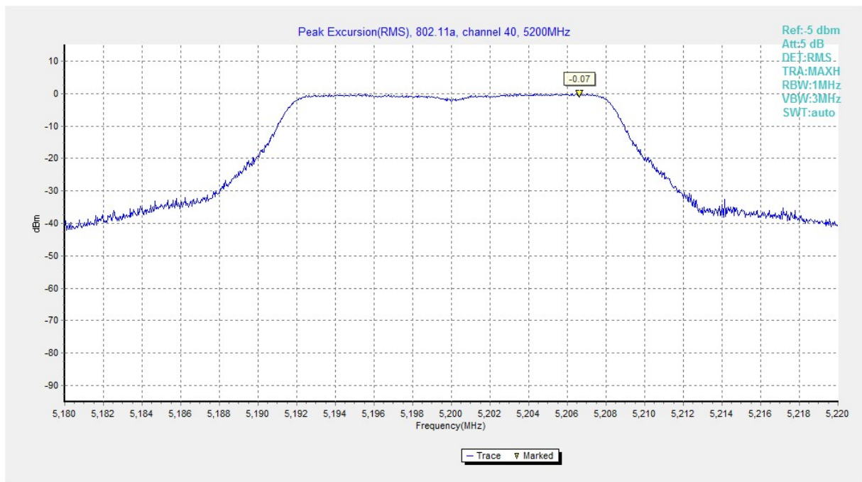
Fig. 133 Peak Excursions (802.11a, ch40, average)
