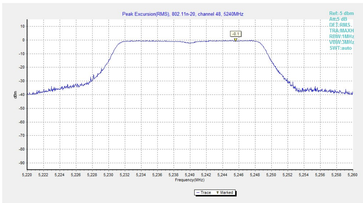
Fig. 152 Peak Excursions (802.11n-HT20, ch48, average)
