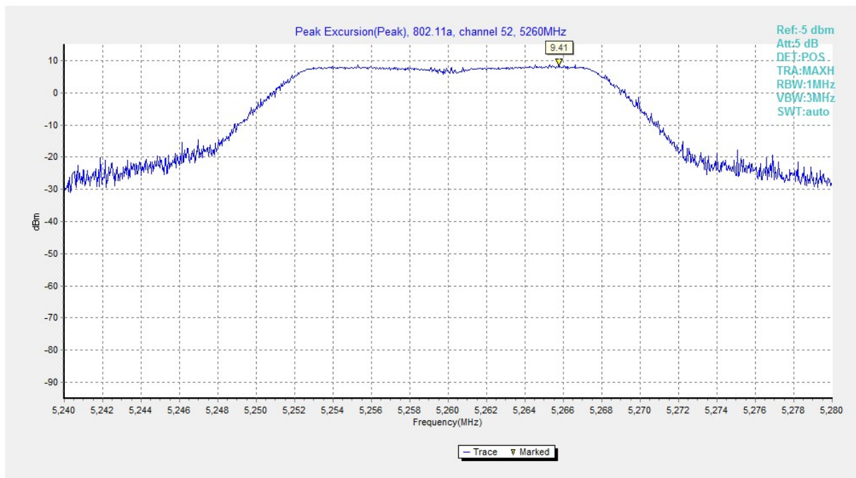
Fig. 135 Peak Excursions (802.11a, ch52, peak)
