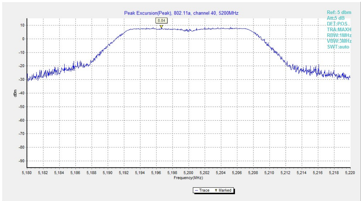
Fig. 130 Peak Excursions (802.11a, ch40, peak)
