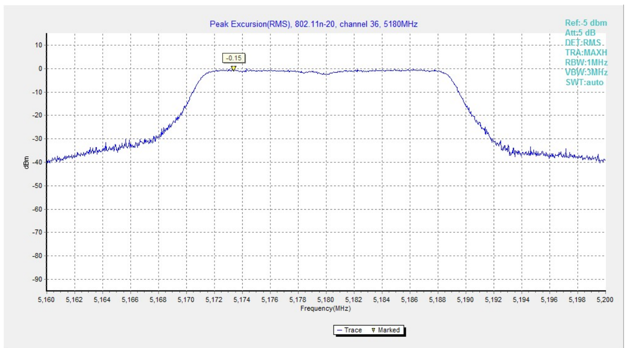
Fig. 150 Peak Excursions (802.11n-HT20, ch36, average)
