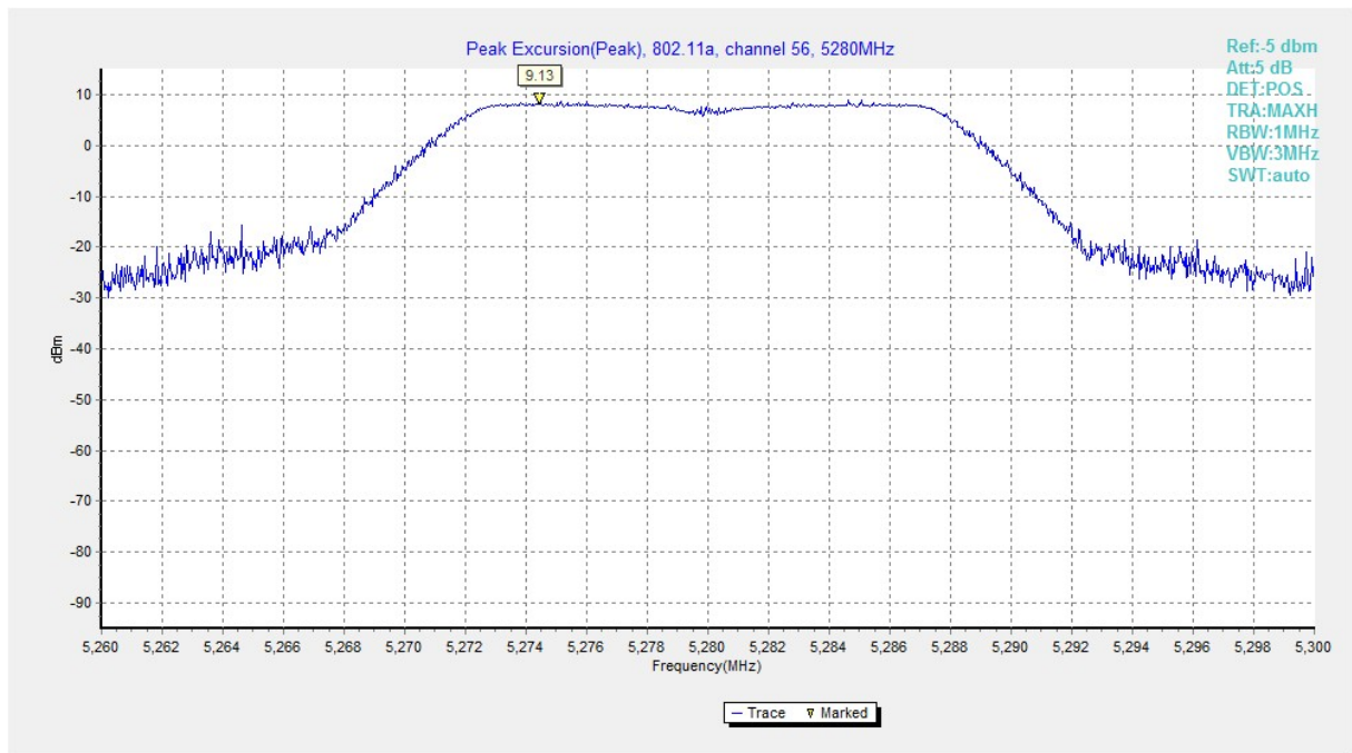
Fig. 136 Peak Excursions (802.11a, ch56, peak)
