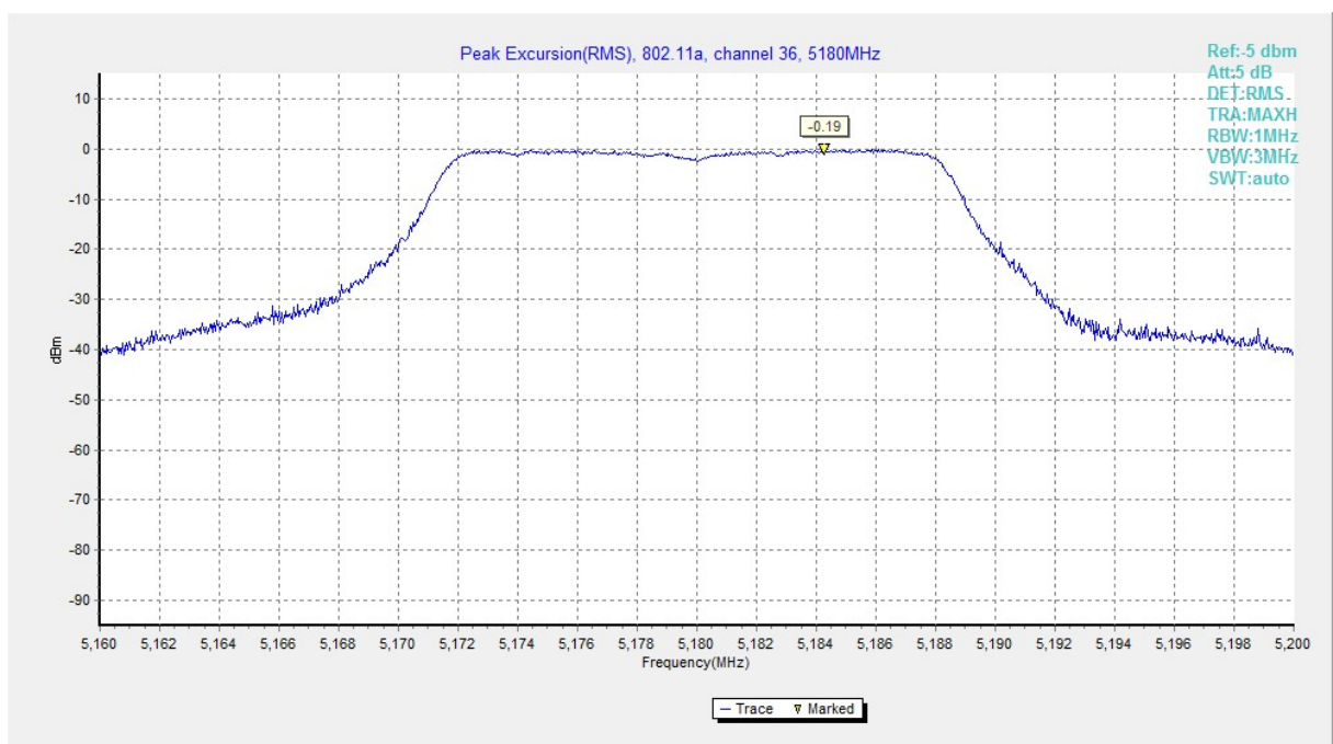
Fig. 132 Peak Excursions (802.11a, ch36, average)
