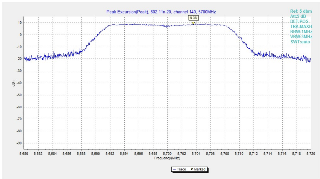
Fig. 161 Peak Excursions (802.11n-HT20, ch140, peak)
