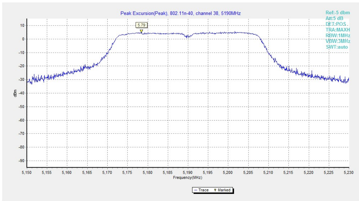
Fig. 165 Peak Excursions (802.11n-HT40, ch38, peak)
