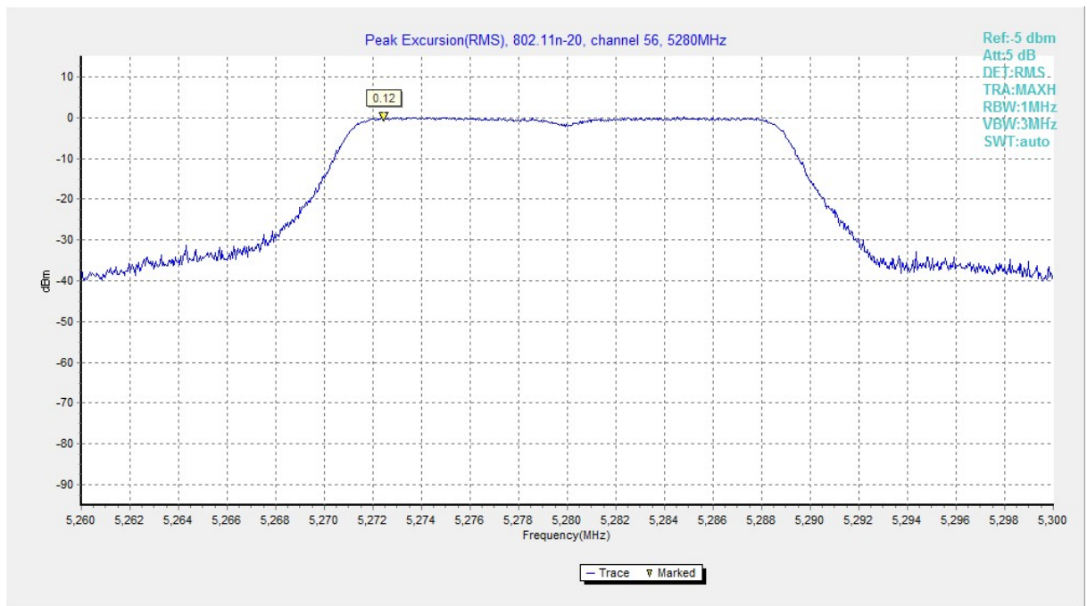
Fig. 157 Peak Excursions (802.11n-HT20, ch56, average)
