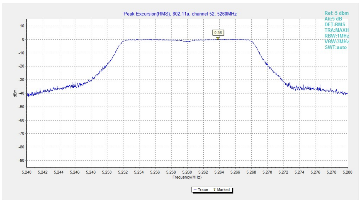
Fig. 138 Peak Excursions (802.11a, ch52, average)
