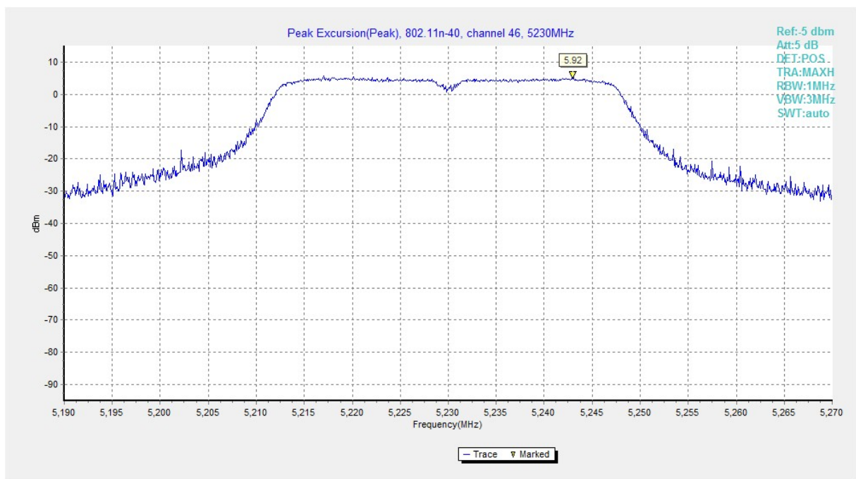
Fig. 166 Peak Excursions (802.11n-HT40, ch46, peak)
