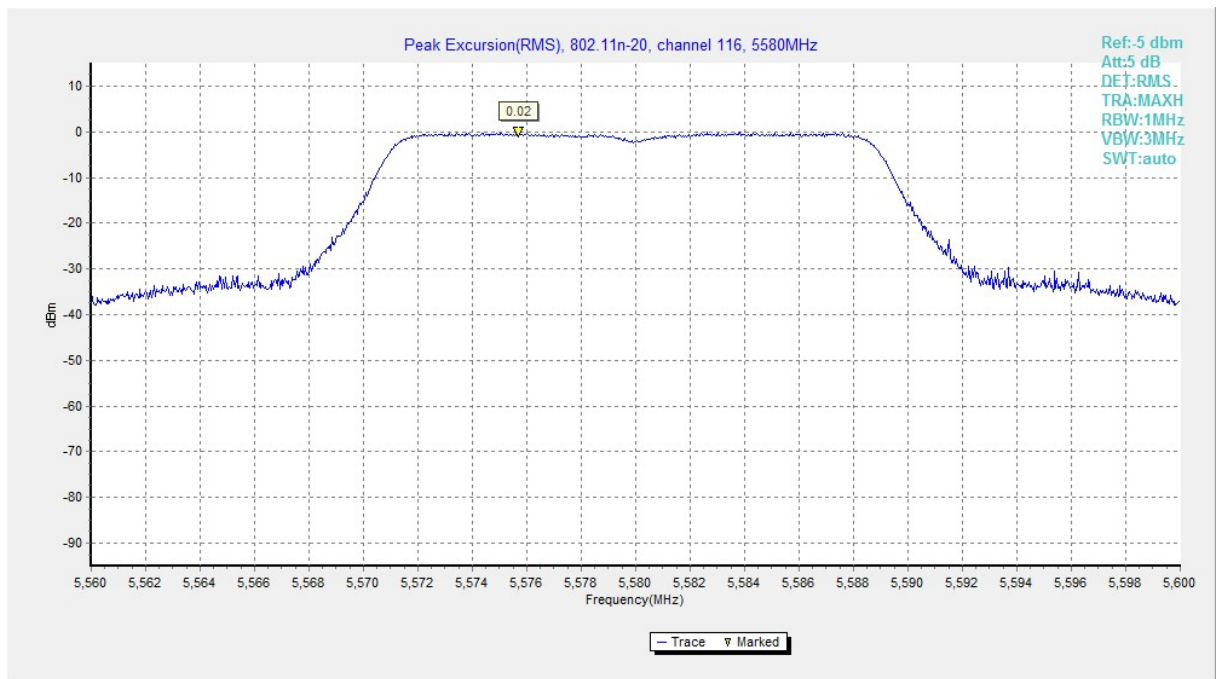
Fig. 163 Peak Excursions (802.11n-HT20, ch116, average)
