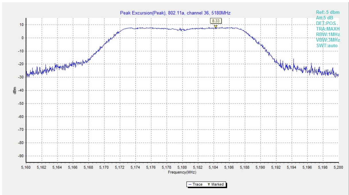
Fig. 129 Peak Excursions (802.11a, ch36, peak)
