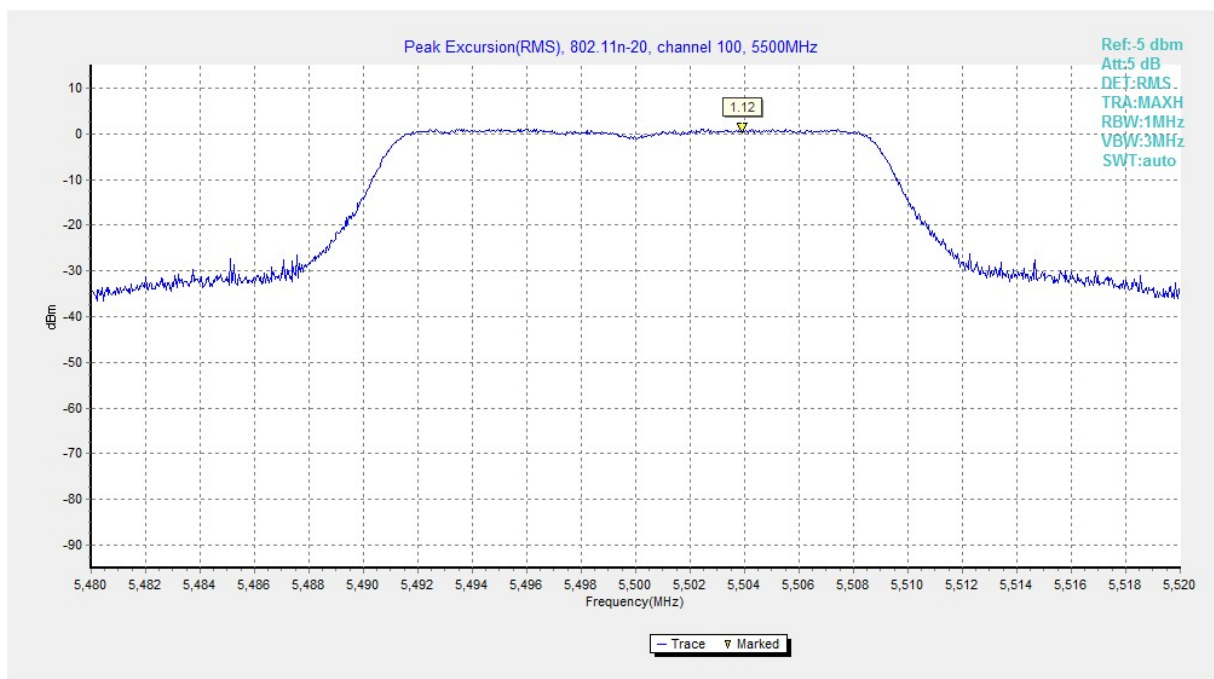
Fig. 162 Peak Excursions (802.11n-HT20, ch100, average)
