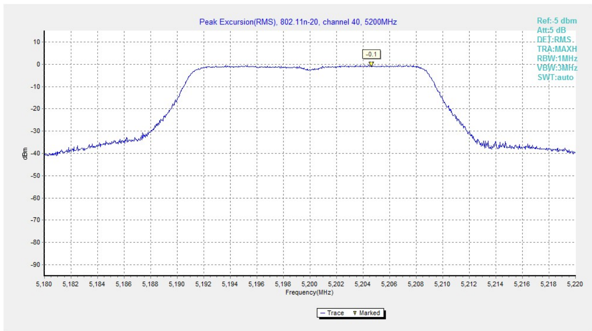
Fig. 151 Peak Excursions (802.11n-HT20, ch40, average)
