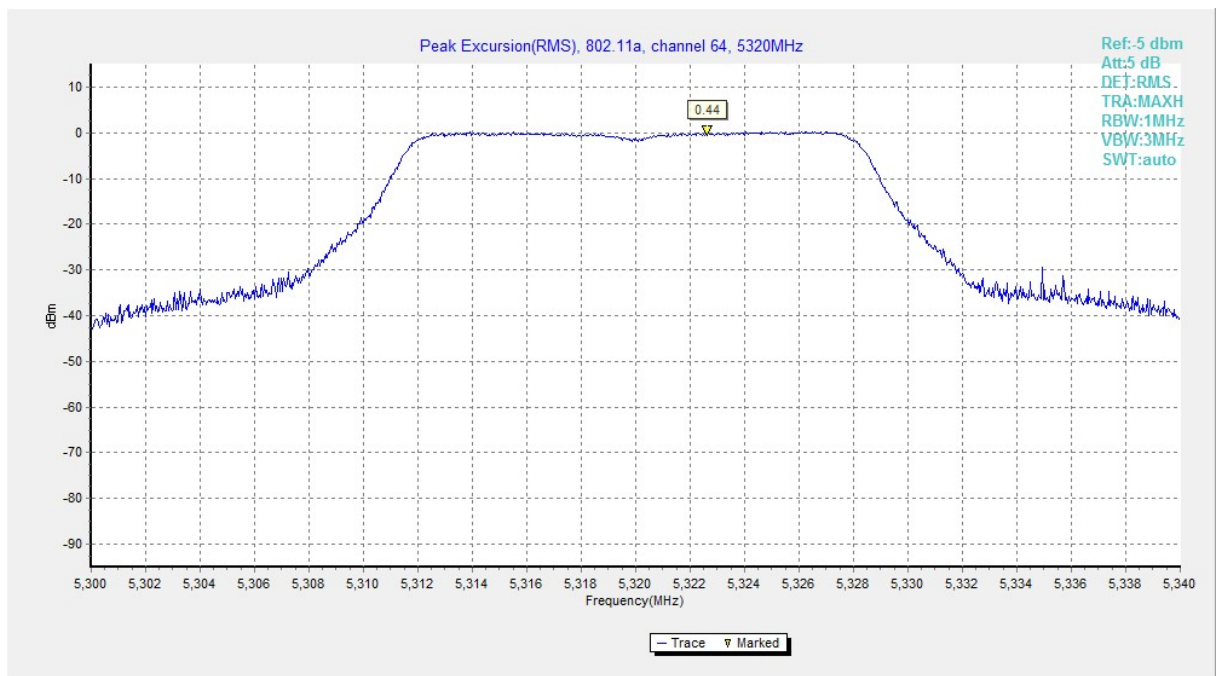
Fig. 140 Peak Excursions (802.11a, ch64, average)
