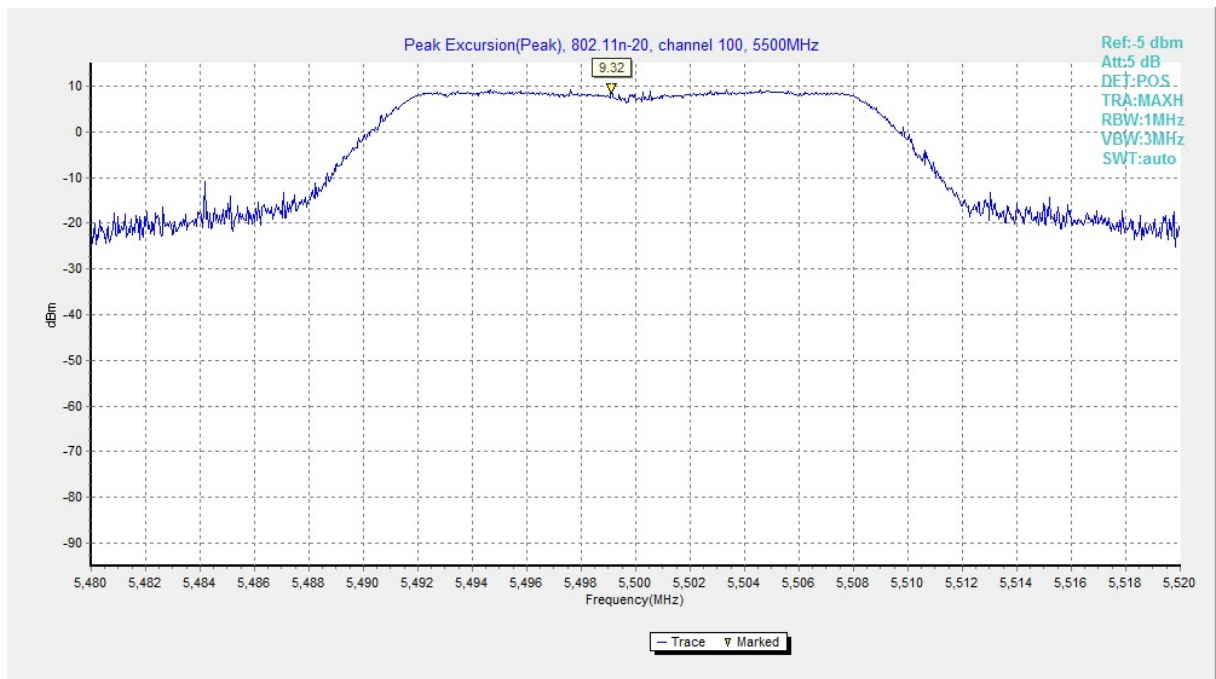
Fig. 159 Peak Excursions (802.11n-HT20, ch100, peak)
