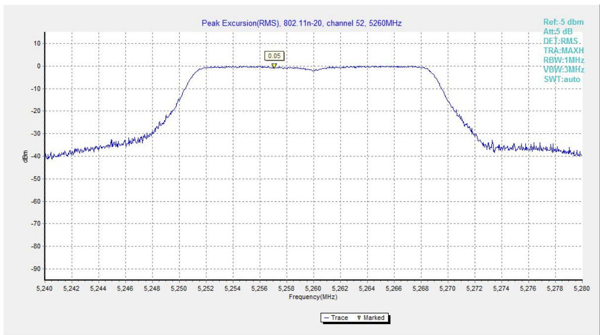
Fig. 156 Peak Excursions (802.11n-HT20, ch52, average)
