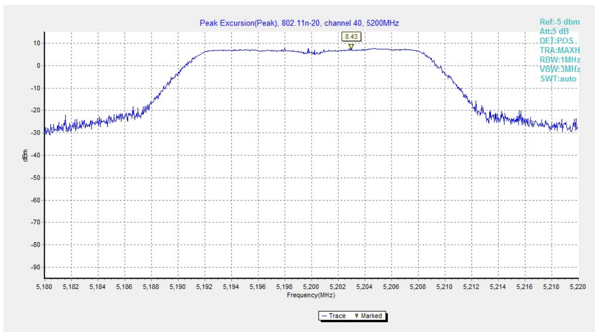
Fig. 148 Peak Excursions (802.11n-HT20, ch40, peak)
