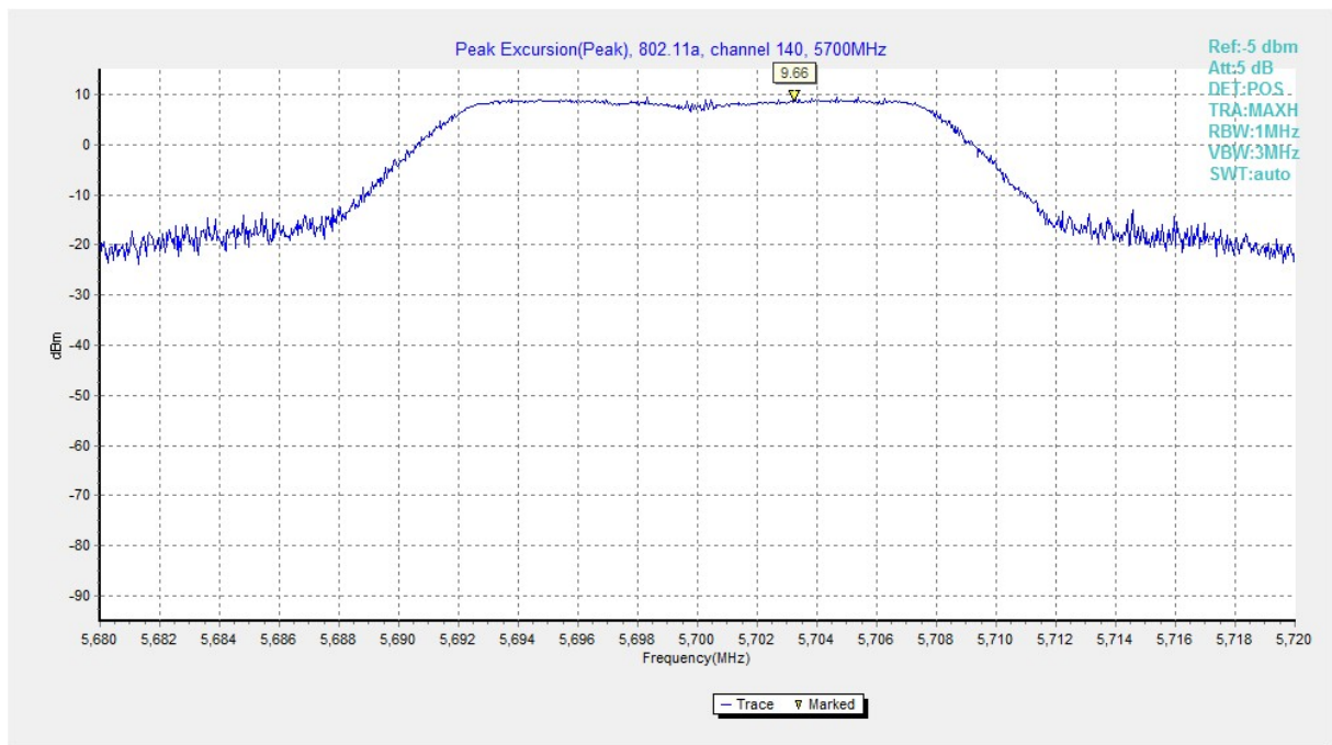
Fig. 143 Peak Excursions (802.11a, ch140, peak)
