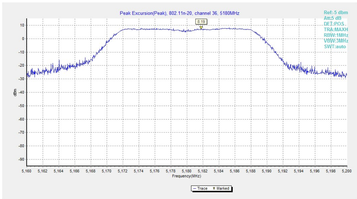
Fig. 147 Peak Excursions (802.11n-HT20, ch36, peak)
