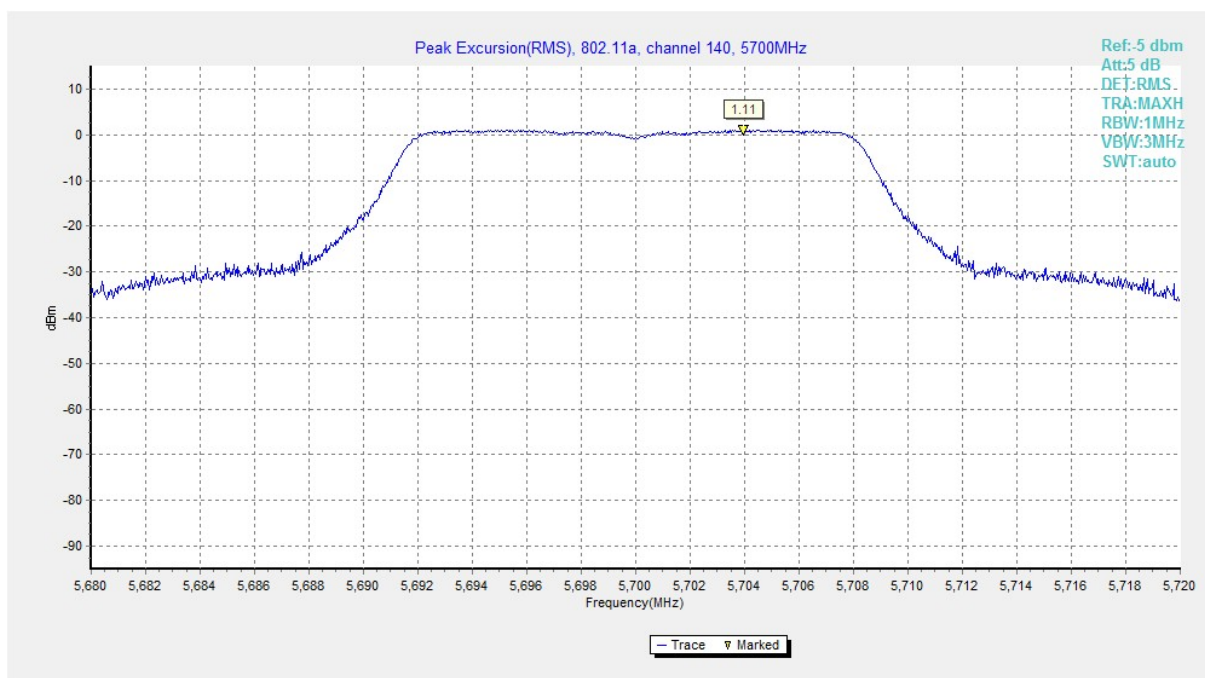
Fig. 146 Peak Excursions (802.11a, ch140, average)
