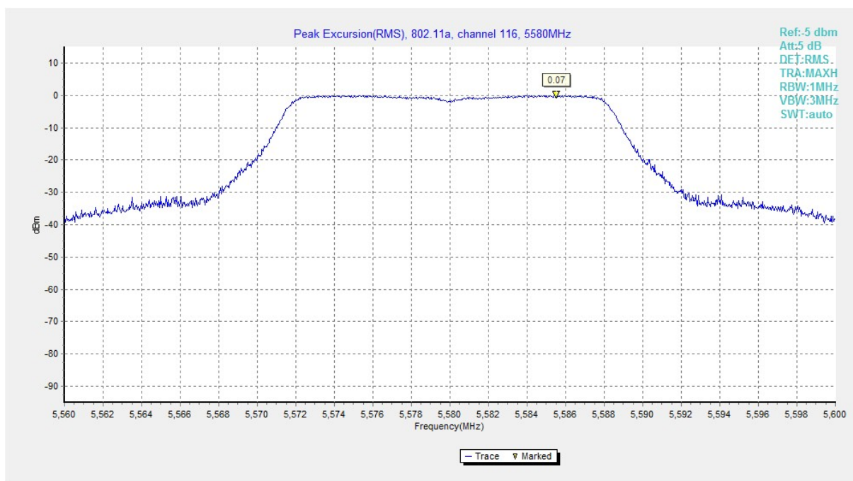
Fig. 145 Peak Excursions (802.11a, ch116, average)
