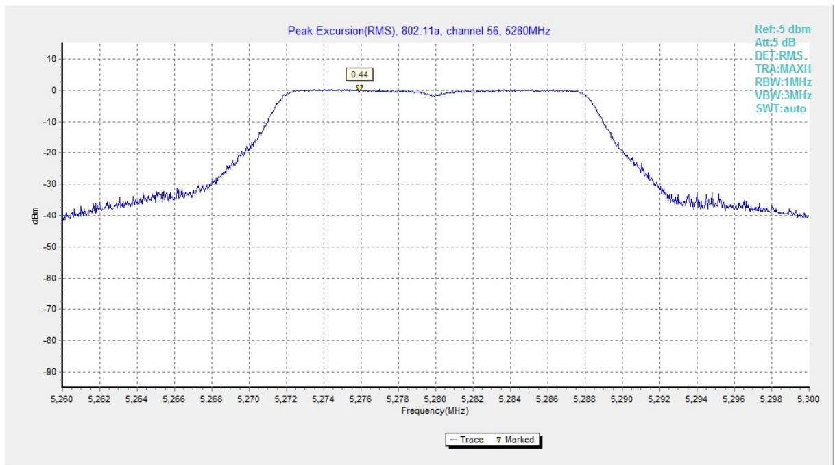
Fig. 139 Peak Excursions (802.11a, ch56, average)
