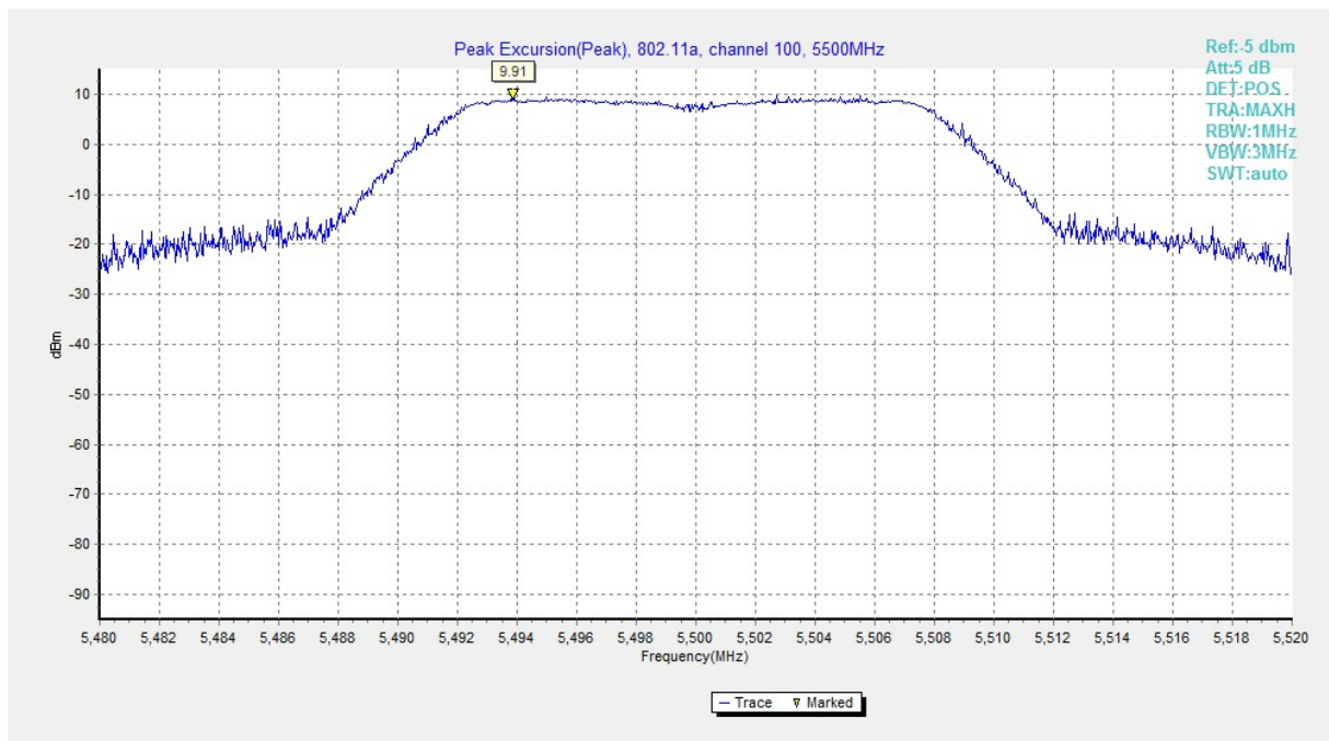
Fig. 141 Peak Excursions (802.11a, ch100, peak)
