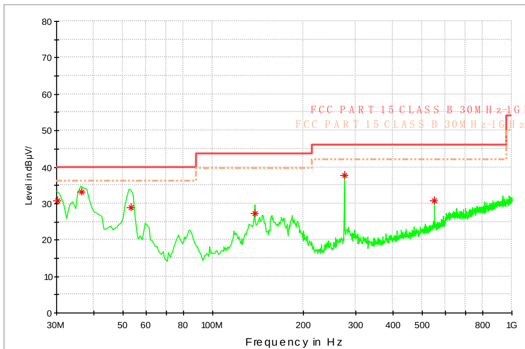
FCC CLASS B RE 30MHz-1GHz
