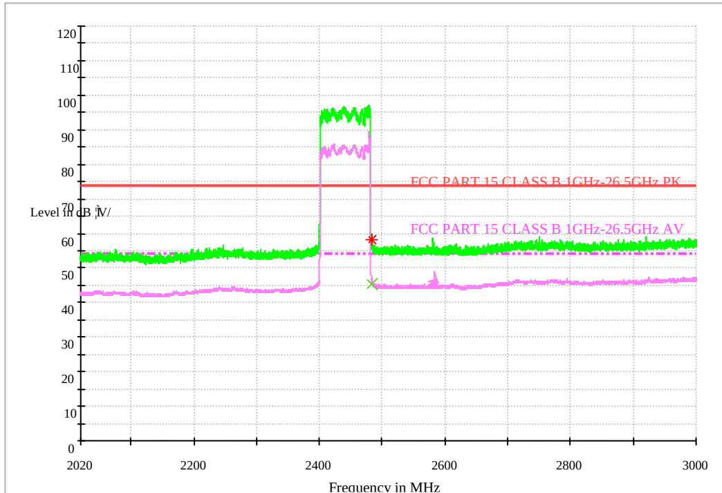
FCC CLASS B WIFI 1GHz-3GHz
