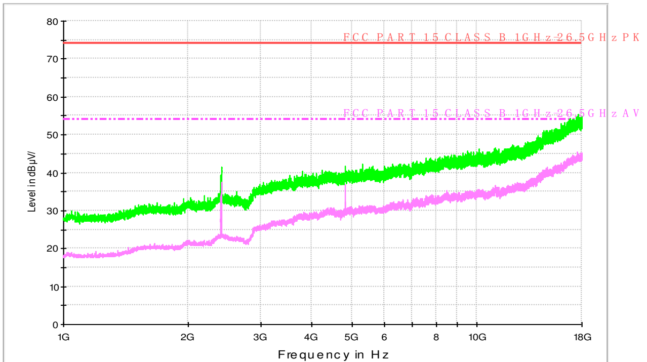
FCC CLASS B RE 1GHz-18GHz
