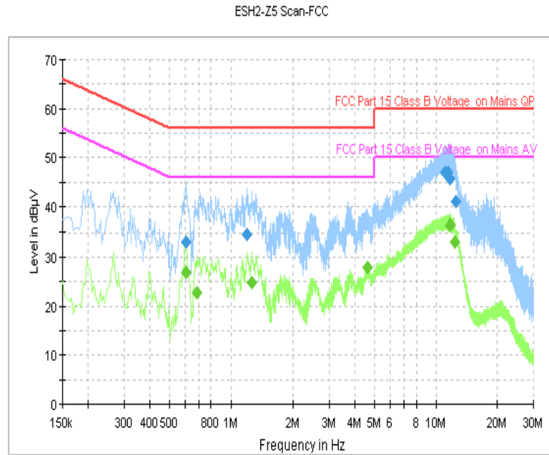
Fig. 41 AC Power line Conducted Emission (Idle, AE4)
