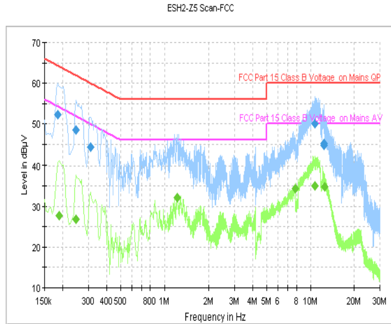
Fig. 35 AC Power line Conducted Emission (Traffic, AE6)
