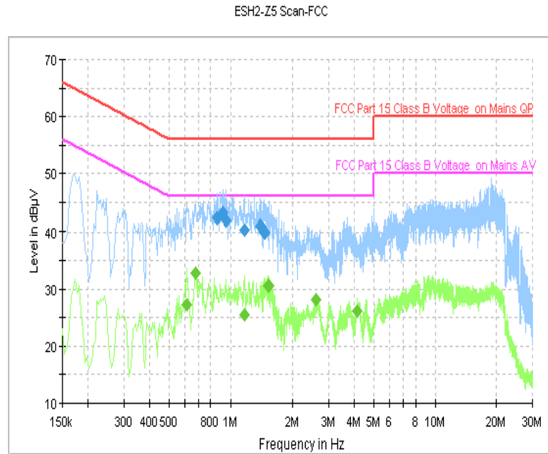
Fig. 37 AC Power line Conducted Emission (Traffic, AE8)
