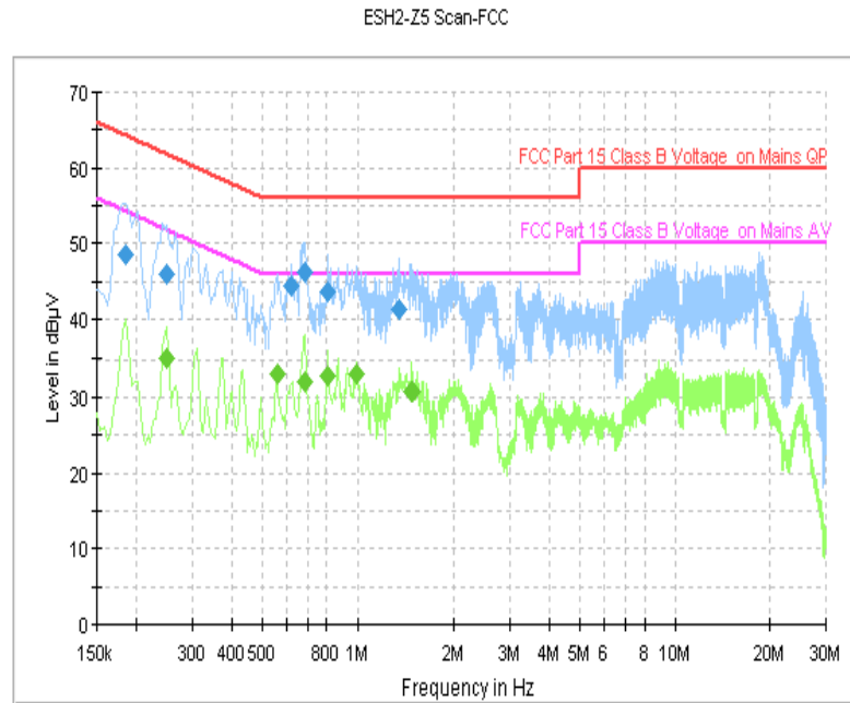
Fig. 32 AC Power line Conducted Emission (Traffic, AE3)
