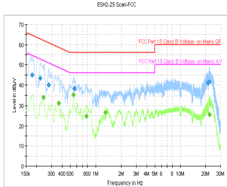
Fig. 39 AC Power line Conducted Emission (Idle, AE2)
