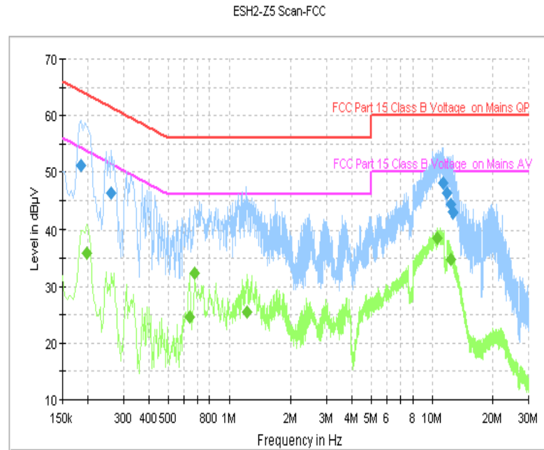
Fig. 42 AC Power line Conducted Emission (Idle, AE5)
