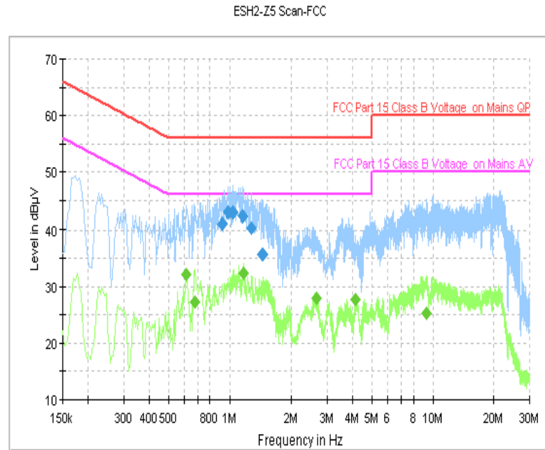
Fig. 45 AC Power line Conducted Emission (Idle, AE8)
