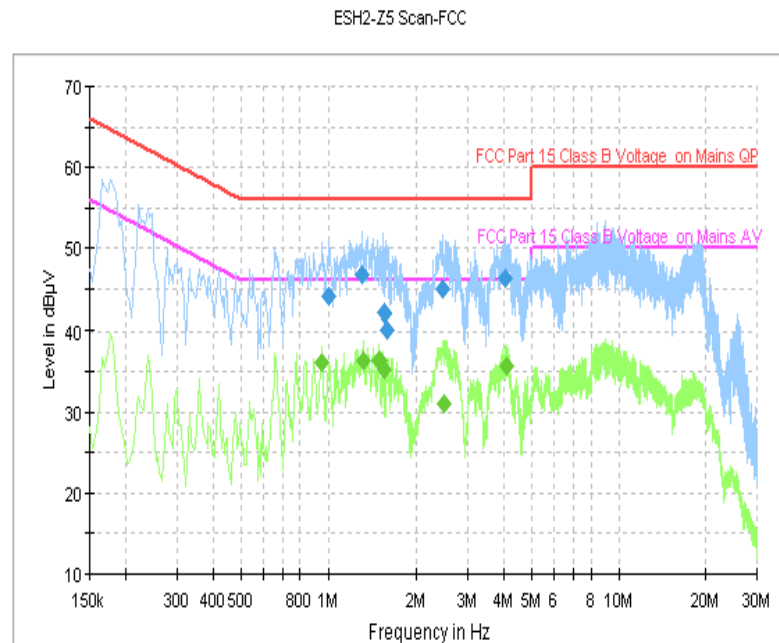
Fig. 34 AC Power line Conducted Emission (Traffic, AE5)
