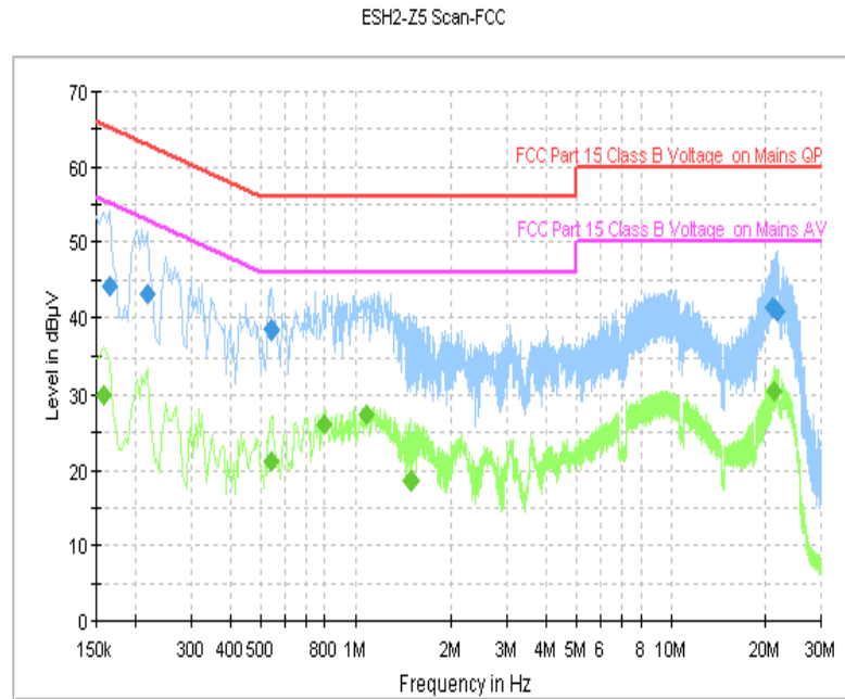
Fig. 38 AC Power line Conducted Emission (Idle, AE1)
