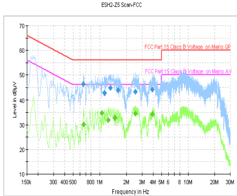
Fig. 43 AC Power line Conducted Emission (Idle, AE6)
