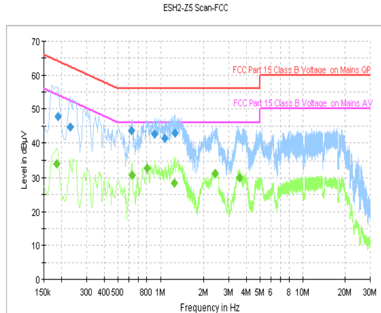
Fig. 36 AC Power line Conducted Emission (Traffic, AE7)
