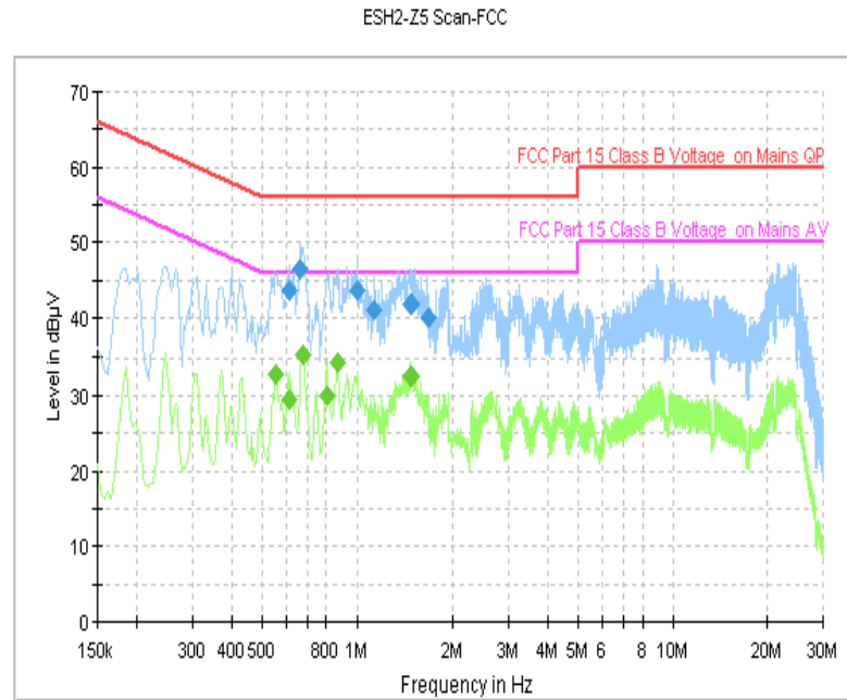
Fig. 40 AC Power line Conducted Emission (Idle, AE3)
