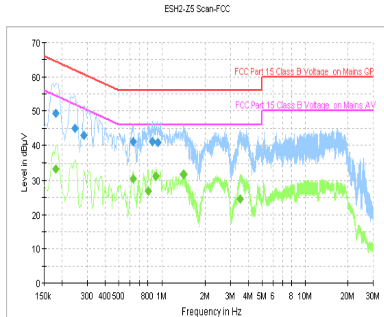
Fig. 33 AC Power line Conducted Emission (Traffic, AE4)
