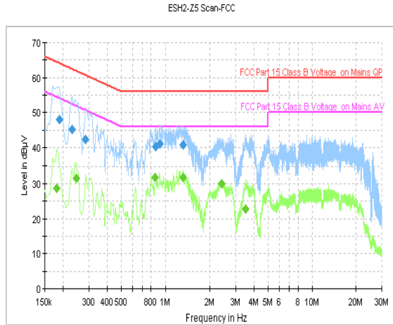
Fig. 44 AC Power line Conducted Emission (Idle, AE7)
