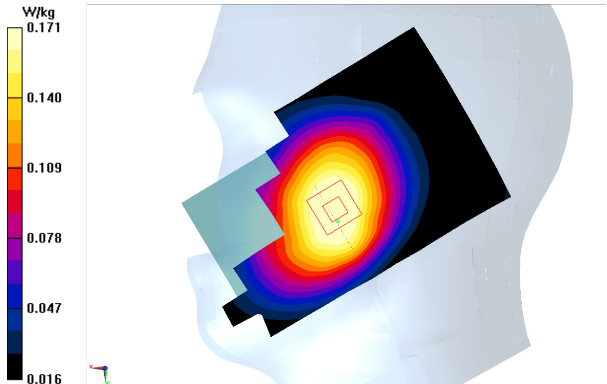
Fig.21 LTE Band17
