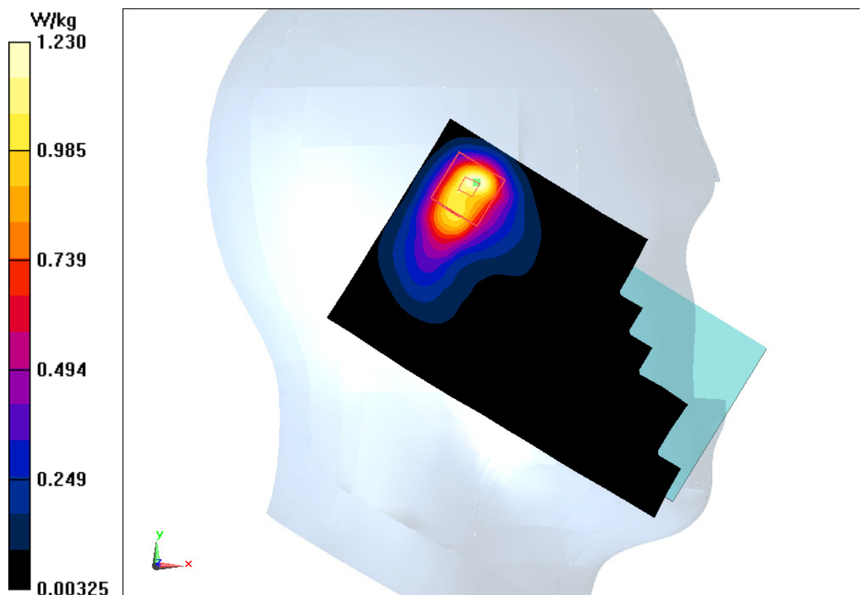
Fig.23 2450 MHz
