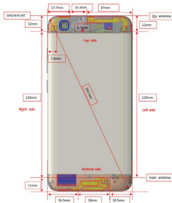
Picture 12.1 Antenna Locations
