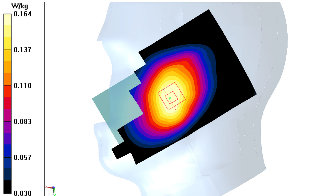
Fig.19 LTE Band12
