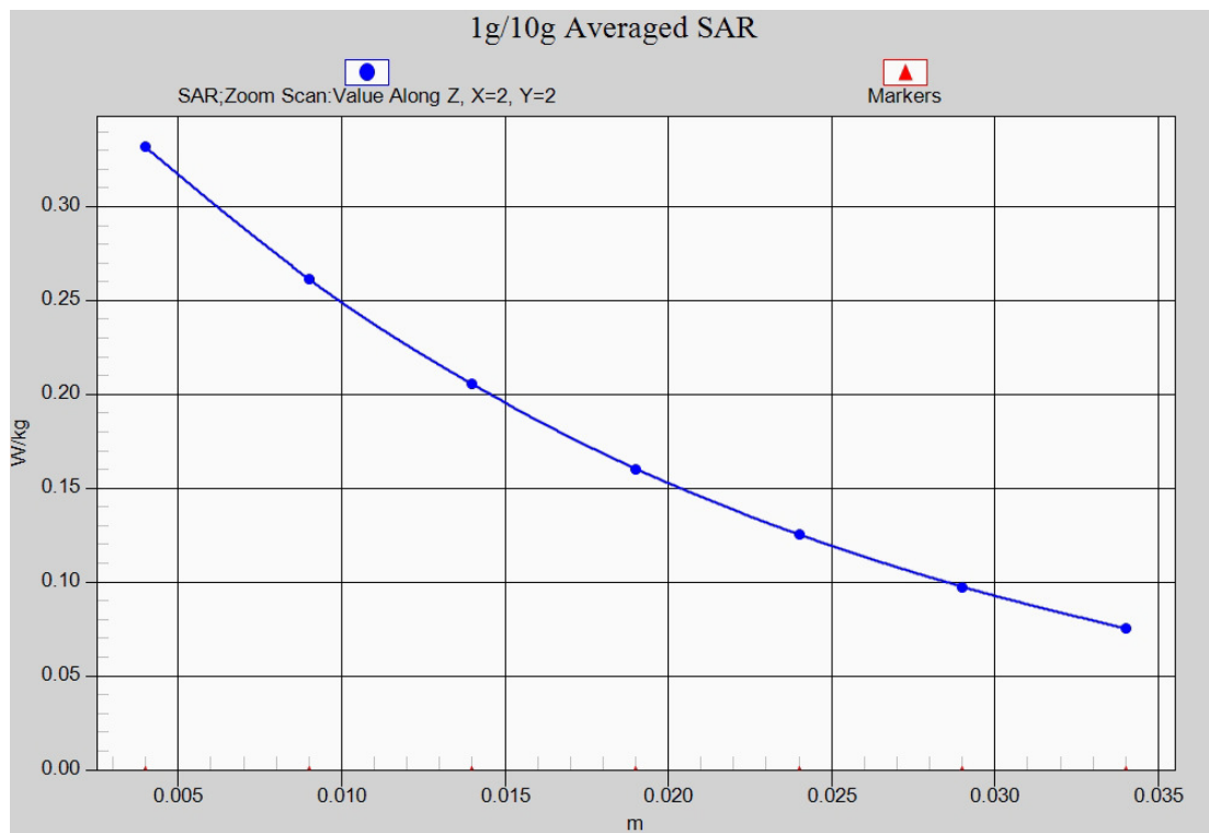
Fig. 20-1 Z-Scan at power reference point (LTE Band12)
