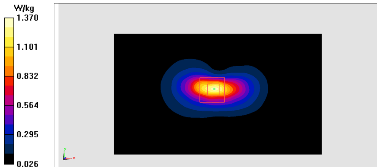
Fig.8 1700 MHz
