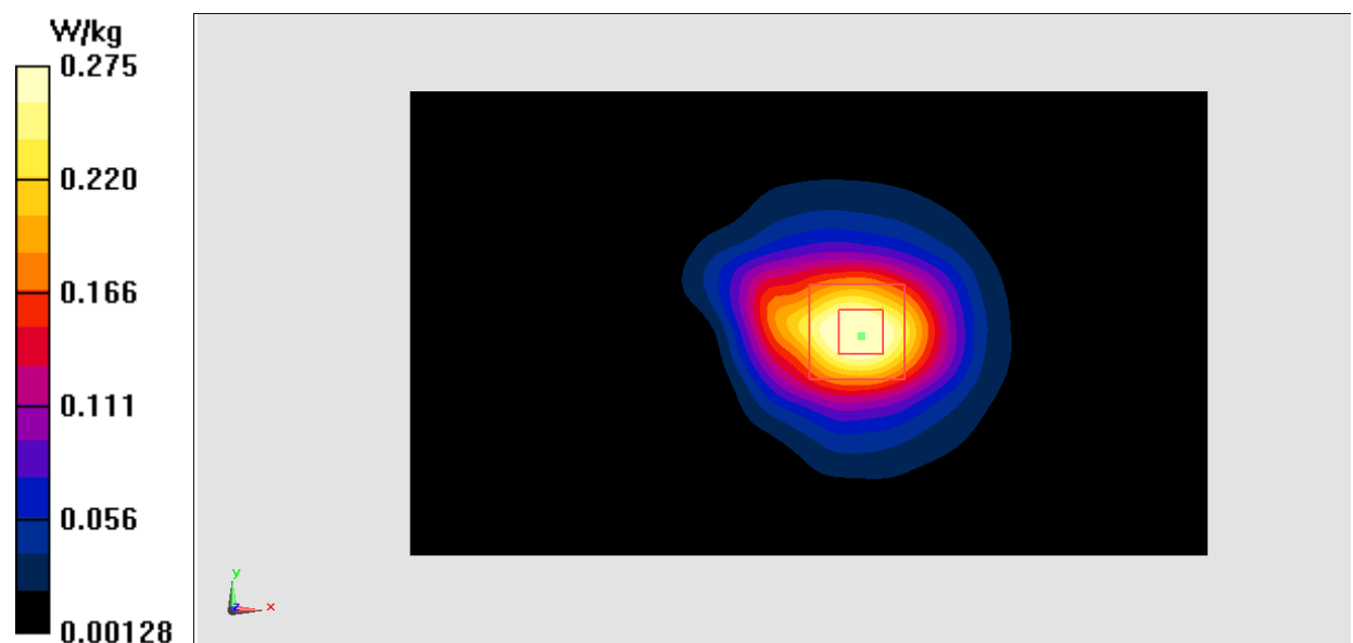
Fig.24 2450 MHz
