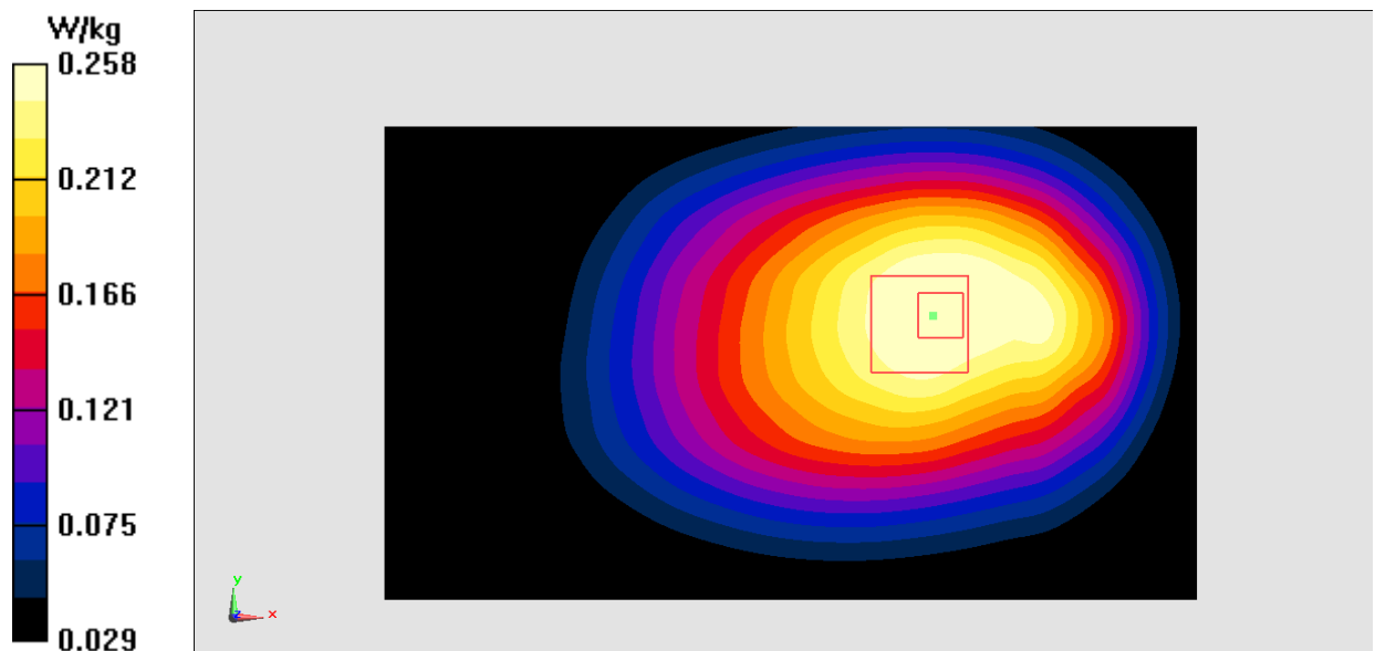
Fig.22 LTE Band17
