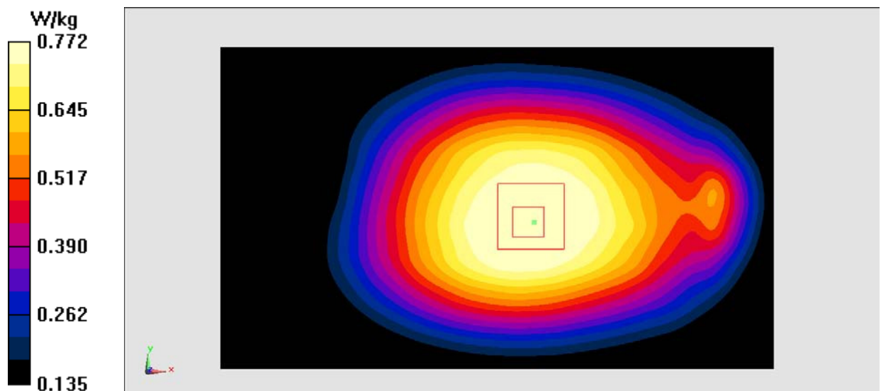
Fig.2 850 MHz
