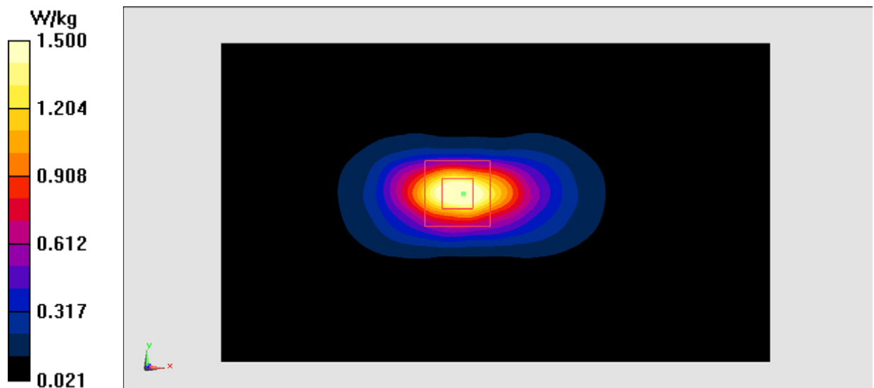
Fig.4 1900 MHz
