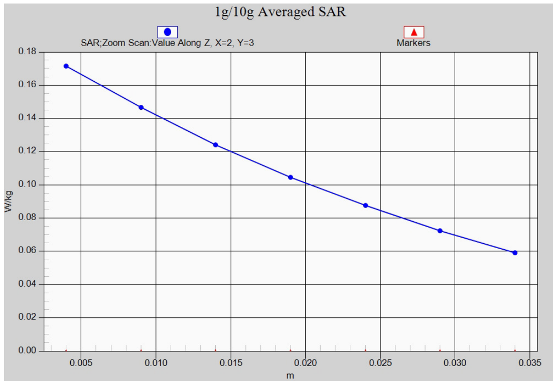
Fig. 21-1 Z-Scan at power reference point (LTE Band17)
