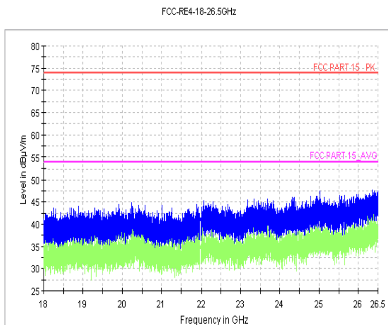
Fig.54 Radiated Spurious Emission (GFSK, Ch39, 18 GHz-26.5GHz)
