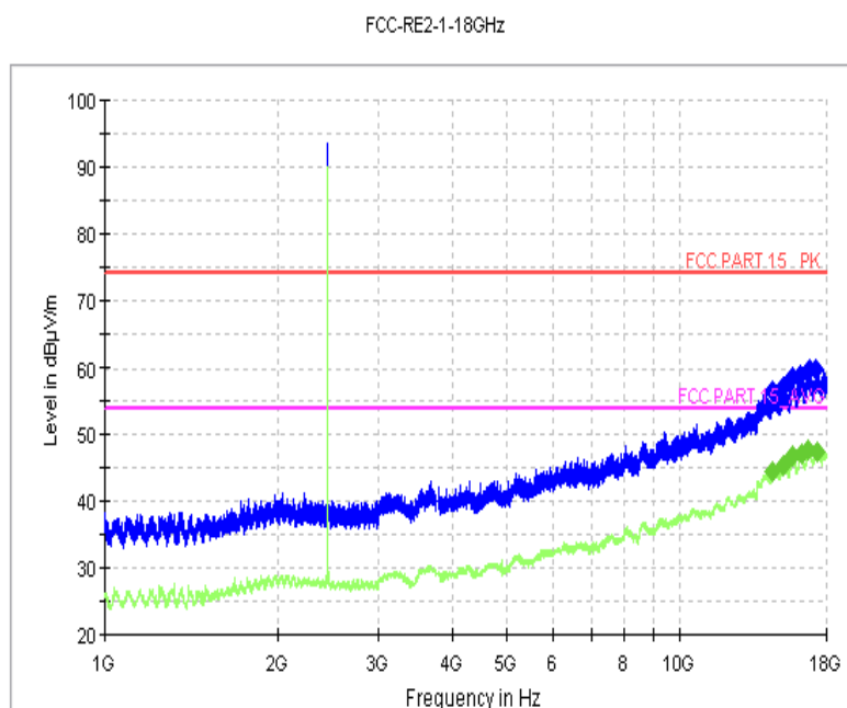
Fig.53 Radiated Spurious Emission (GFSK, Ch39, 1 GHz-18GHz)
