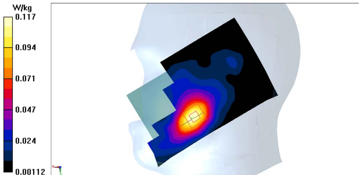
Fig.3 1900 MHz
