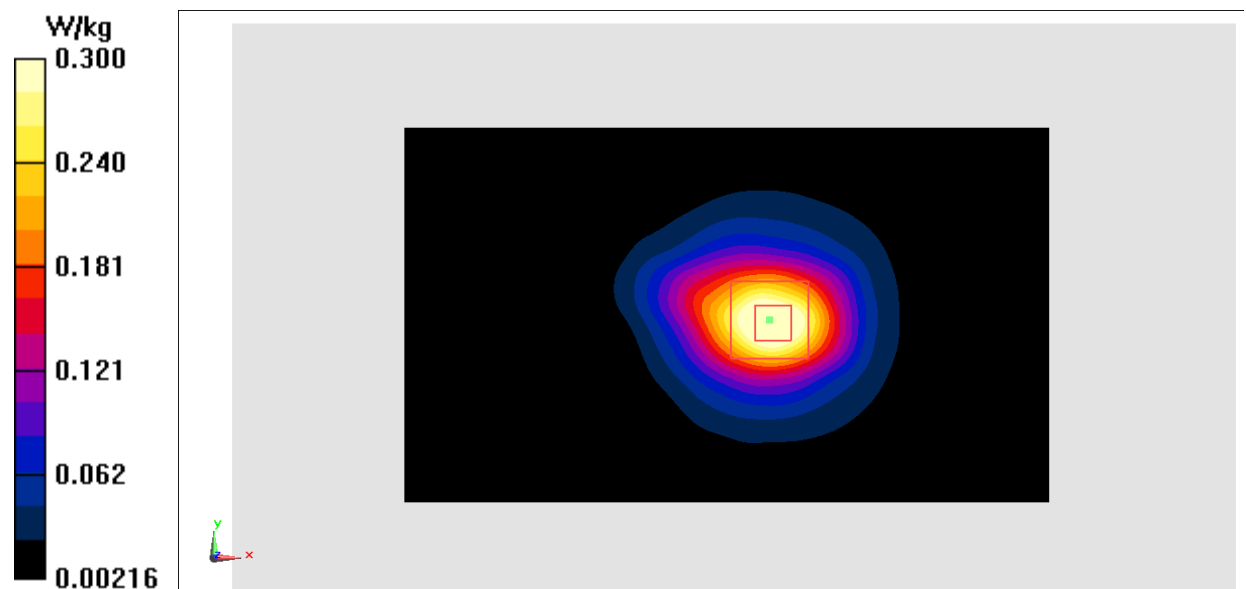
Fig.20 2450 MHz
