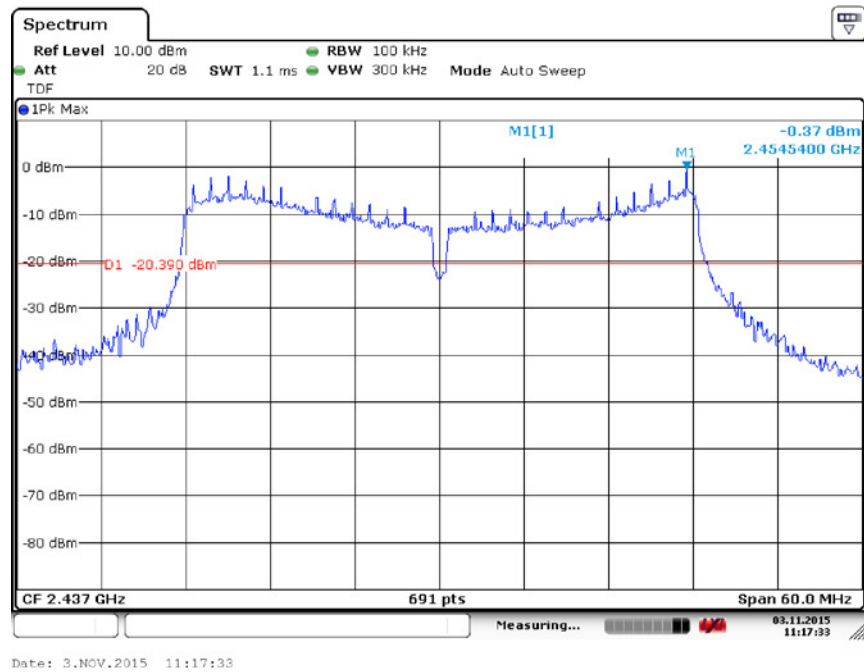
Fig.147 Conducted Spurious Emission (802.11n-40M, Ch6, Center Frequency)
