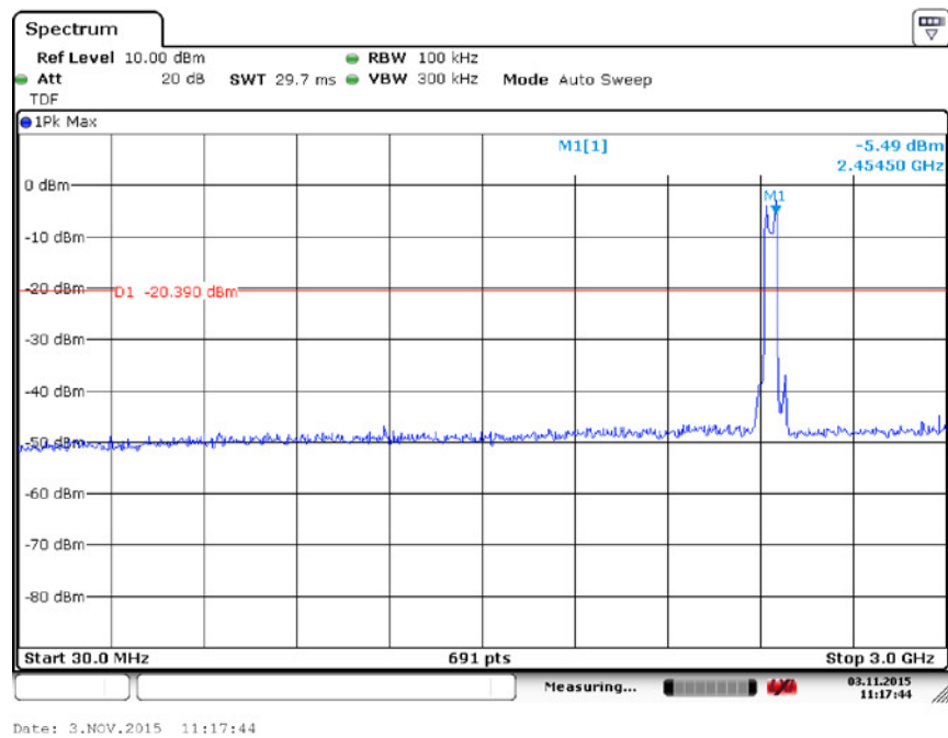
Fig.148 Conducted Spurious Emission (802.11n-40M, Ch6, 30 MHz-3 GHz)
