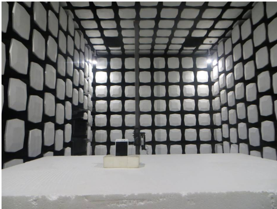
8. Radiated Emissions (Part 15C) (18GHz-26.5GHz)
