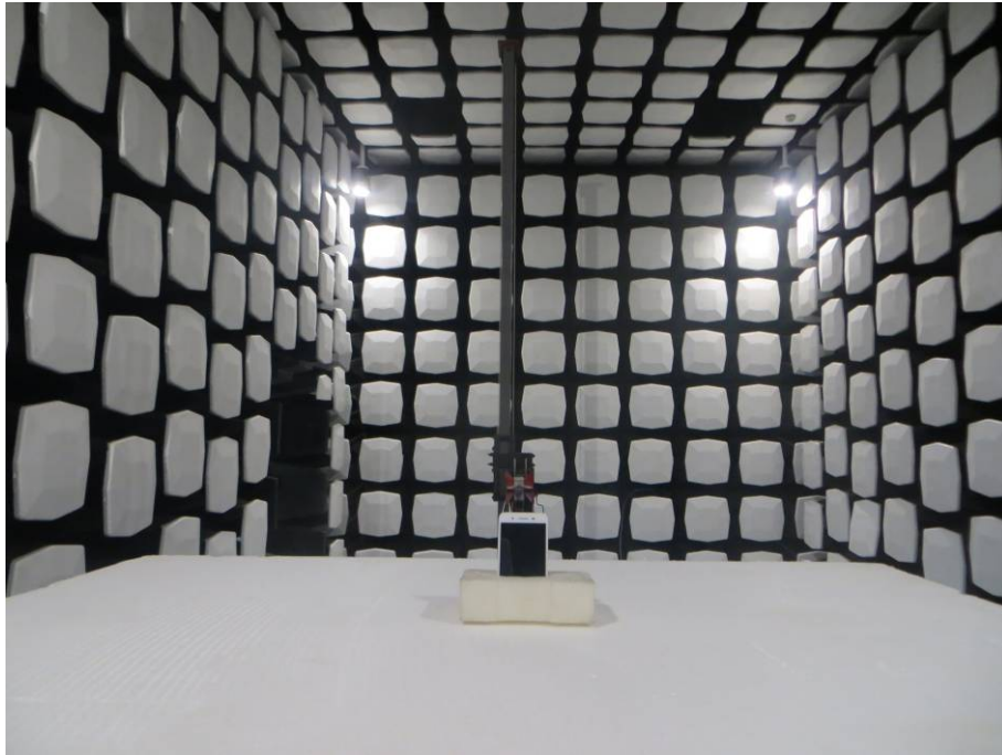
7. Radiated Emissions (Part 15C) (1GHz-18GHz)
