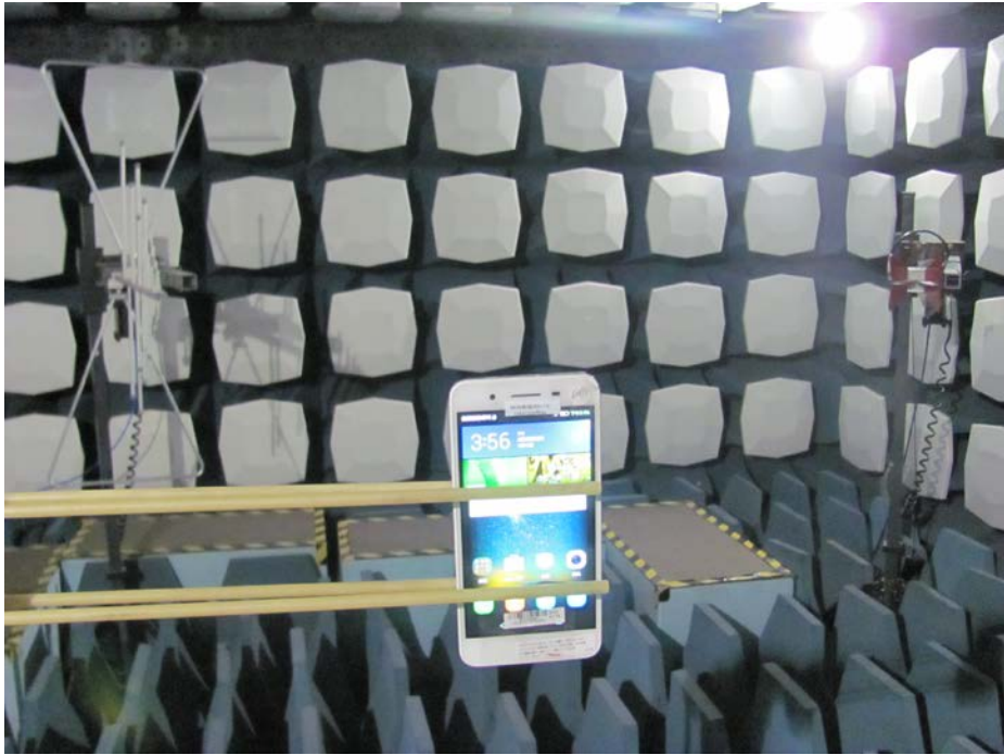
11. Radiated Emissions (Part 22/24/27) (below 3GHz)
