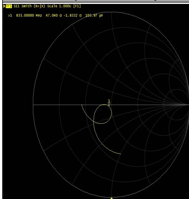
Impedance Test-Body
