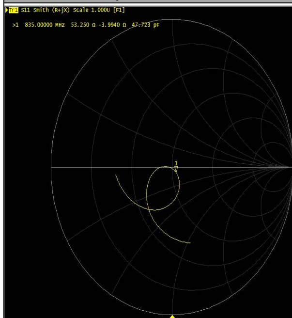
Impedance Test-Body
