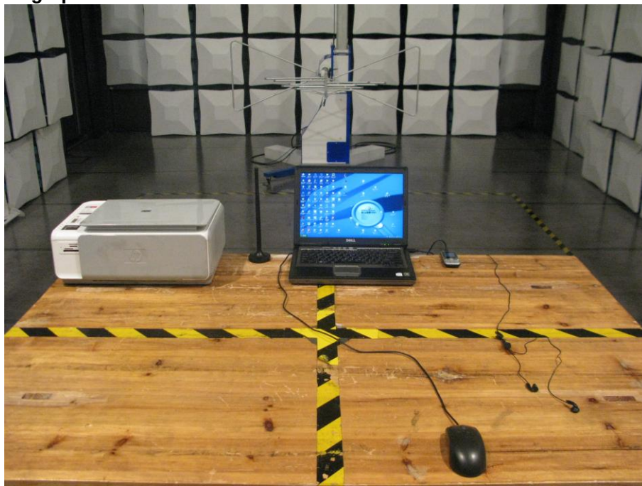
Radiated Disturbance Emissions (30MHz-1GHz)
