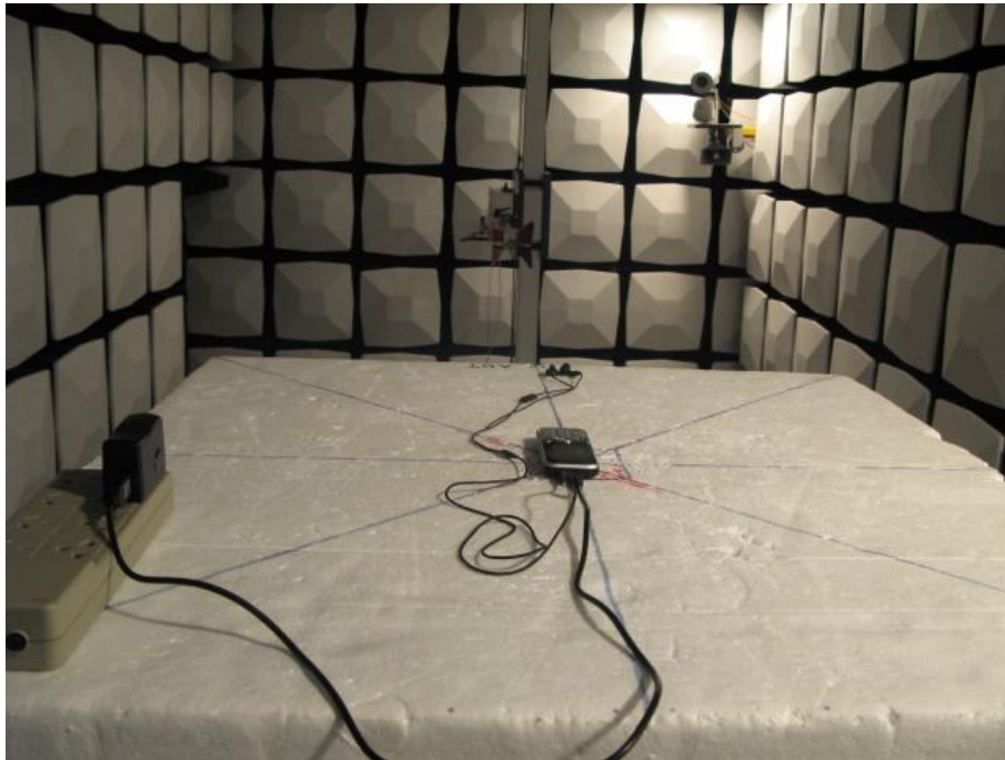
Rural Radiated Spurious Emission (2GHz to18GHz)
