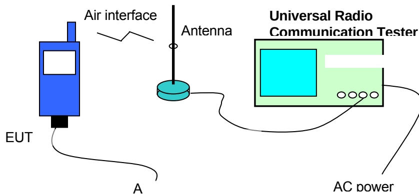
Figure 1.: Test Configuration
