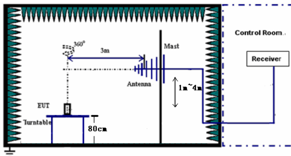
Figure 3. Test set-up
