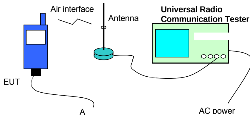
Figure 2. Test Configuration
