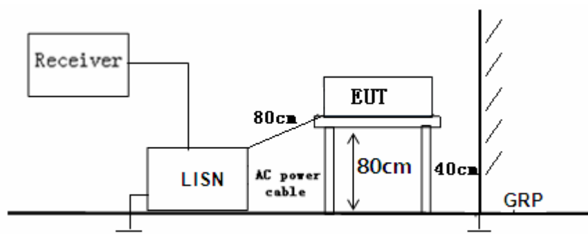
Figure 4. Test Set-up
