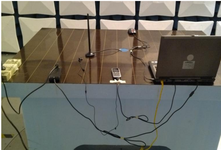
Radiated Disturbance Emissions (below 1GHz)
