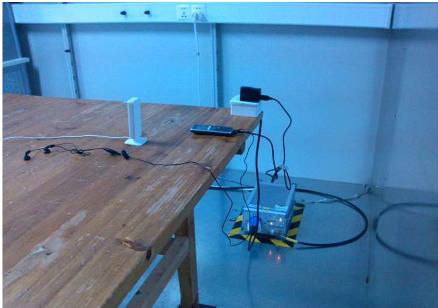
Conducted Emissions with AC Ports
