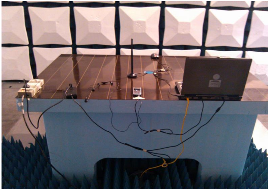
Radiated Disturbance Emissions (1GHz to18GHz)
