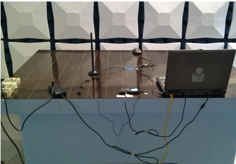
Radiated Disturbance (below 1GHz)
