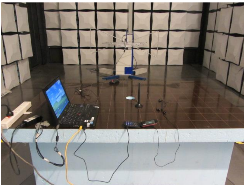
Radiated Disturbance Emissions (30MHz to 1GHz)
