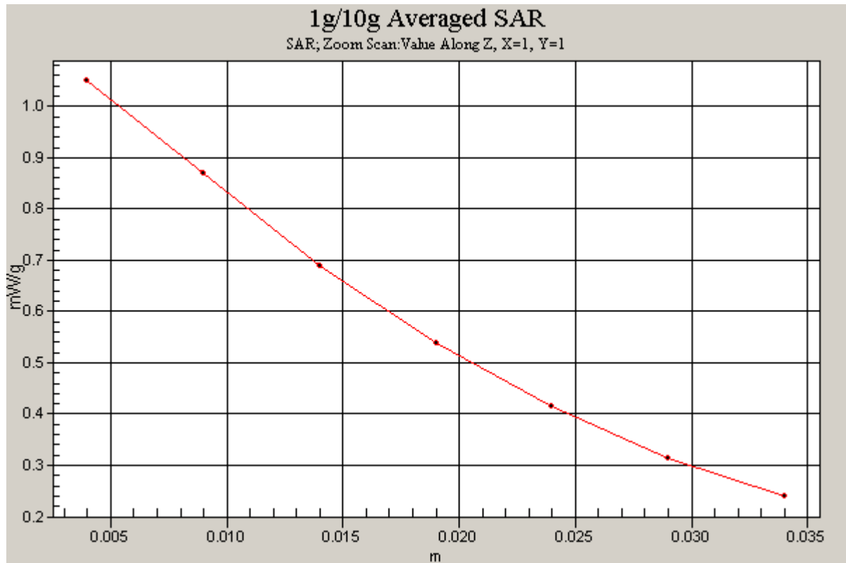
Figure 19 Right Hand Touch Cheek GSM 850 Channel 128
