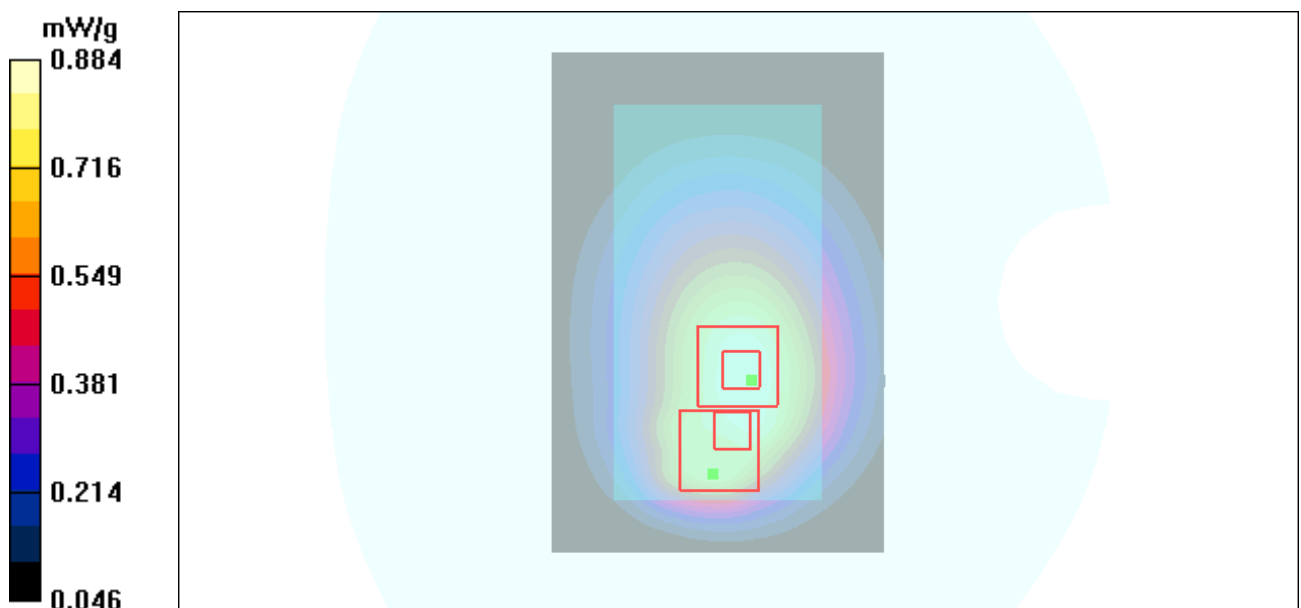
Figure 21 Body, Back Side, GSM 850 GPRS (2Txslots) Channel 251
