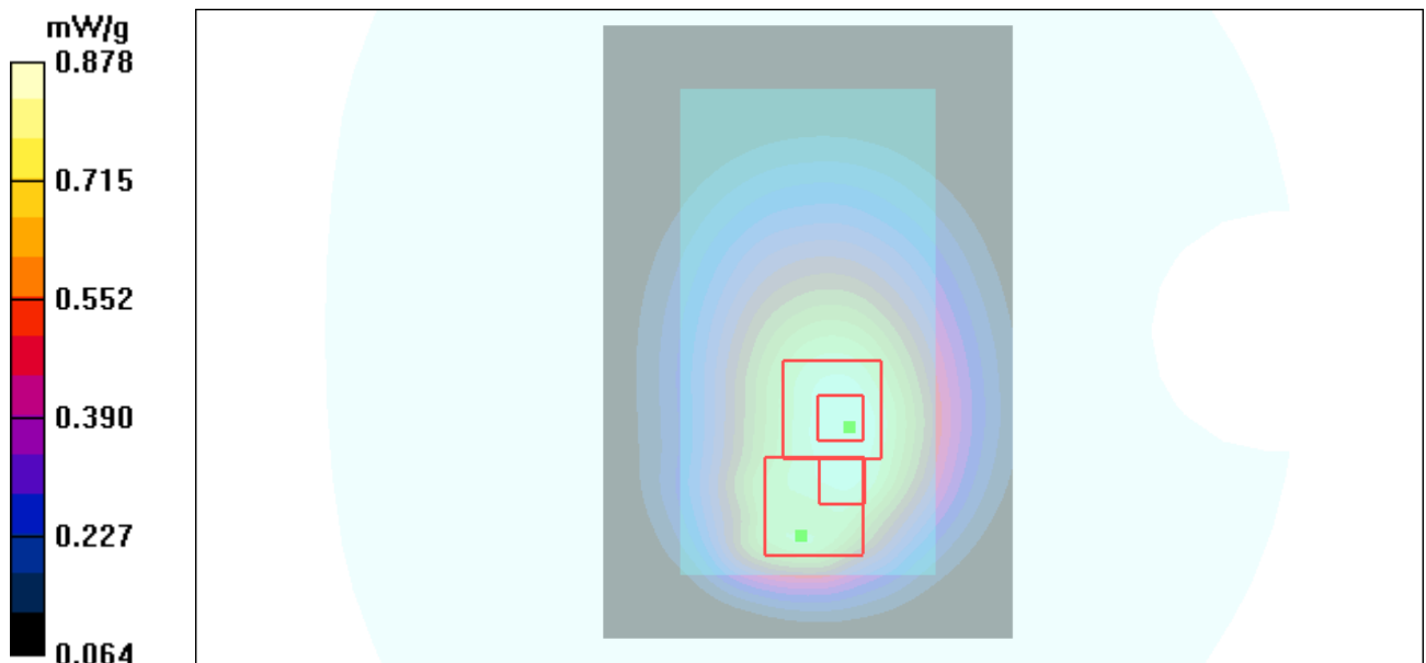
Figure 22 Body, Back Side, GSM 850 GPRS (2Txslots) Channel 190
