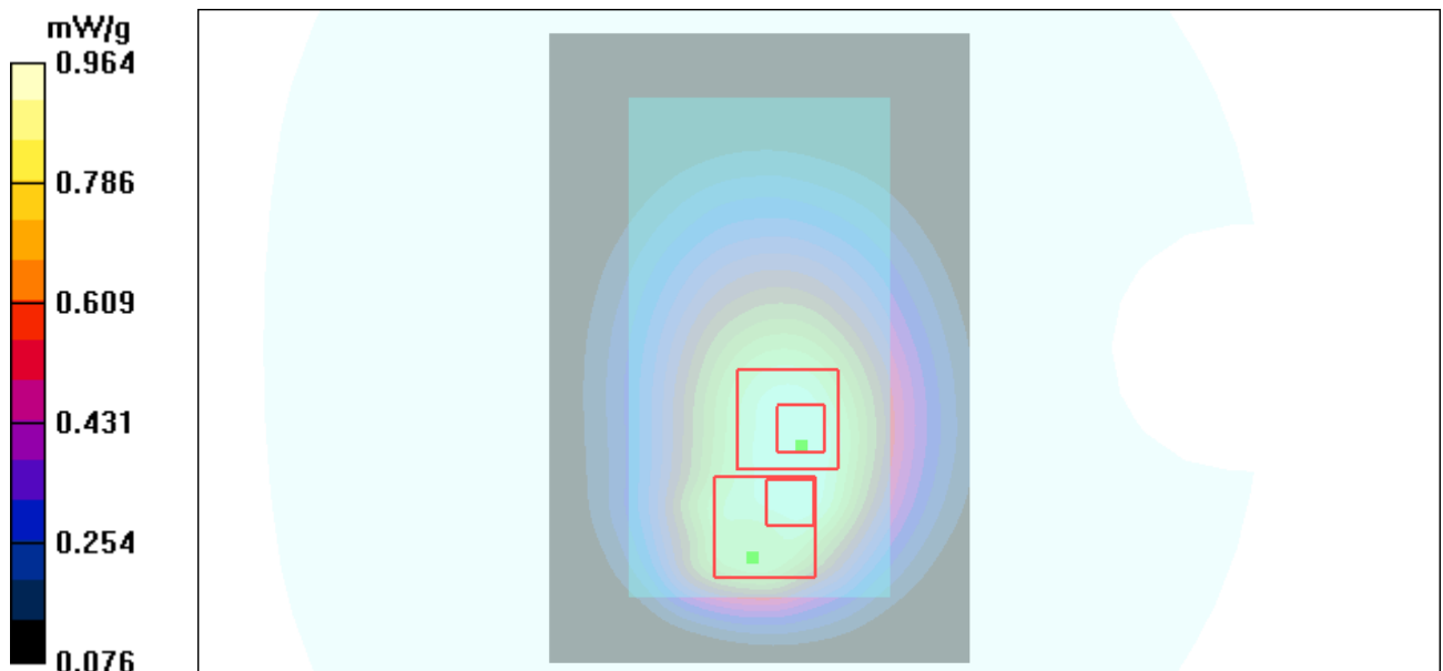
Figure 23 Body, Back Side, GSM 850 GPRS (2Txslots) Channel 128
