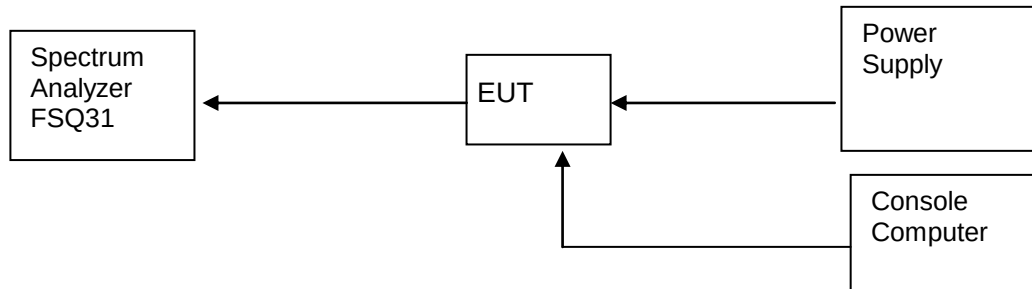
Figure 2. Test Set-up
