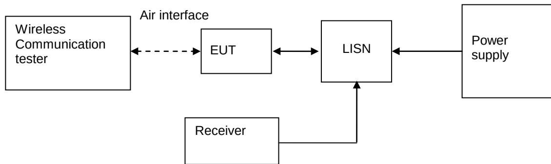
Figure 7. Test Set-up
