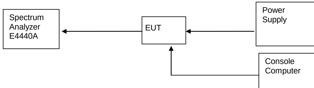
Figure 1. Test Set-up
