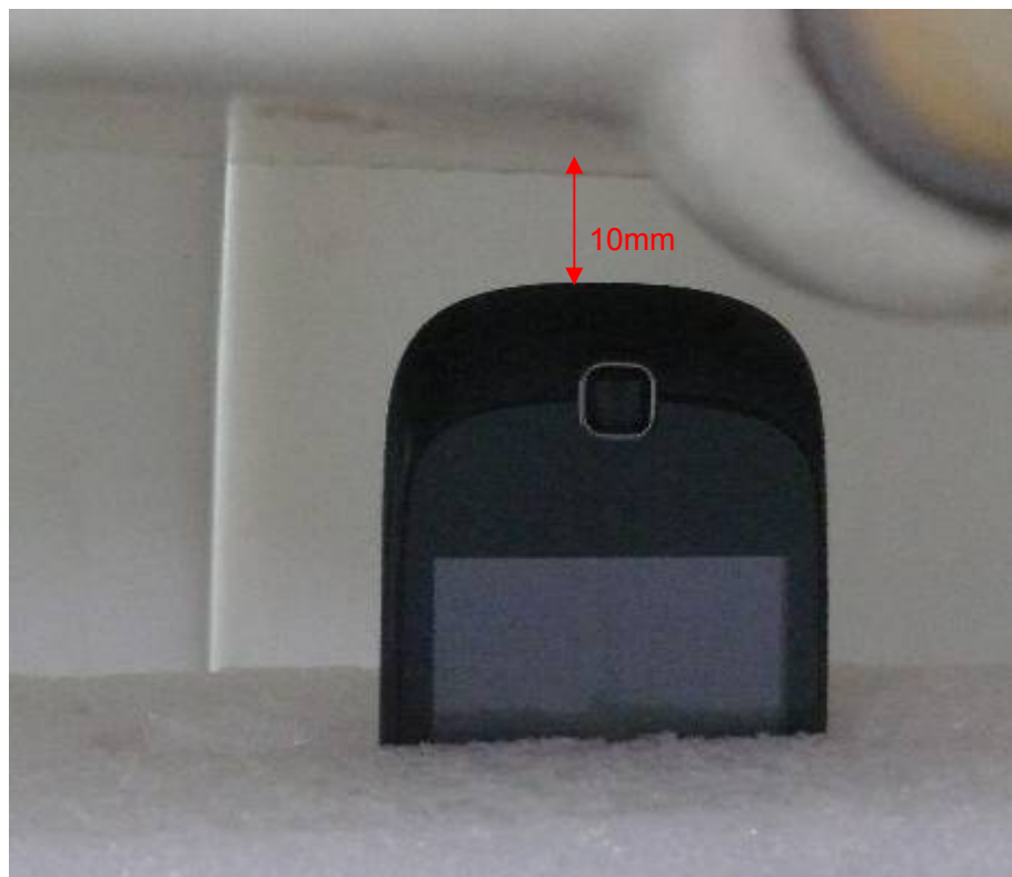
Picture 18: Bottom Edge, the distance from handset to the bottom of the Phantom is 10mm
