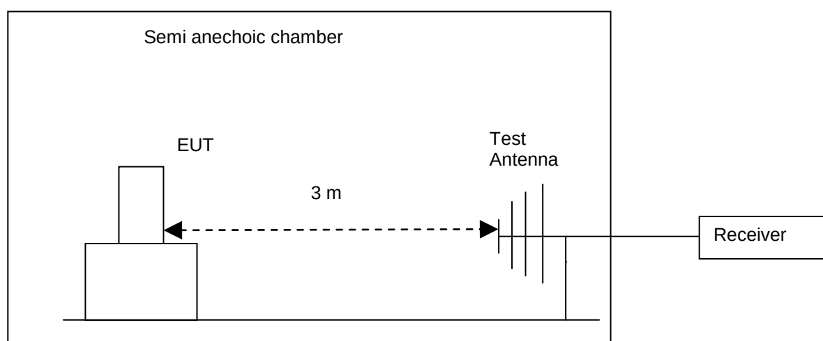
Figure 1. Test set-up
