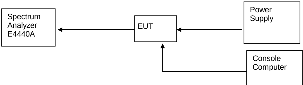
Figure 1. Test Set-up
