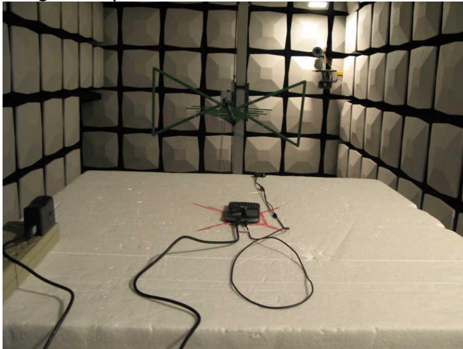
Field Strength of Spurious Emissions (below 3GHz)
