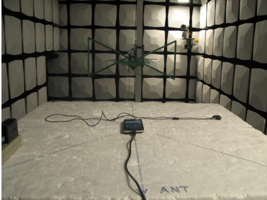
Field Strength of Spurious Emissions (below 2GHz)
