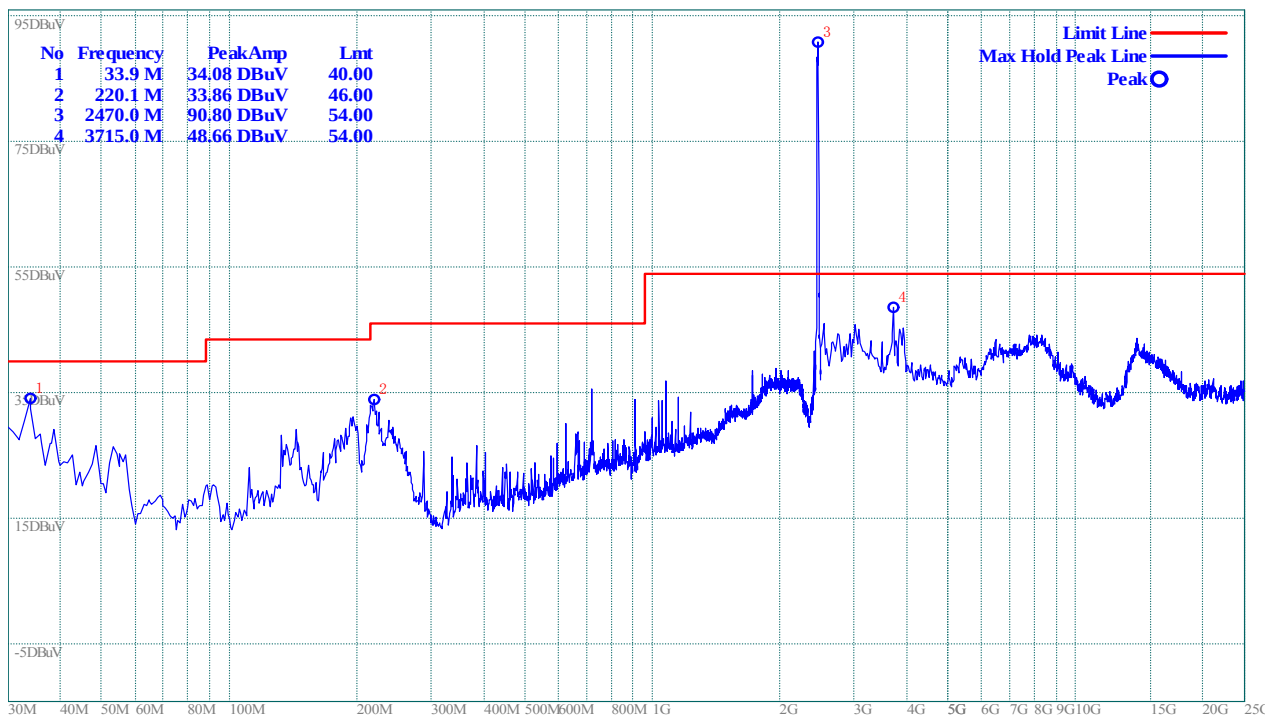
(Plot C.3: Antenna Vertical, 30MHz to 25GHz)
