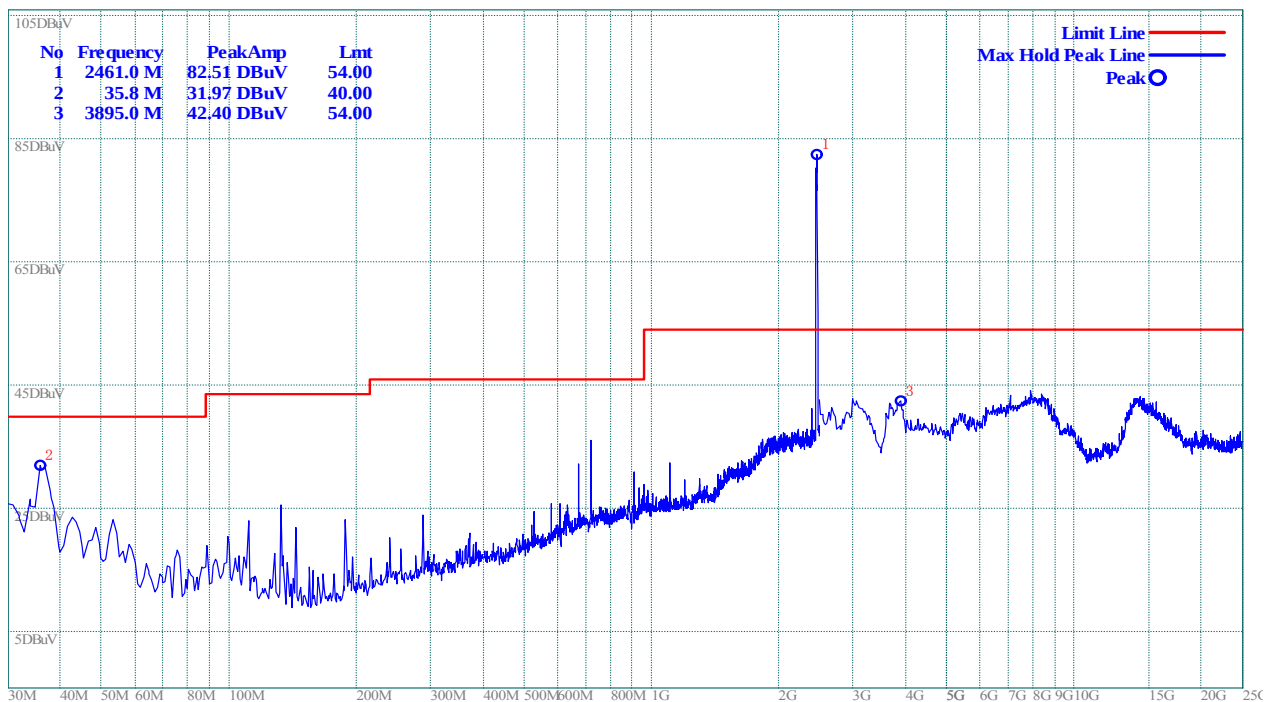
(Plot C.3: Antenna Vertical, 30MHz to 25GHz)
