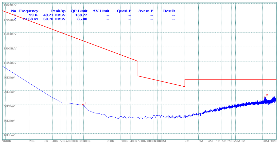
(Plot A.1: 9kHz to 30MHz)
