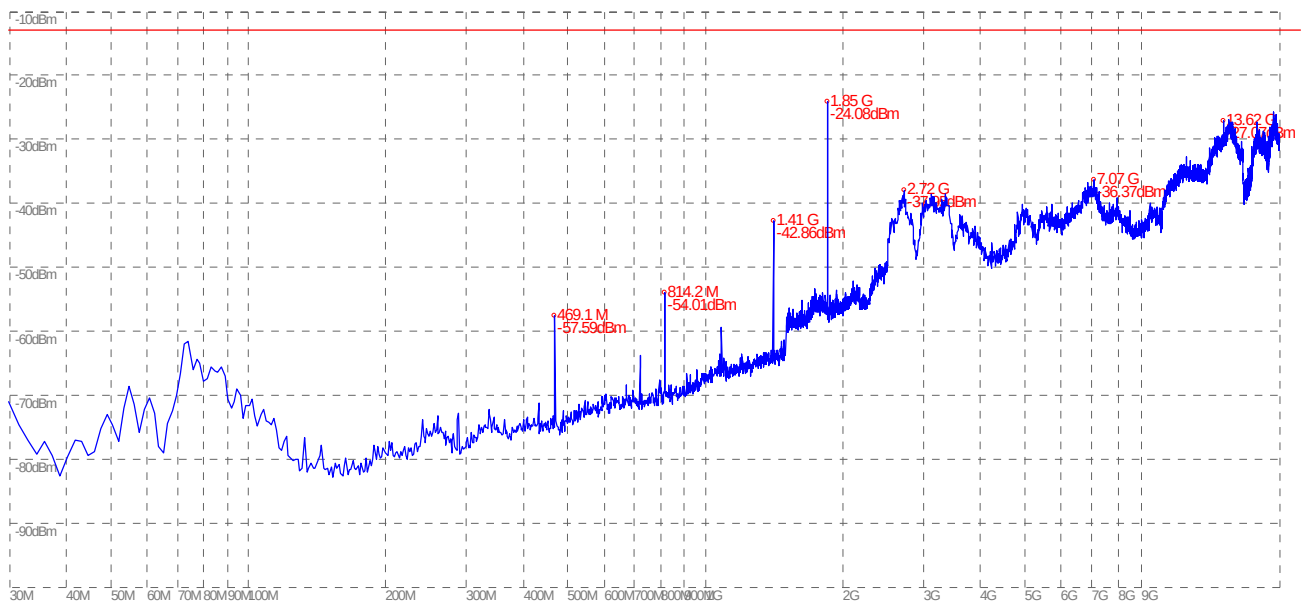
(Plot D.1: EDGE 1900MHz Channel = 512, Test Antenna Horizontal)
