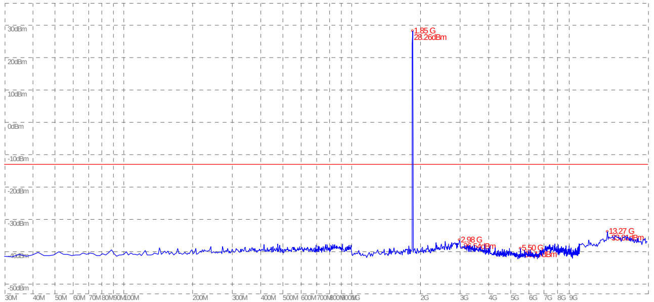
(Plot A: GSM 1900MHz Channel = 512, 30MHz to 20GHz)
