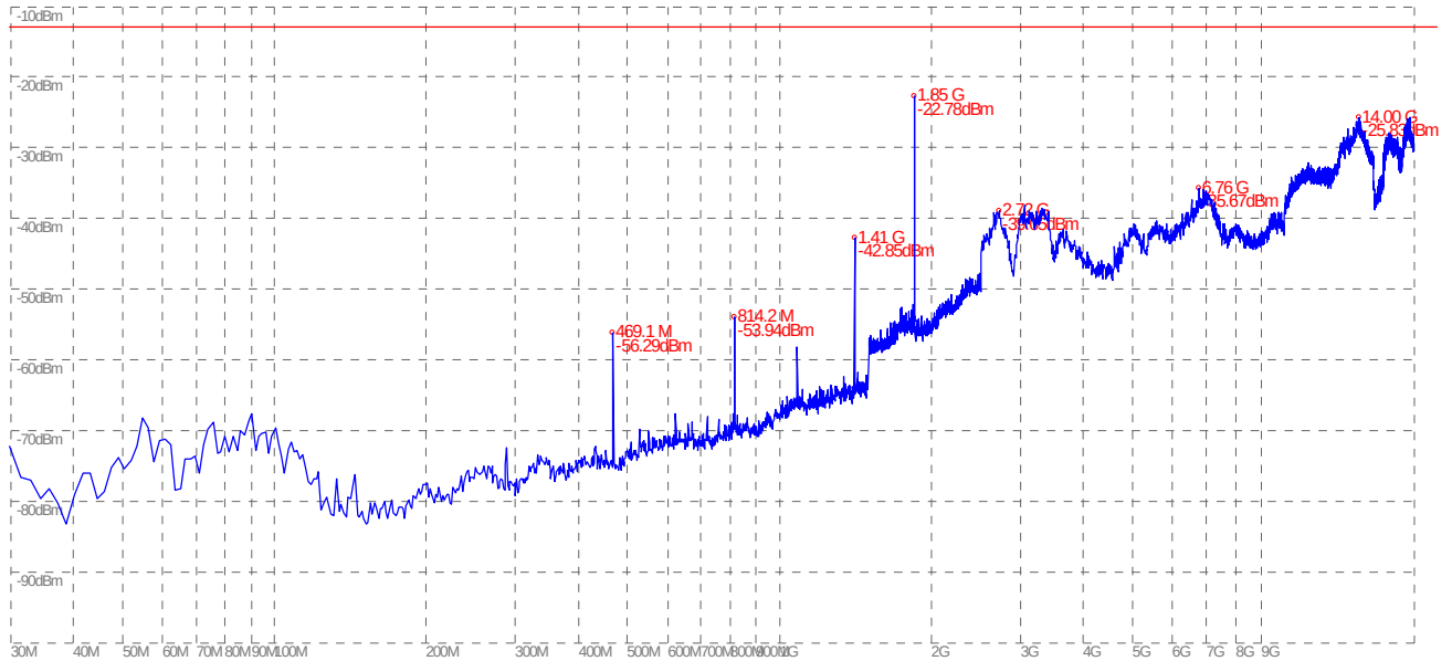
(Plot A.1: GSM 1900MHz Channel = 512, Test Antenna Horizontal)
