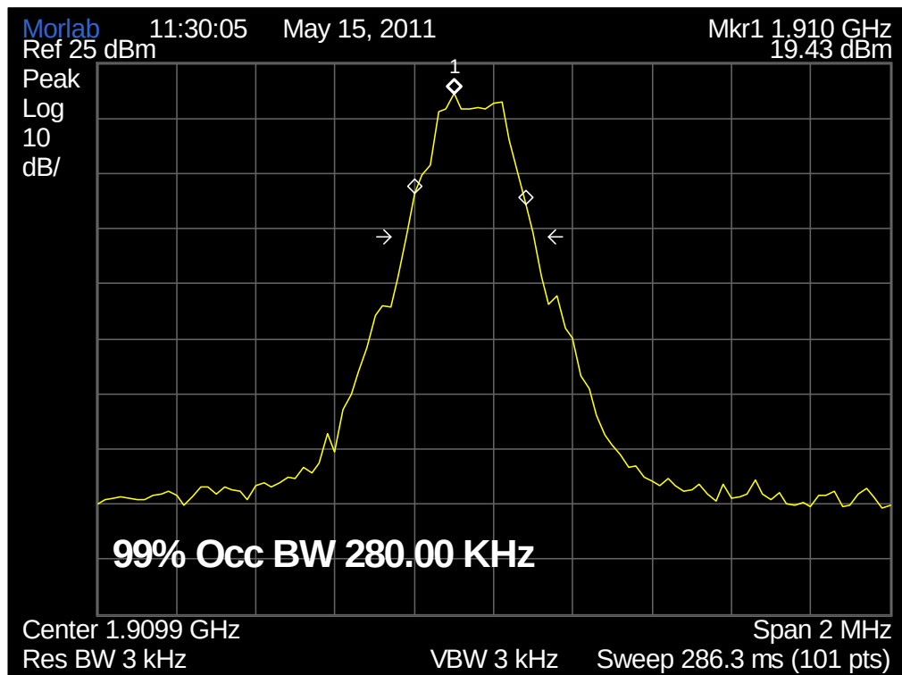
(Plot F: EDGE 1900MHz Channel = 810)
