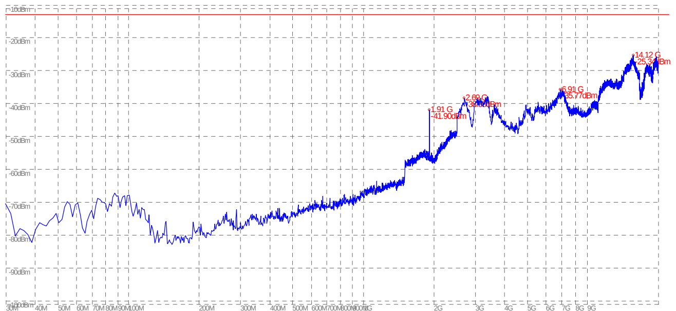
(Plot C.2: GSM 1900MHz Channel = 810, Test Antenna Vertical)
