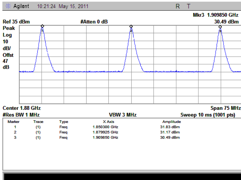
(Plot B: GPRS 1900MHz Channel = 512, 661, 810)
