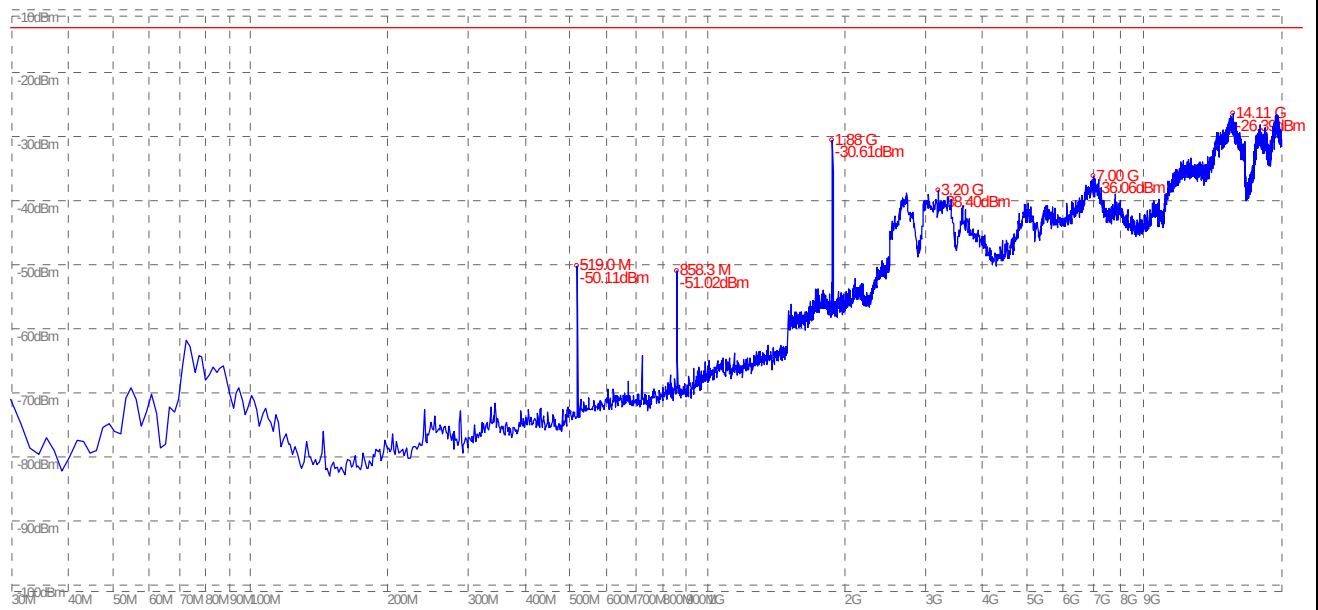
(Plot E.1: EDGE 1900MHz Channel = 661, Test Antenna Horizontal)
