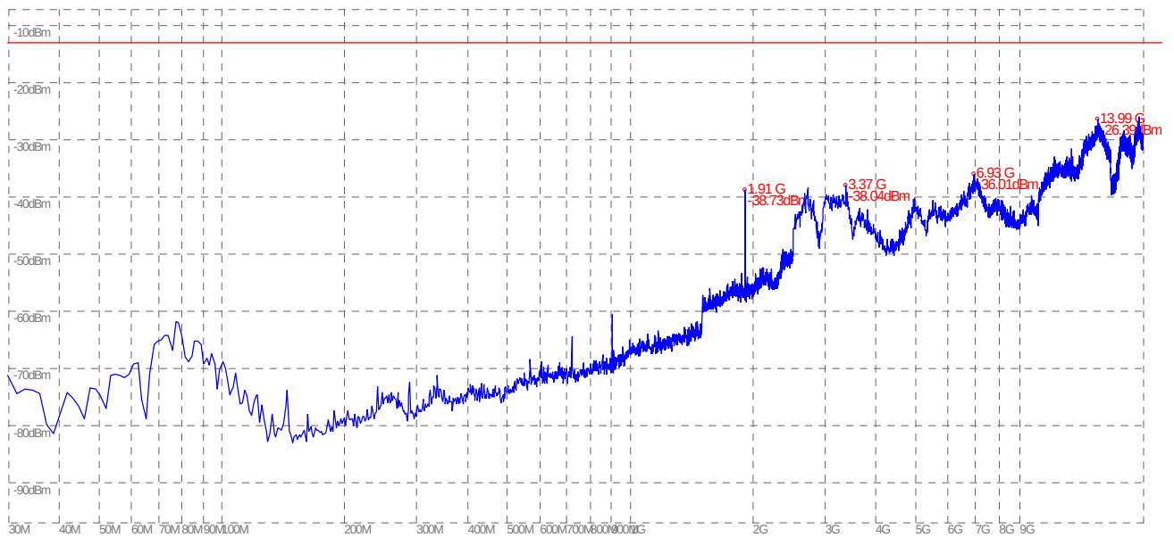
(Plot F.2: EDGE 1900MHz Channel = 810, Test Antenna Vertical)
