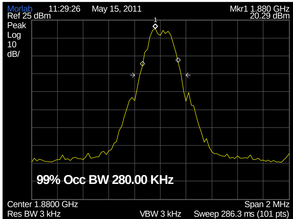
(Plot E: EDGE 1900MHz Channel = 661)
