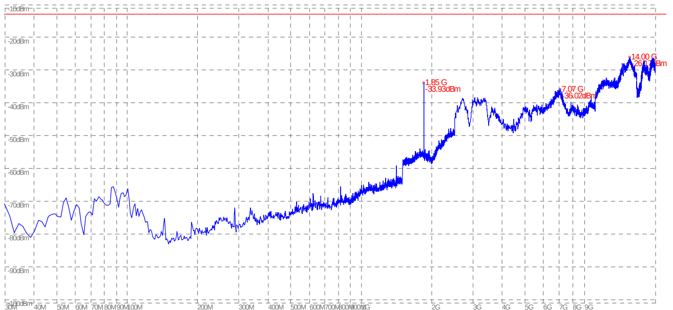
(Plot A.2: GSM 1900MHz Channel = 512, Test Antenna Vertical)
