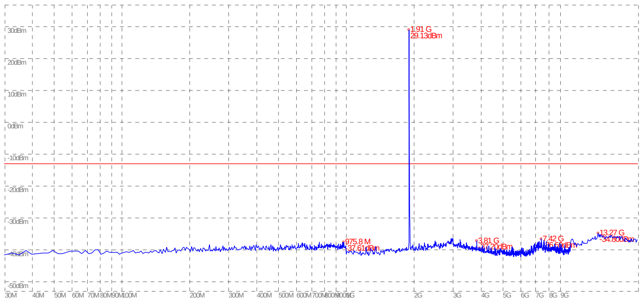
(Plot C: GSM 1900MHz Channel = 810, 30MHz to 20GHz)
