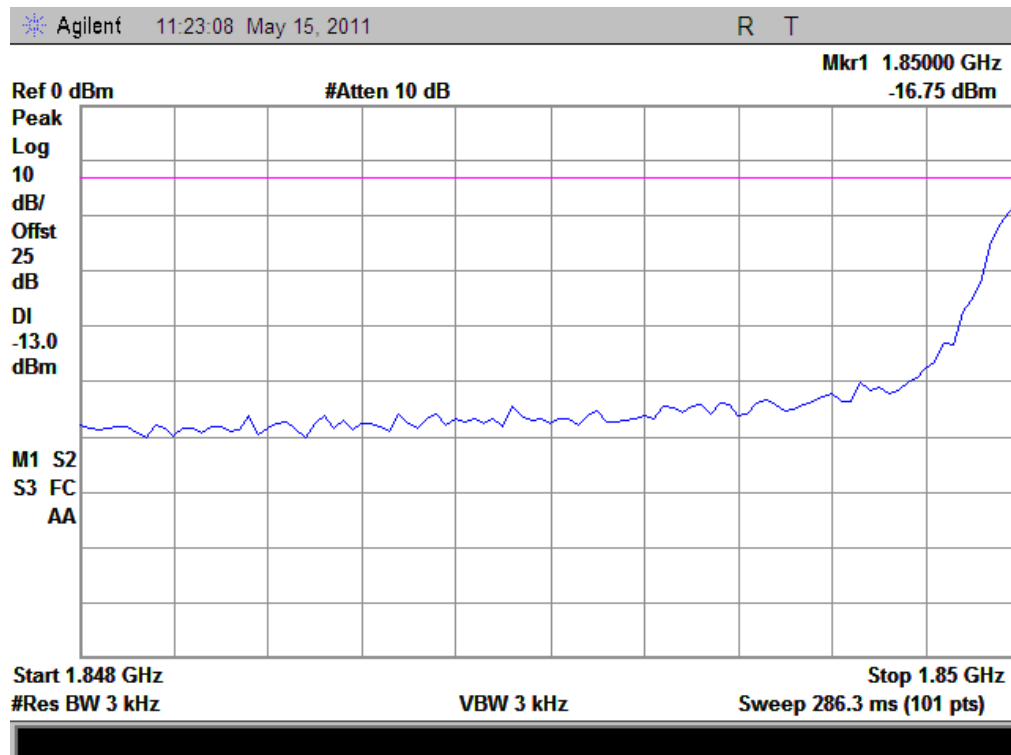
(Plot C: EDGE1900, Channel = 512)
