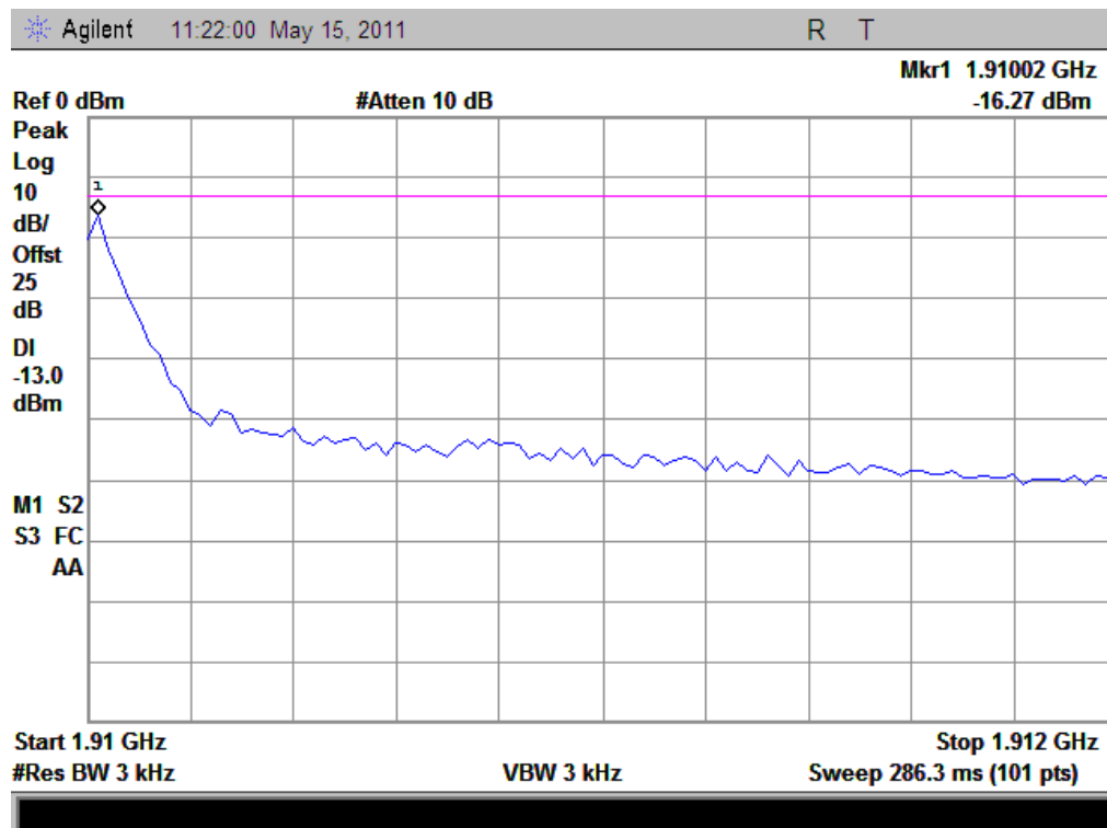
(Plot D: EDGE1900, Channel = 810)
