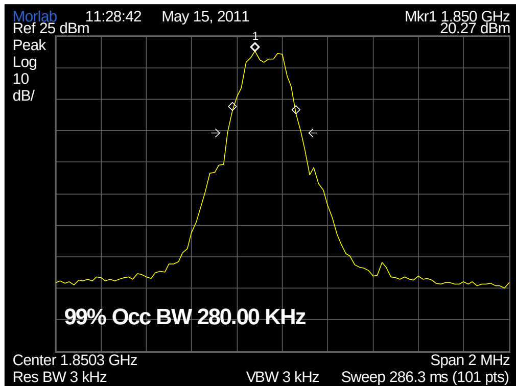
(Plot D: EDGE 1900MHz Channel = 512)
