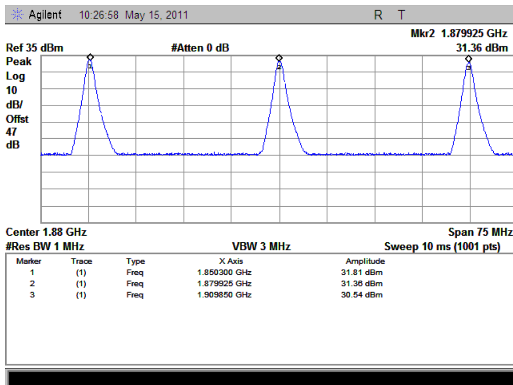
(Plot C: EDGE 1900MHz Channel = 512, 661, 810)
