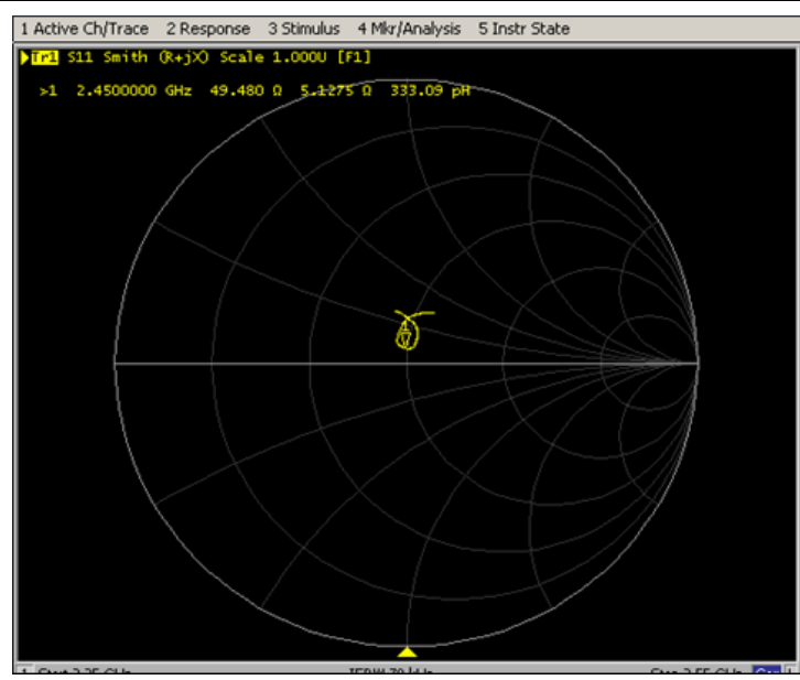
Impedance Test-Body
