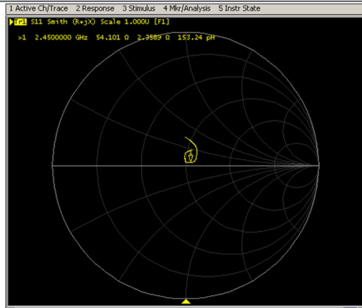
Impedance Test-Body
