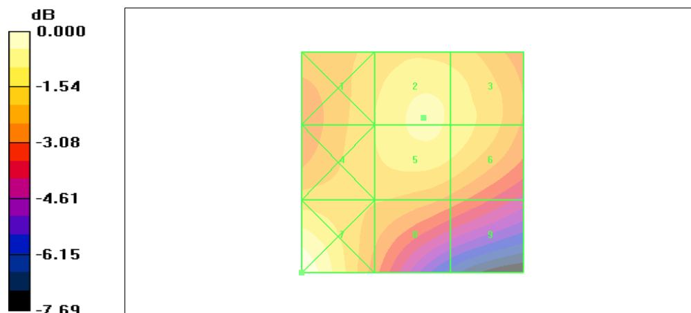
Figure 32 HAC RF H-Field WCDMA Band II Channel 9262
