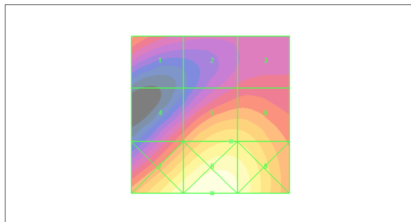
Figure 37 HAC RF E-Field WCDMA Band IV Channel 1413
