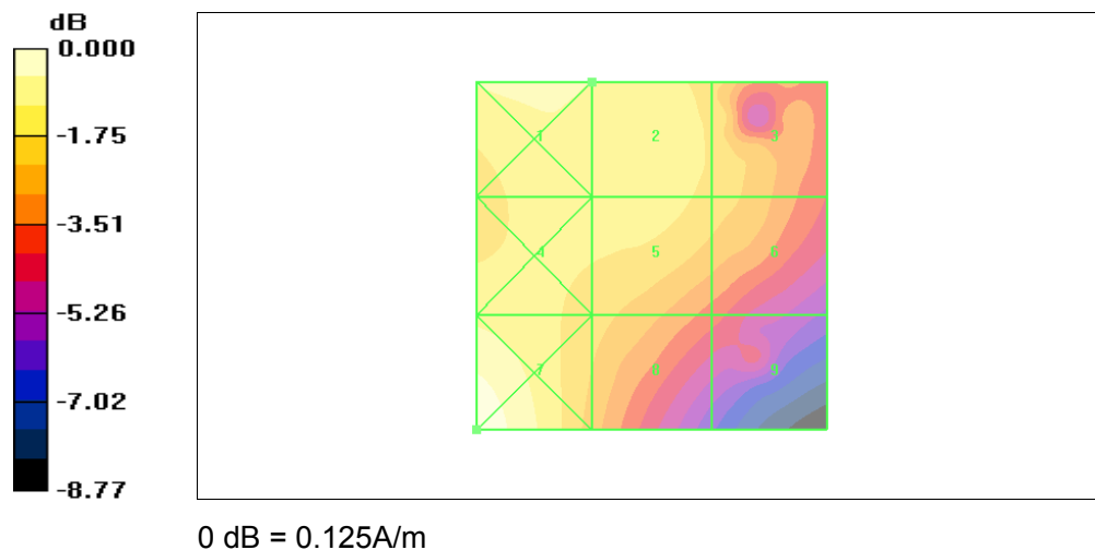
Figure 47 HAC RF H-Field WCDMA Band IV HSDPA Channel 1312
