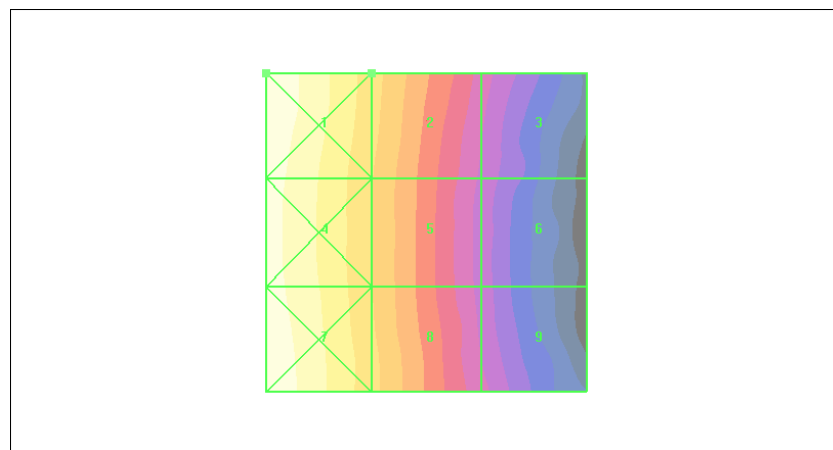
Figure 54 HAC RF H-Field WCDMA Band V Channel 4233
