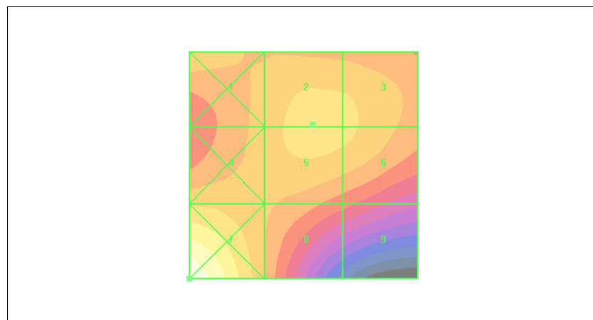
Figure 31 HAC RF H-Field WCDMA Band II Channel 9400
