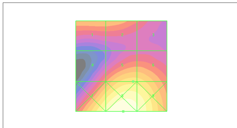
Figure 25 HAC RF E-Field WCDMA Band II Channel 9400
