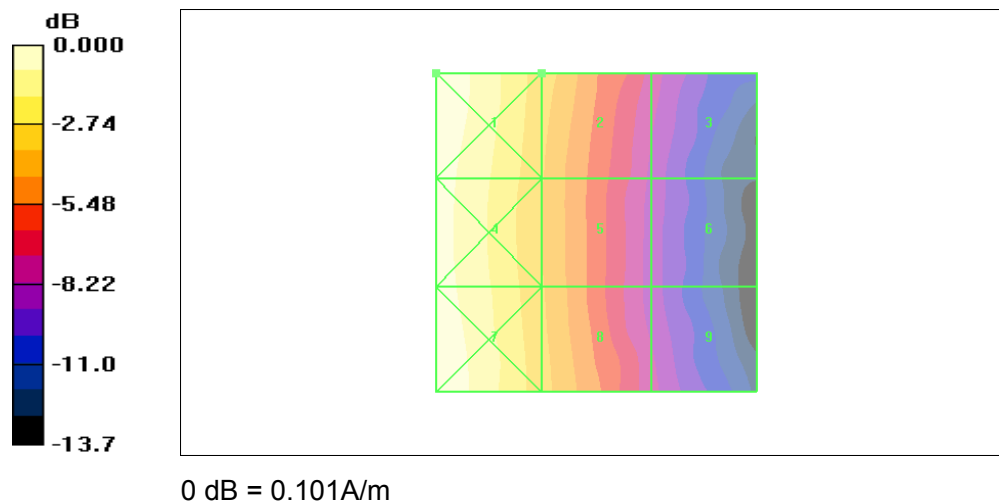
Figure 58 HAC RF H-Field WCDMA Band V HSDPA Channel 4183
