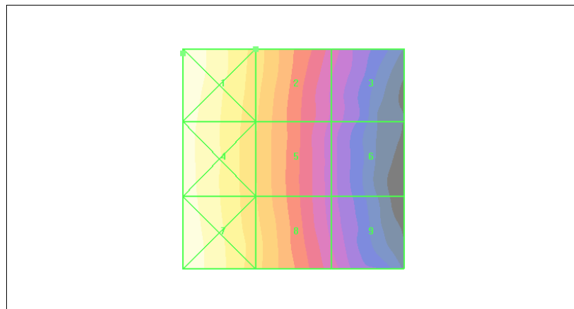
Figure 16 HAC RF H-Field GSM 850 Channel 190
