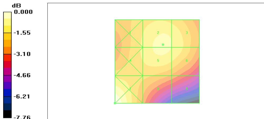
Figure 35 HAC RF H-Field WCDMA Band II HSDPA Channel 9262
