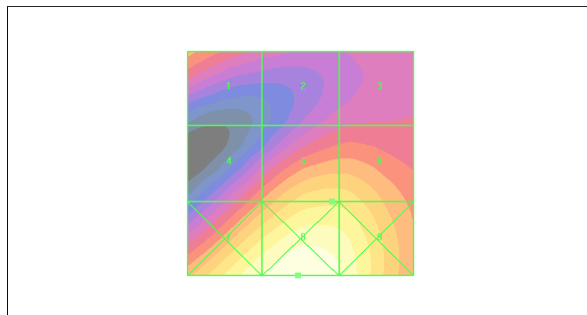
Figure 36 HAC RF E-Field WCDMA Band IV Channel 1513
