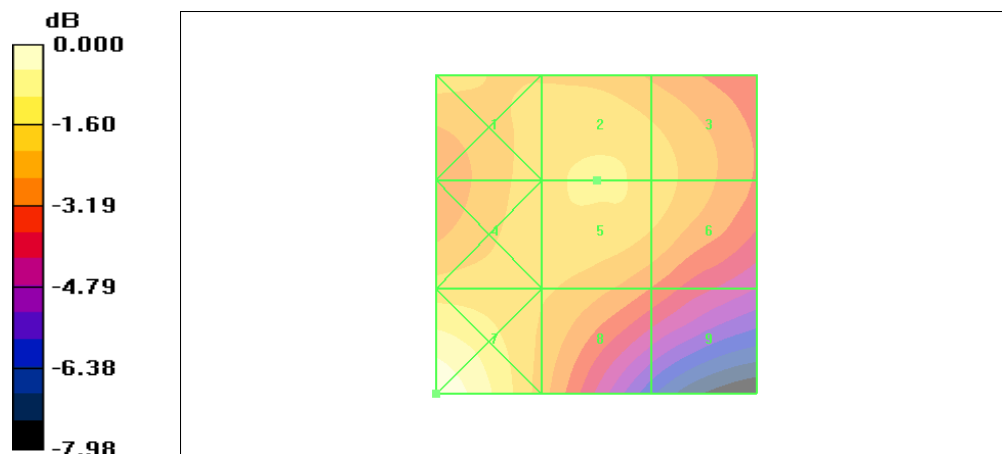
Figure 33 HAC RF H-Field WCDMA Band II HSDPA Channel 9538
