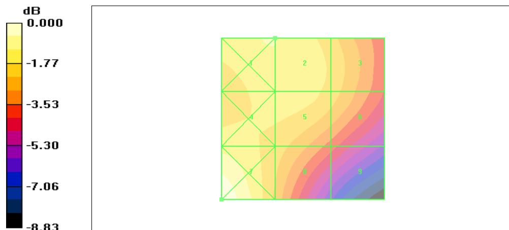
Figure 44 HAC RF H-Field WCDMA Band IV Channel 1312
