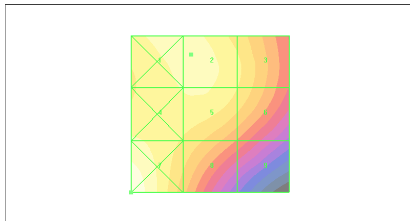
Figure 45 HAC RF H-Field WCDMA Band IV HSDPA Channel 1513
