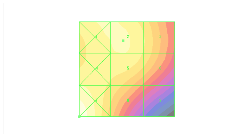
Figure 42 HAC RF H-Field WCDMA Band IV Channel 1513
