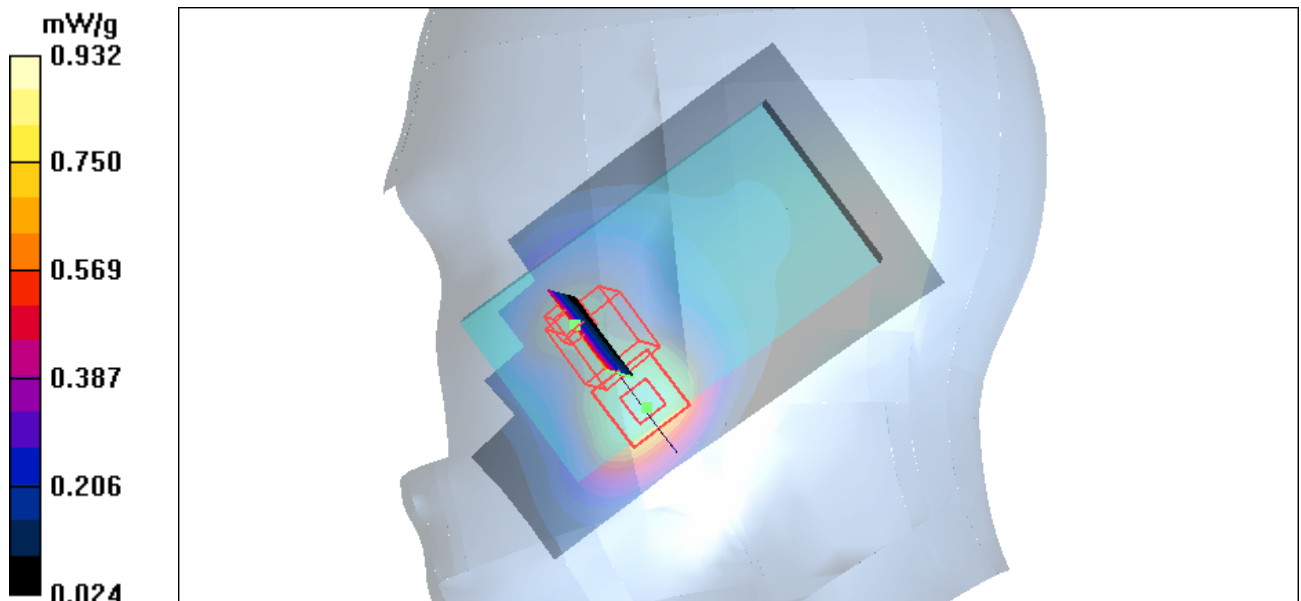
Figure 49 Right Hand Touch Cheek WCDMA Band II Channel 9262
