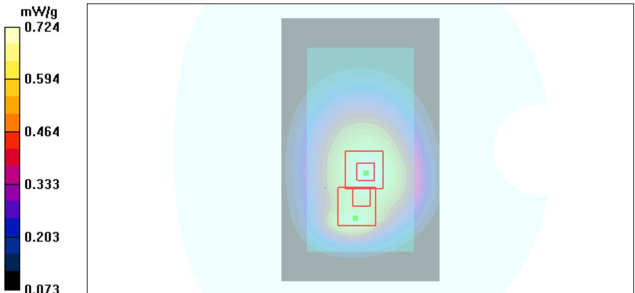
Figure 21 Body, Back Side, GSM 850 GPRS (1Txslot) Channel 128
