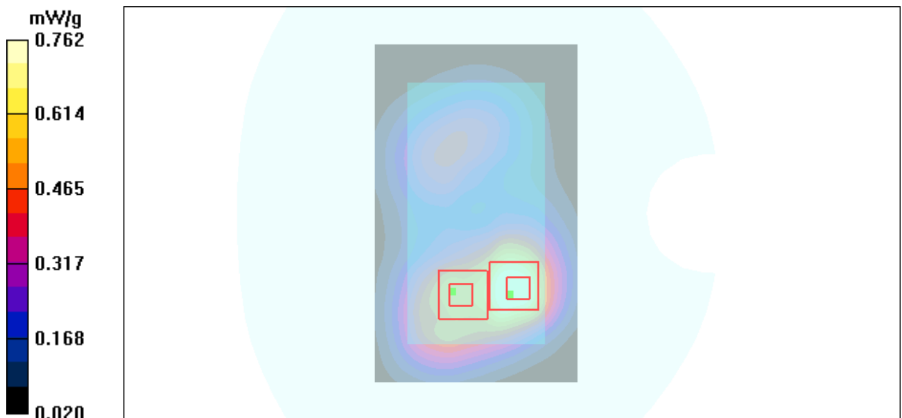
Figure 51 Body, Back Side, WCDMA Band II Channel 9538
