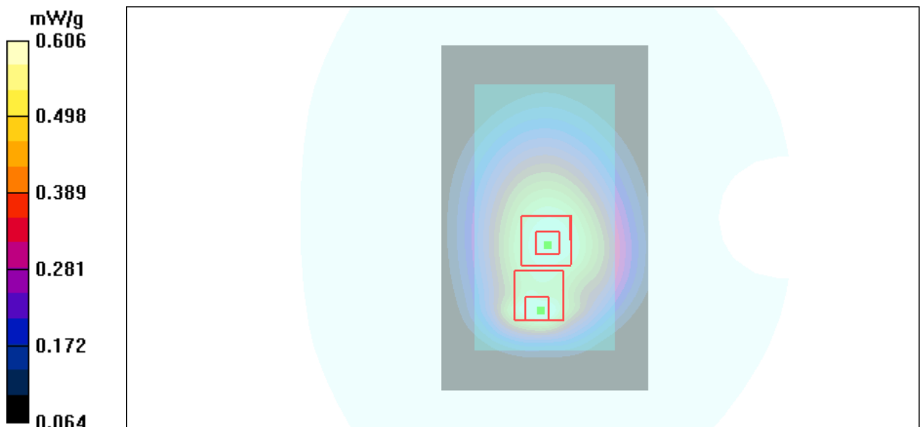
Figure 84 Body with Earphone, Back Side, WCDMA Band V Channel 4183
