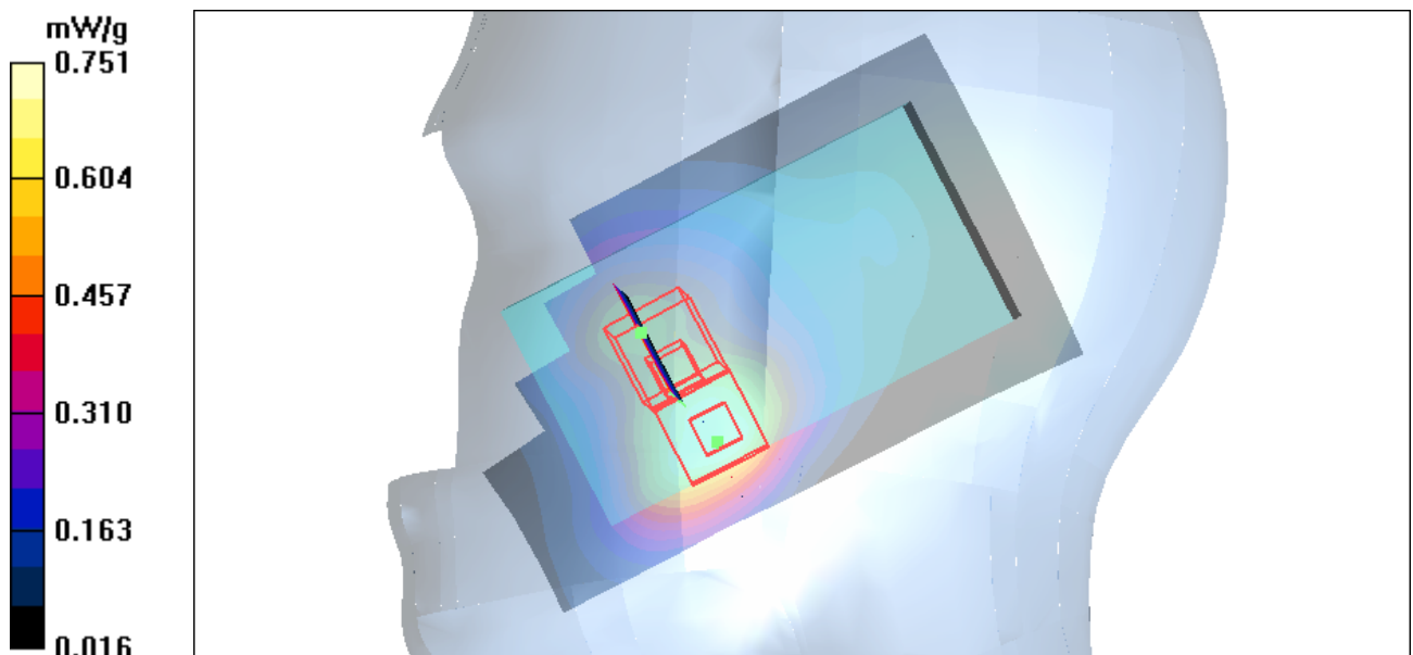
Figure 65 Right Hand Touch Cheek WCDMA Band IV Channel 1413
