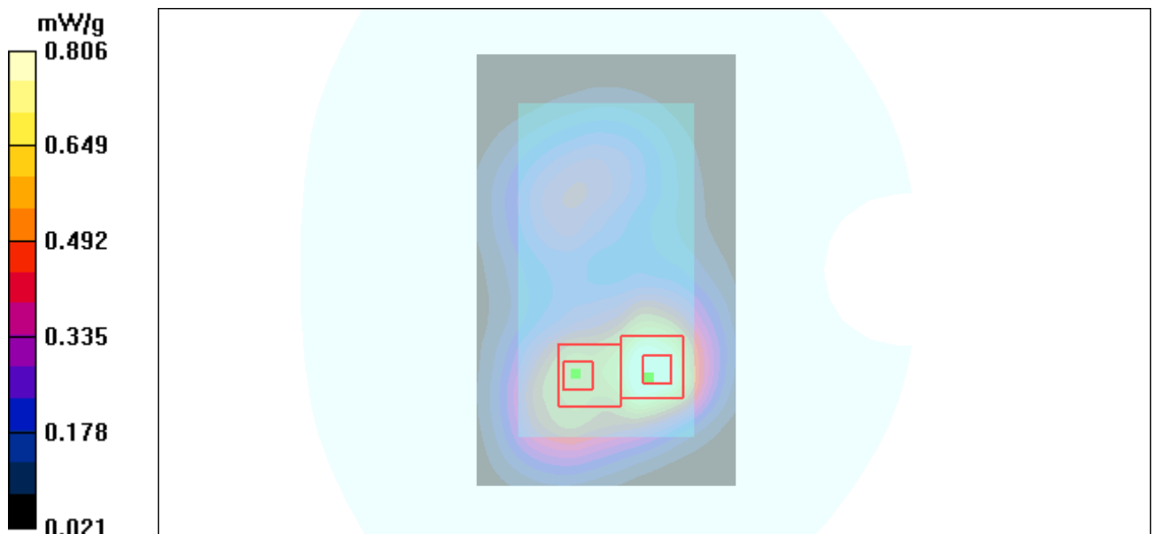
Figure 53 Body, Back Side, WCDMA Band II Channel 9262
