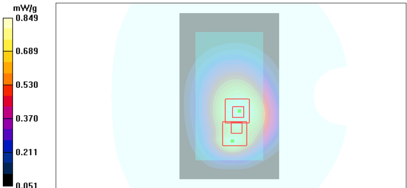
Figure 20 Body, Back Side, GSM 850 GPRS (1Txslot) Channel 190
