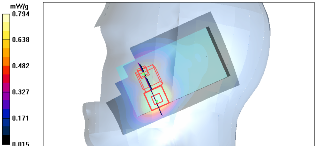
Figure 47 Right Hand Touch Cheek WCDMA Band II Channel 9538
