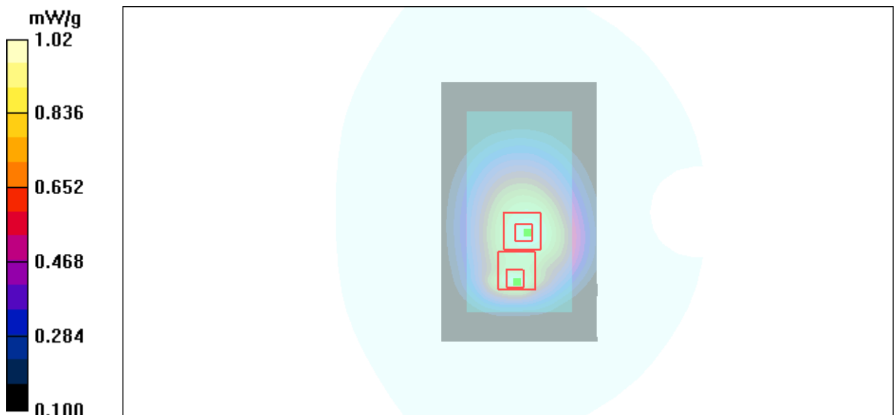
Figure 30 Body, Back Side, GSM 850 EGPRS (2Txslots) Channel 190
