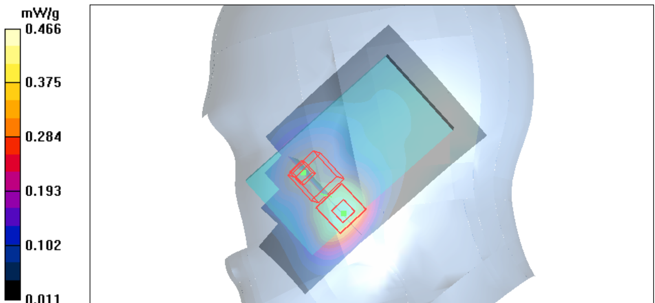
Figure 33 Right Hand Touch Cheek GSM 1900 Channel 661
