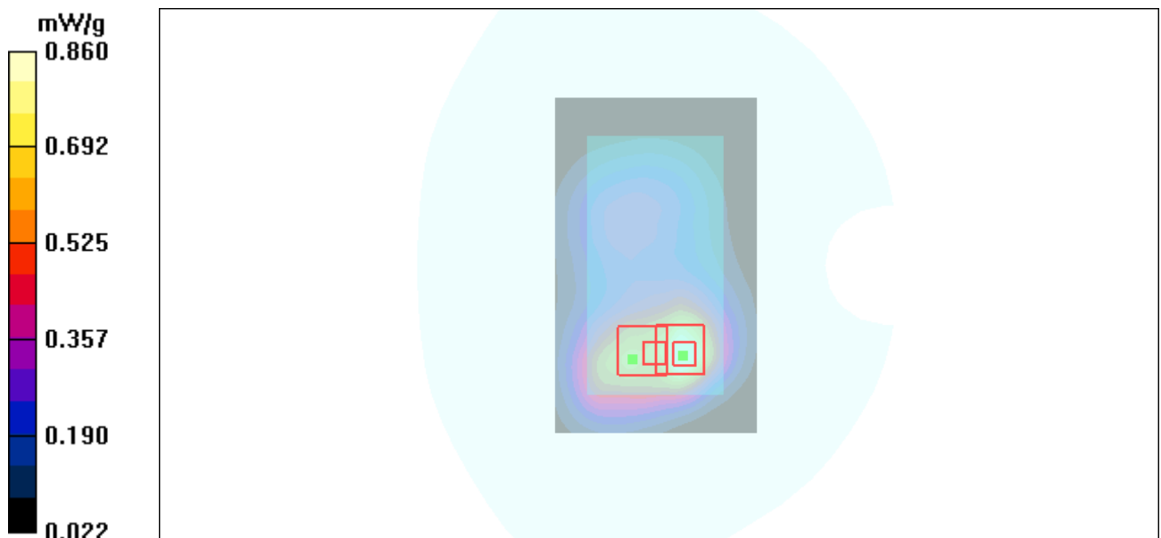
Figure 67 Body, Back Side, WCDMA Band IV Channel 1413
