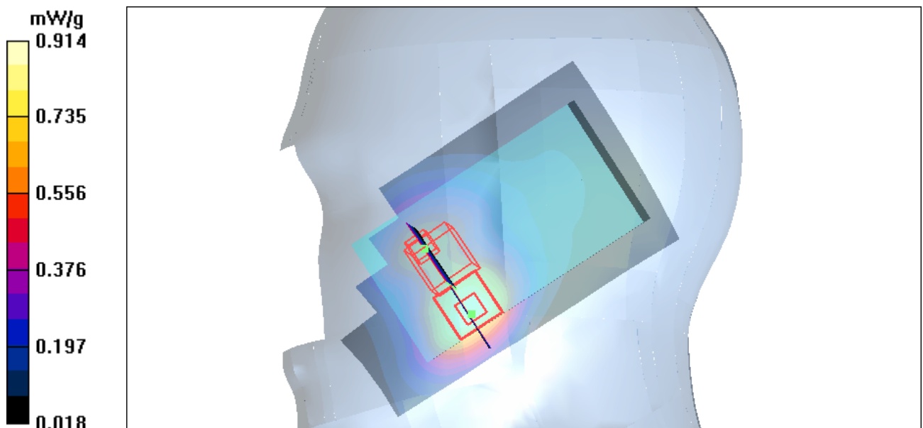
Figure 48 Right Hand Touch Cheek WCDMA Band II Channel 9400
