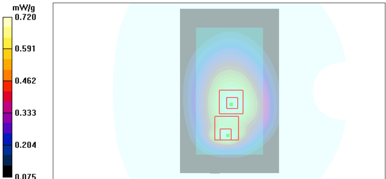
Figure 29 Body with Earphone, Back Side, GSM 850 Channel 190
