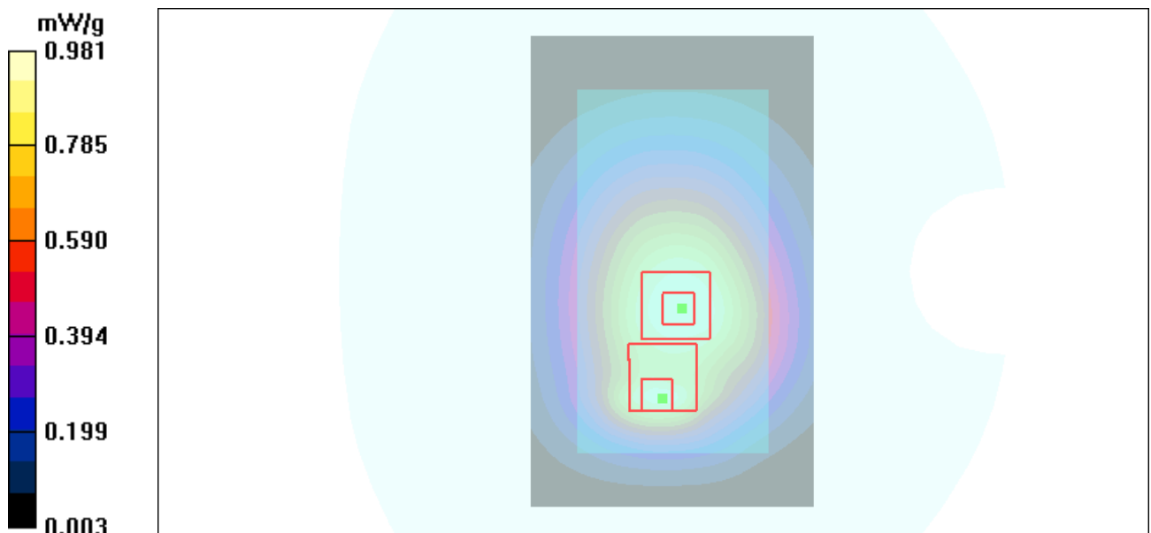
Figure 22 Body, Back Side, GSM 850 GPRS (2Txslots) Channel 251
