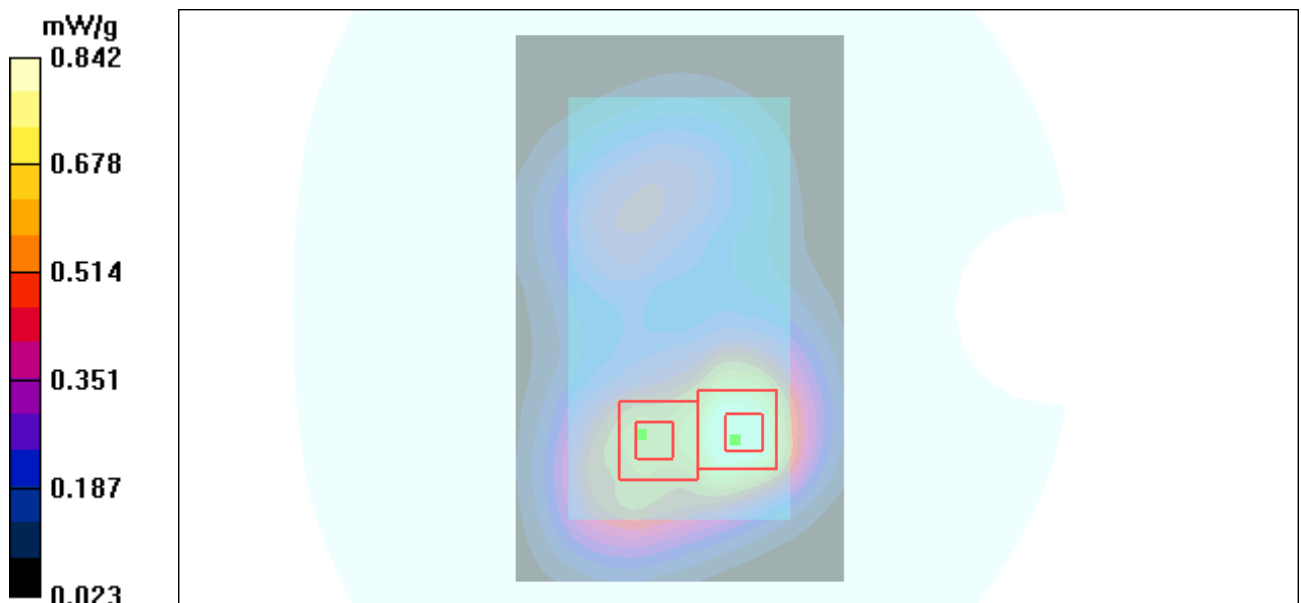
Figure 52 Body, Back Side, WCDMA Band II Channel 9400
