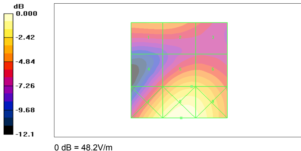
Figure 28 HAC RF E-Field WCDMA Band II HSDPA Channel 9400
