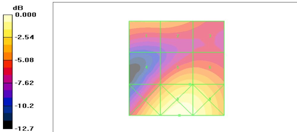
Figure 27 HAC RF E-Field WCDMA Band II HSDPA Channel 9538
