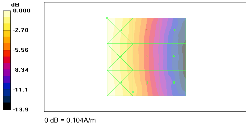
Figure 59 HAC RF H-Field WCDMA Band V HSDPA Channel 4132
