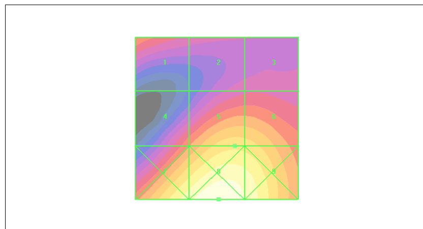
Figure 41 HAC RF E-Field WCDMA Band IV HSDPA Channel 1312
