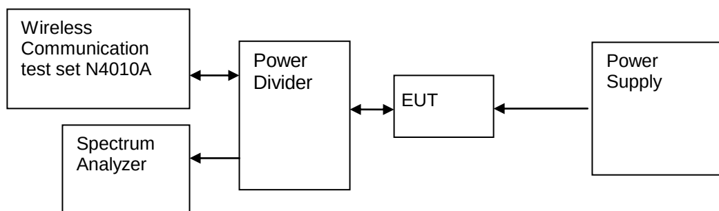
Figure 2. Test Set-up
