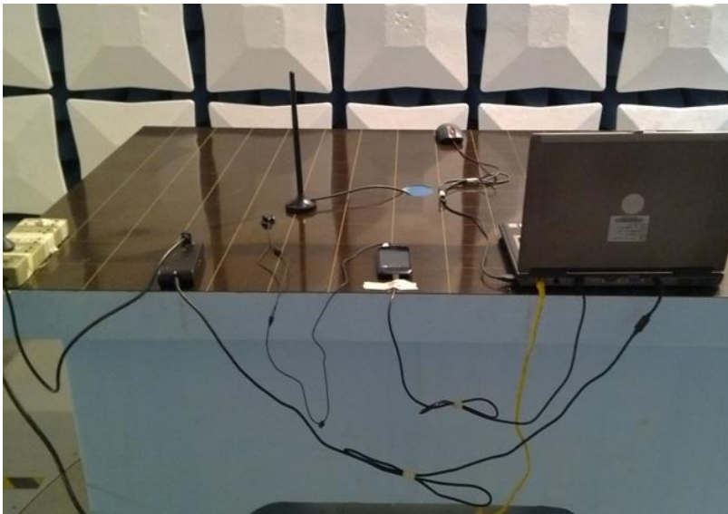
Radiated Emission (below 1GHz)
