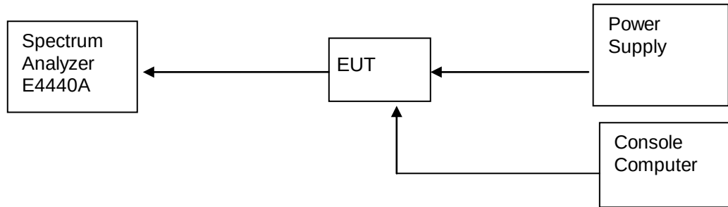
Figure 3. Test Set-up
