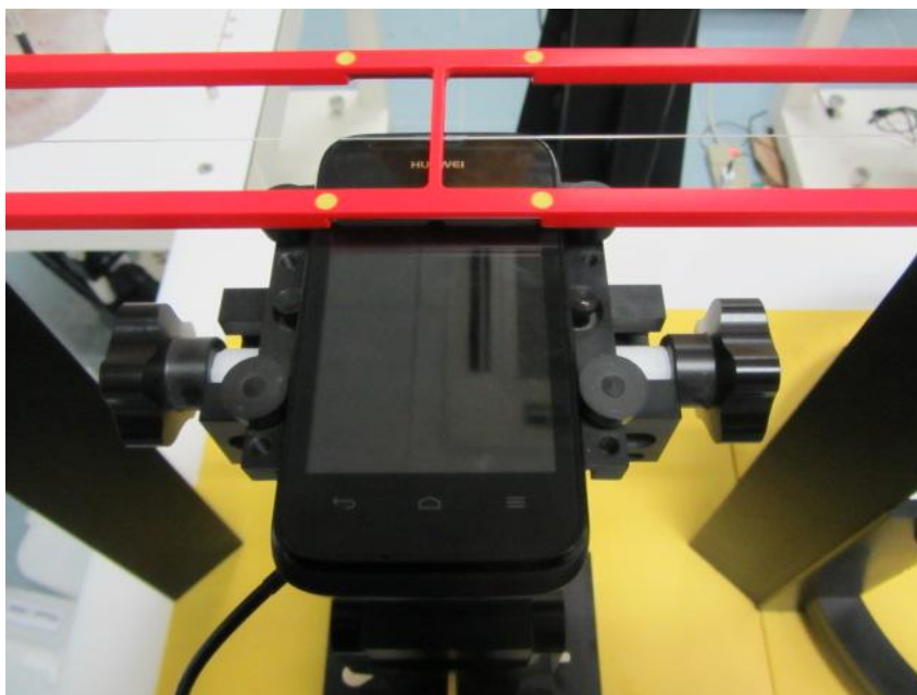
HAC T-coil test photo
