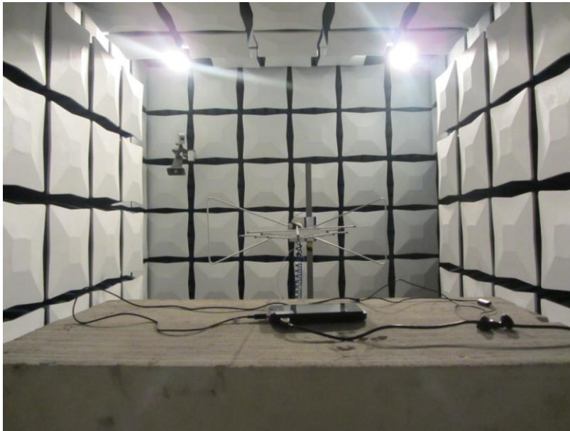
Radiated Spurious Emission (30MHz-1GHz)
