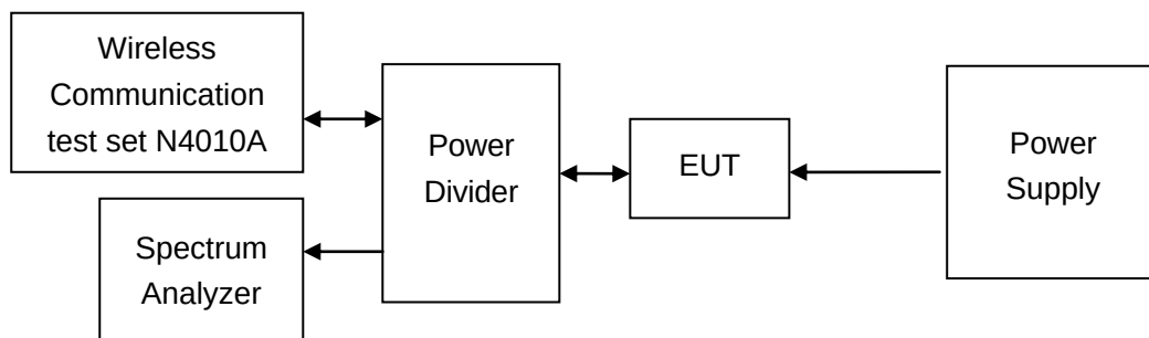
Figure 7. Test Set-up
