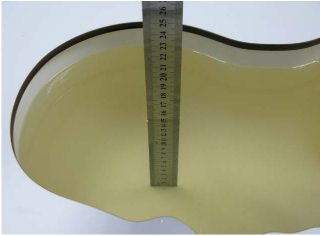
Photo 17: HSL1900MHz depth (15.2cm)
