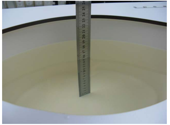
Photo 18: MSL1900MHz depth (15.1cm)
