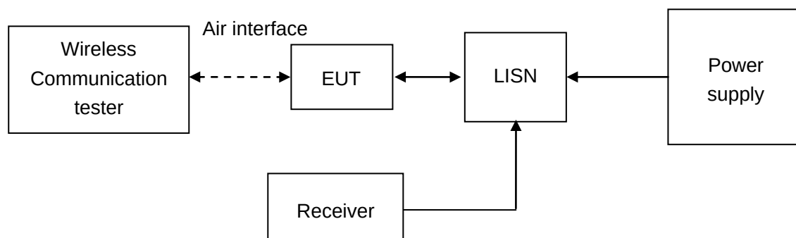
Figure 9. Test Set-up
