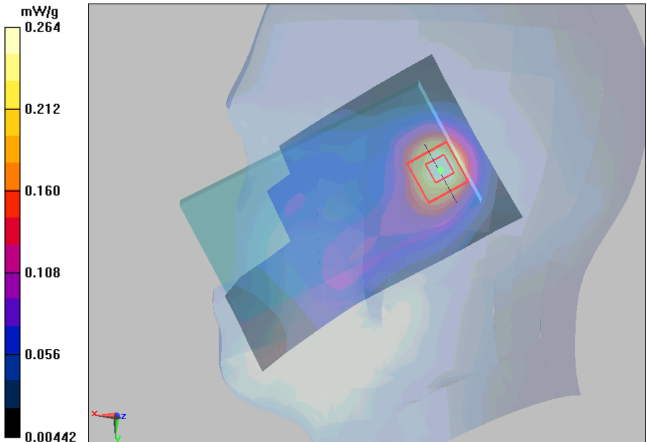
Figure 56 Right Hand Tilt 15°WCDMA Band IV Channel 1413
