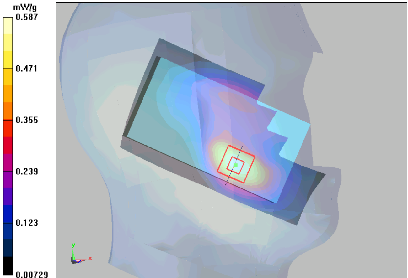
Figure 53 Left Hand Touch Cheek WCDMA Band IV Channel 1413
