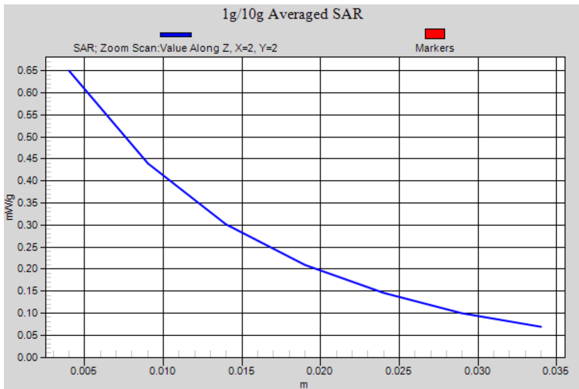
Figure 55 Right Hand Touch Cheek WCDMA Band IV Channel 1413
