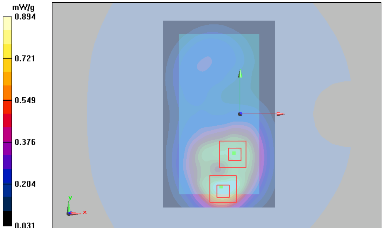
Figure 57 Body, Back Side, WCDMA Band IV Channel 1513
