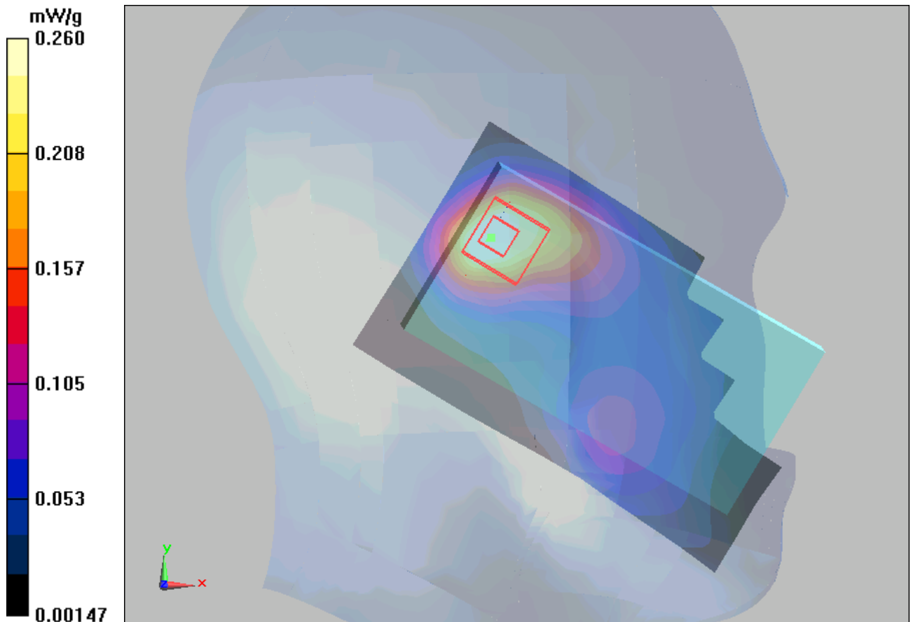
Figure 54 Left Hand Tilt 15°WCDMA Band IV Channel 1413
