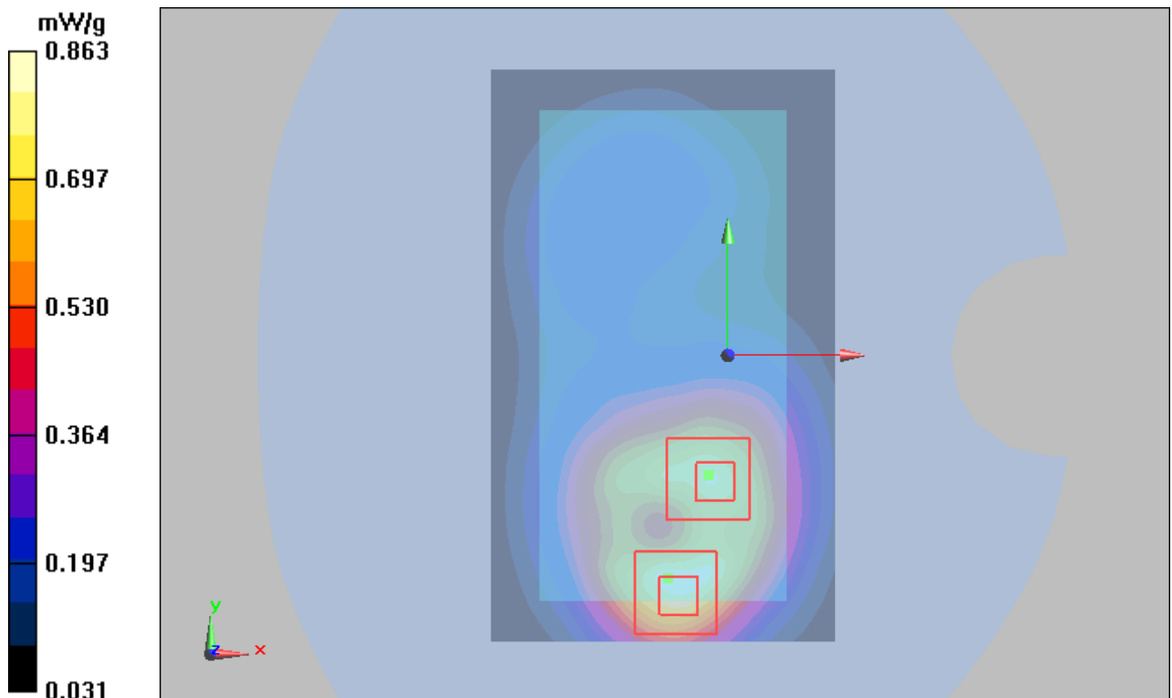
Figure 59 Body, Back Side, WCDMA Band IV Channel 1312
