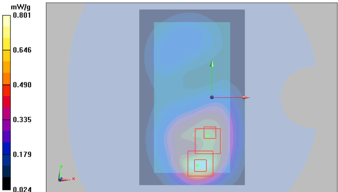
Figure 45 Body, Back Side, WCDMA Band II Channel 9400
