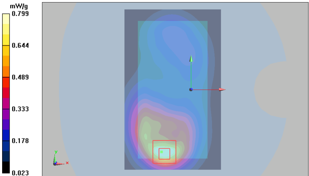
Figure 68 Body with Earphone, Front Side, WCDMA Band IV Channel 1513
