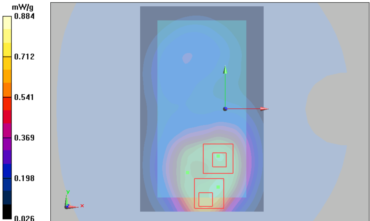
Figure 58 Body, Back Side, WCDMA Band IV Channel 1413
