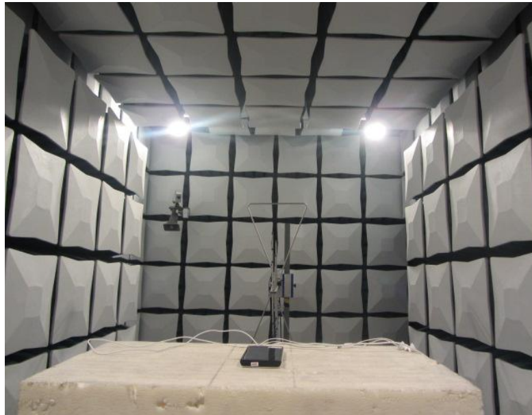
Field Strength of Spurious Emissions (below 3GHz)
