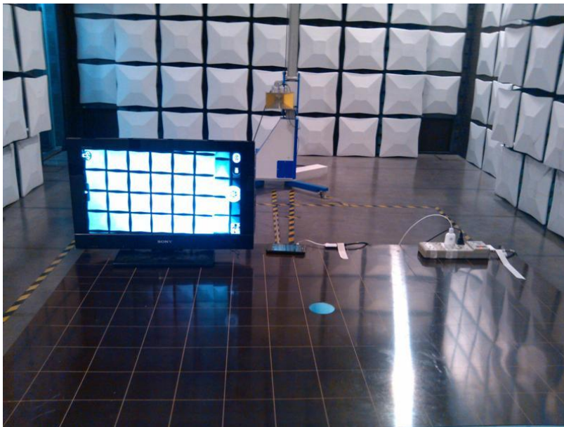
Radiated Emissions (1GHz to18GHz)
