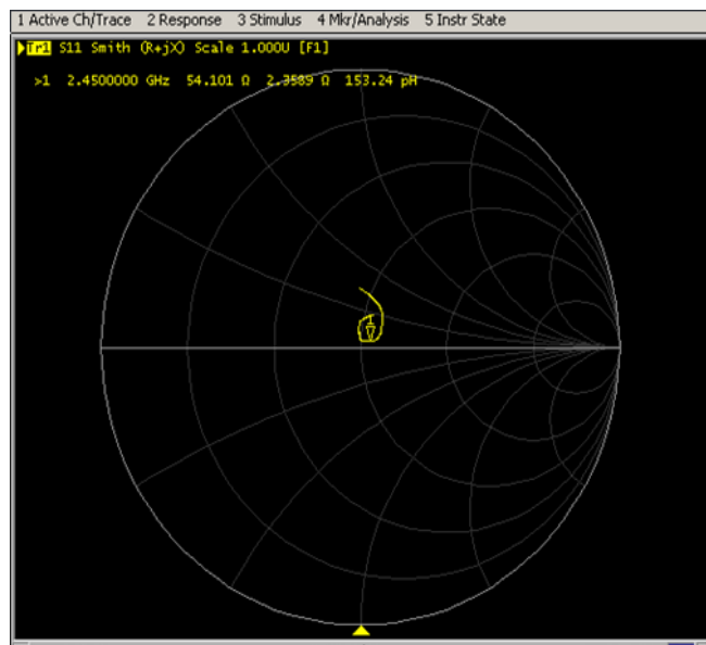
Impedance Test-Body
