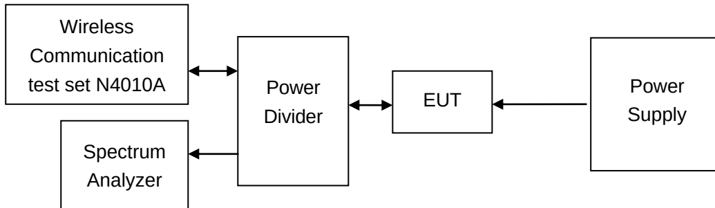
Figure 6. Test Set-up
